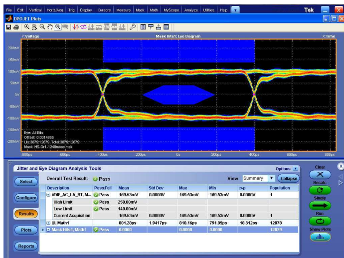
MIPI® M-PHY Debug, Analysis, Characterization and Conformance Test Solution (Option M-PHY) – Verify to the M-PHY specification by rapidly characterizing and discovering sources of jitter and signal integrity concerns. Using DPOJET, Option M-PHY enables transmitter signaling and timing measurements such as differential transmit eye diagrams, rise and fall times, slew rate, amplitude parameters, common mode voltages on each lane for both the large and small amplitude configurations, as well as the terminated and unterminated cases.
