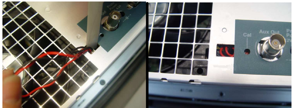
Figure 4-2: Reconnecting the fan cable
