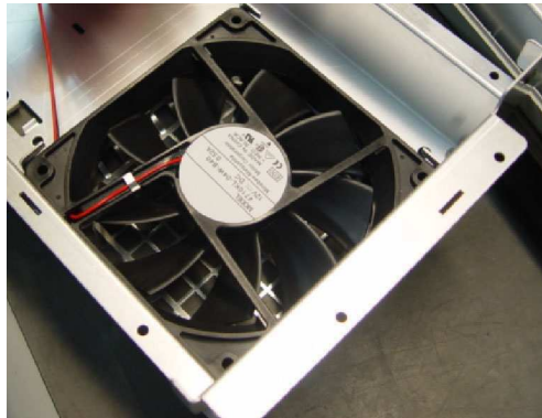
Figure 4-3: Fan cable dress
