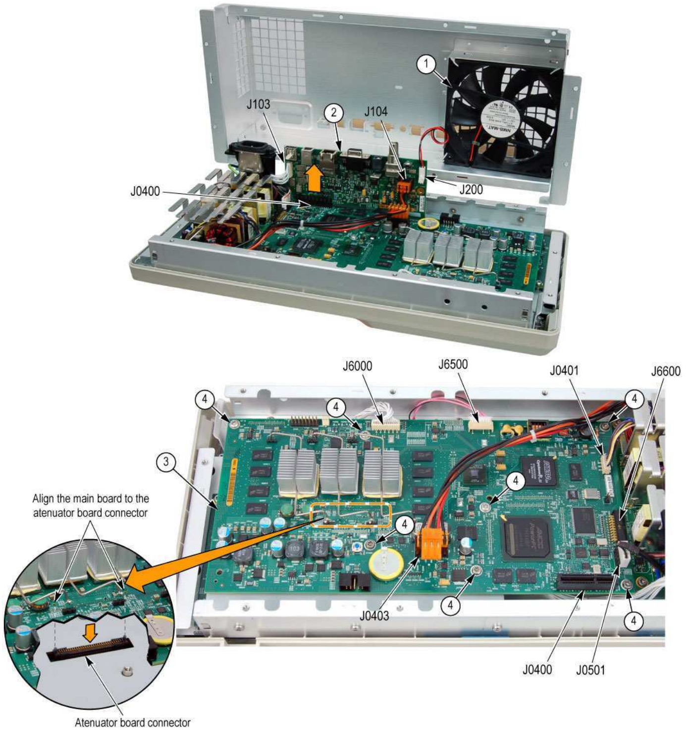
Figure 5-2: Exploded view: DPO3000 I/O and main boards
