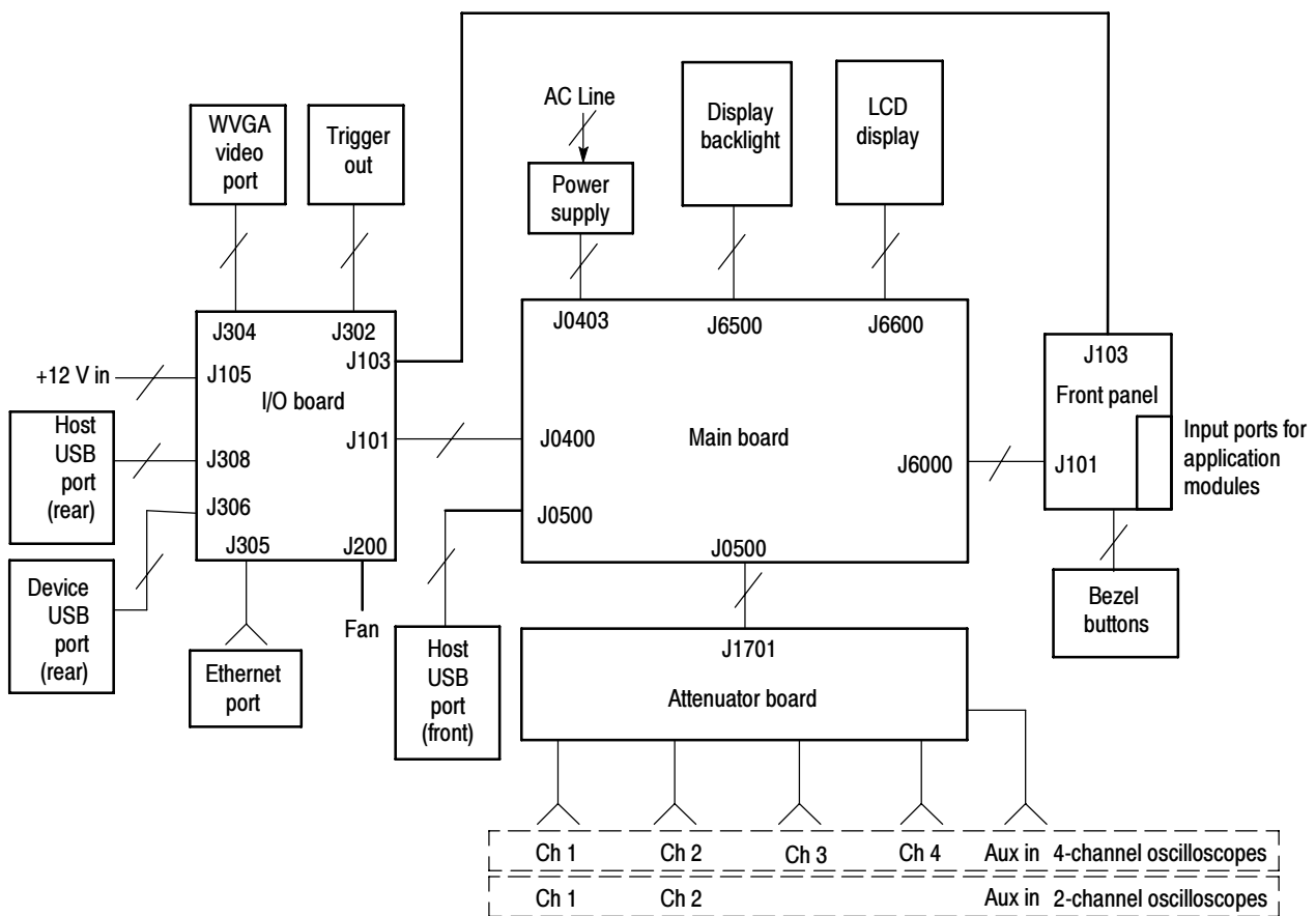
Figure 2-1: Oscilloscope module interconnections
