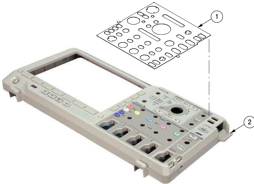
Figure 5-4: Exploded view: DPO3000 front panel labels
