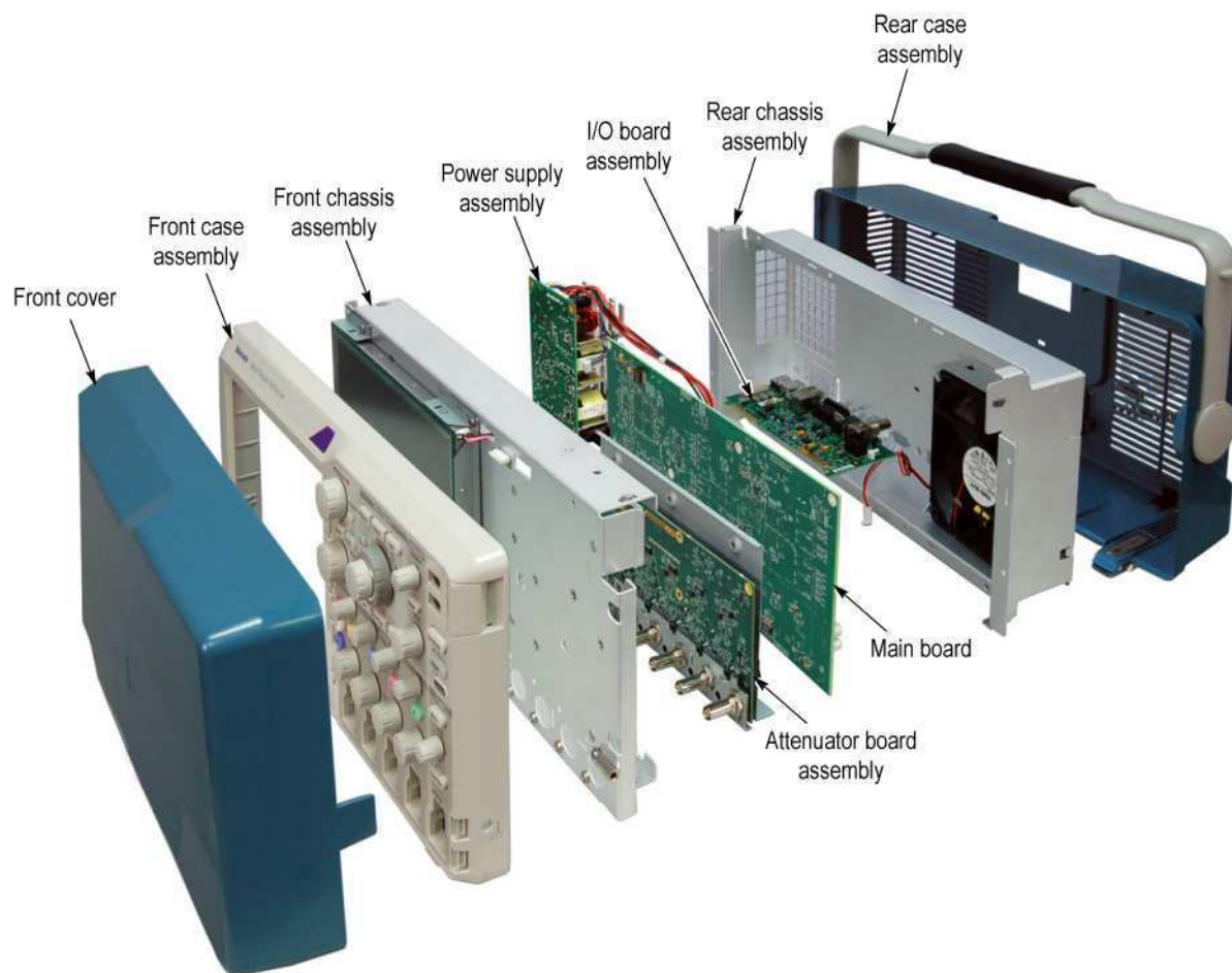
Figure 4-1: Locator for internal modules
