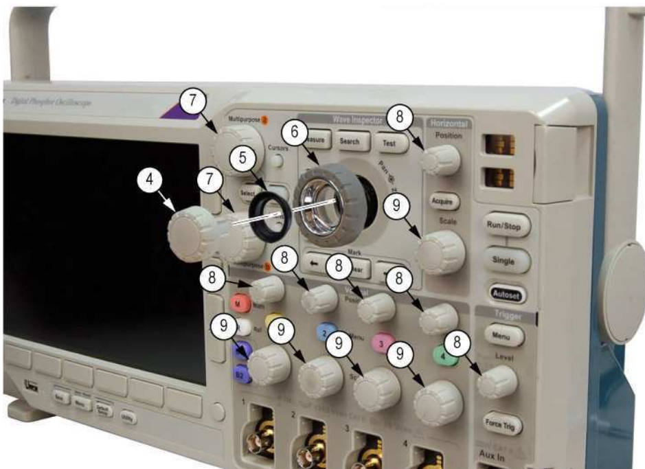
Figure 5-3: Exploded view: DPO3000 front panel and power supply
