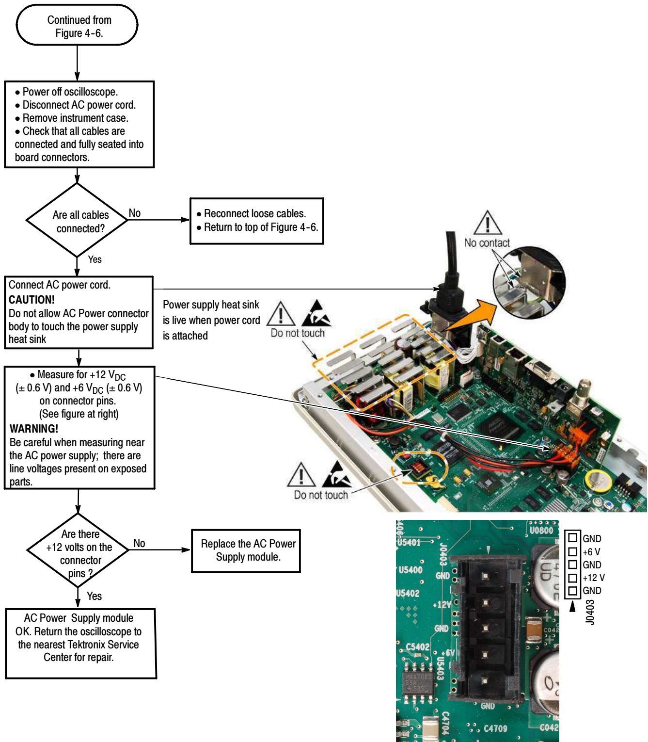
Figure 4-7: AC power supply troubleshooting procedure
