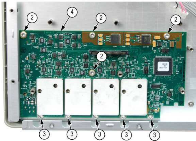
Figure 5-5: Exploded view: Main board shield and attenuator board
