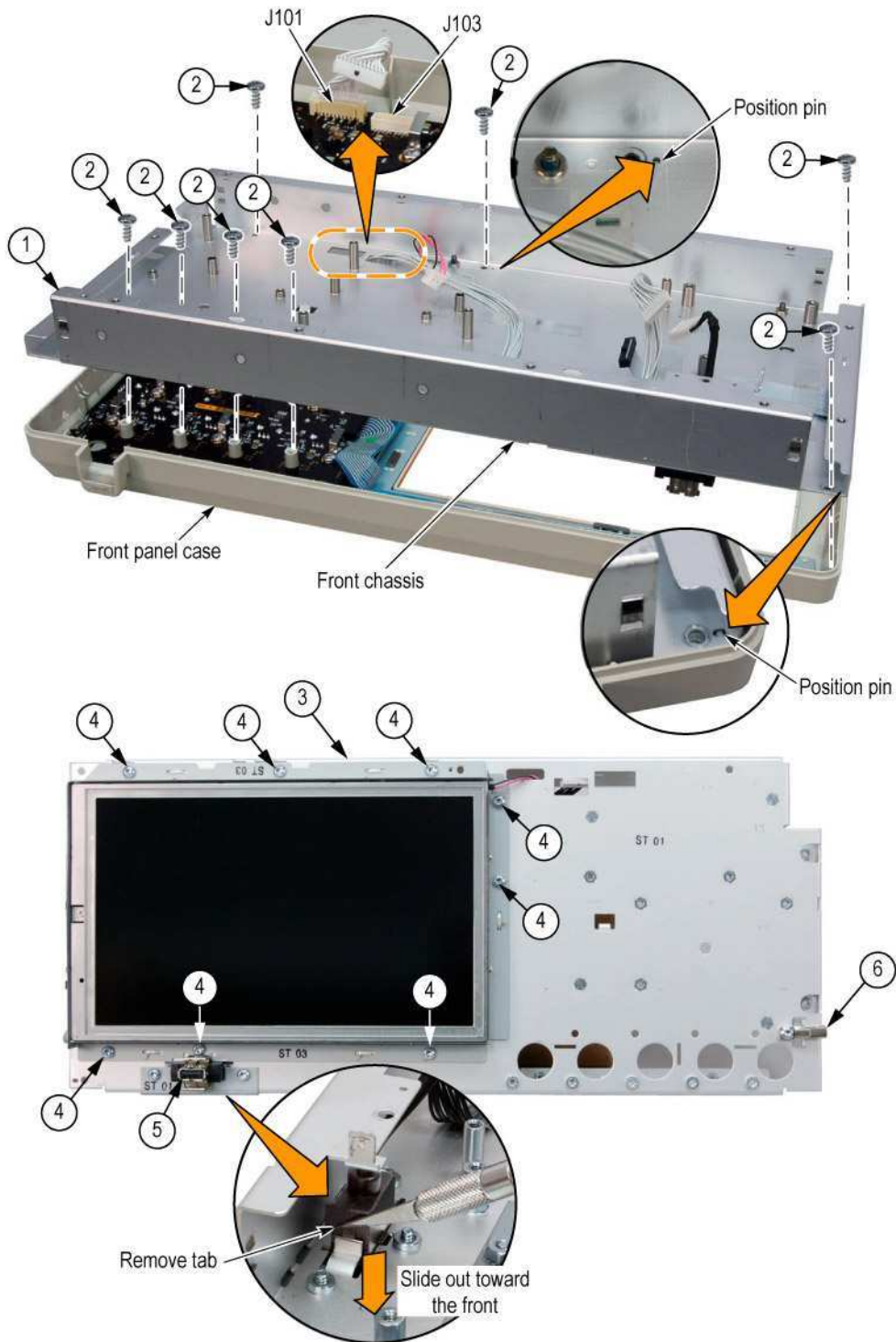
Figure 5-6: Exploded view: DPO3000 front chassis and LCD assembly
