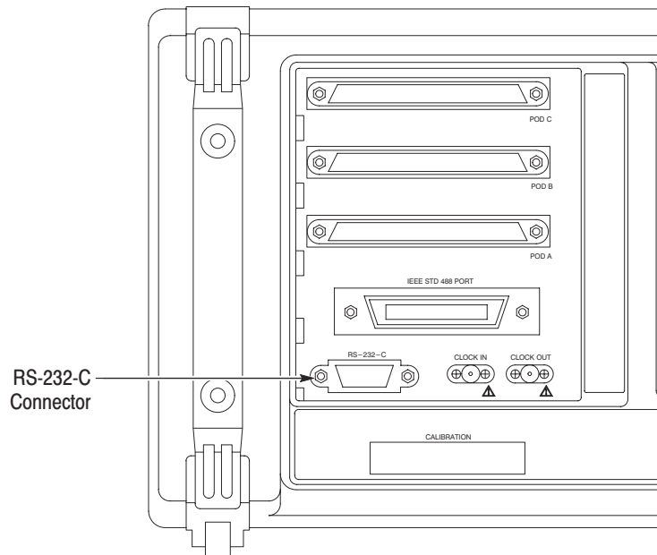
Figure 1-6: RS-232-C port
