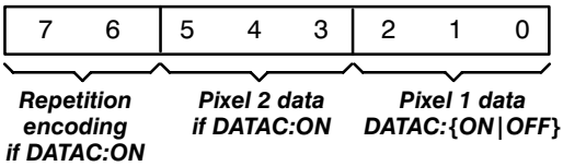
Figure 2-3: Bits in a Pixel Block Data Byte
