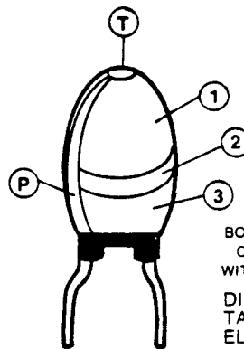
METAL-FILM RESISTORS
