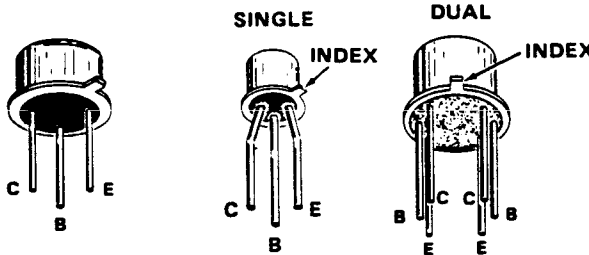
METAL-CASED TRANSISTORS
