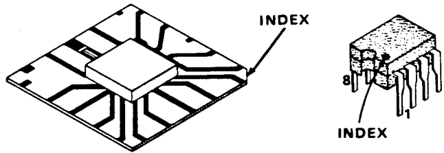
INTEGRATED CIRCUITS
