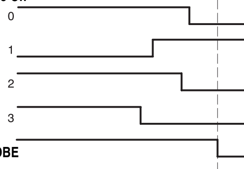
Figure 3-30: Event signal timing and strobe
