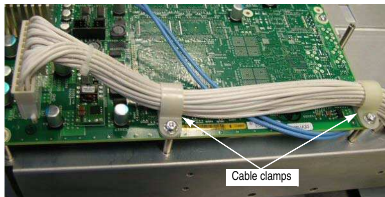
Figure 4-16: Location of the cable clamps on the AWG1G board
