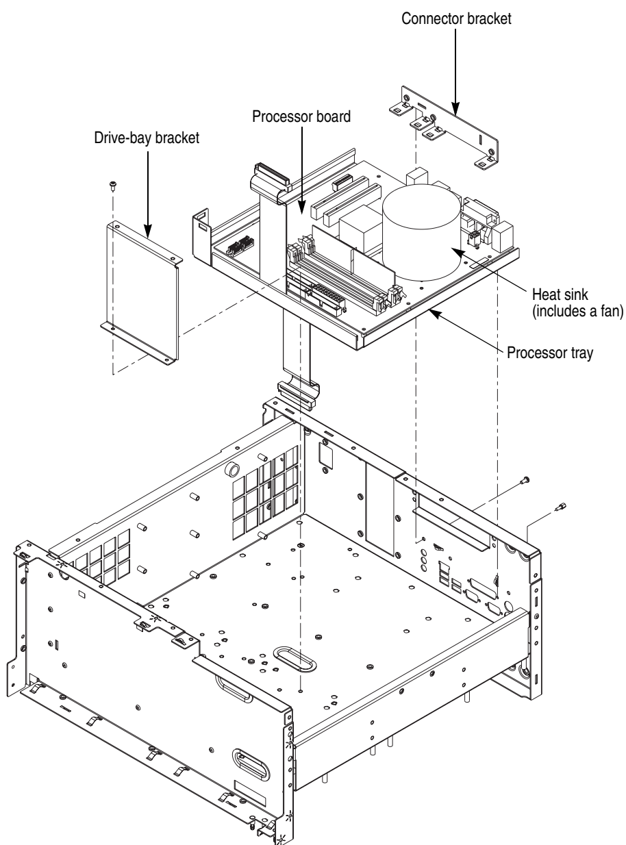
Figure 4-11: Processor board removal
