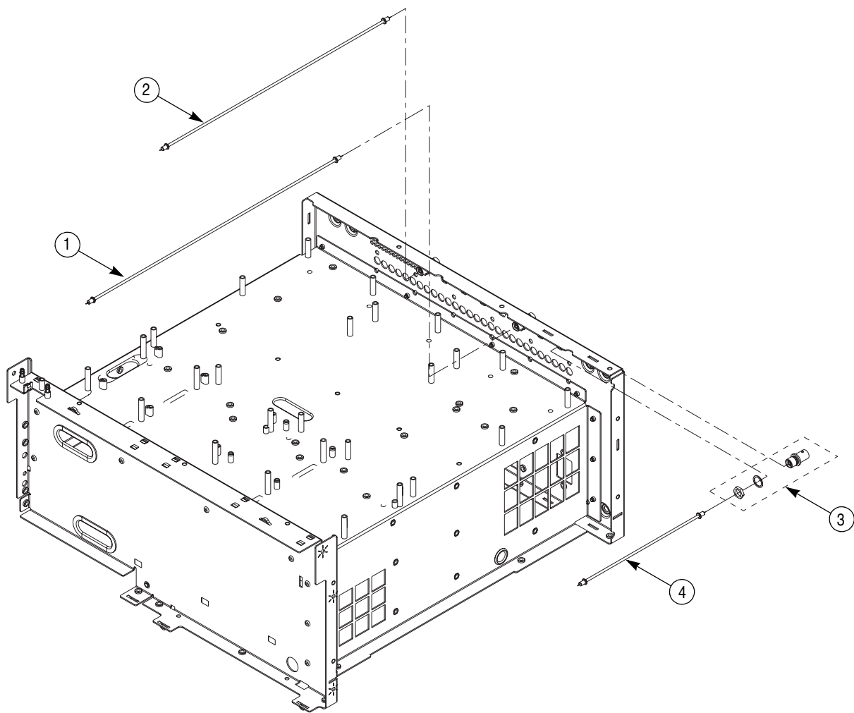
Figure 5-15: Exploded diagram - Rear connectors
