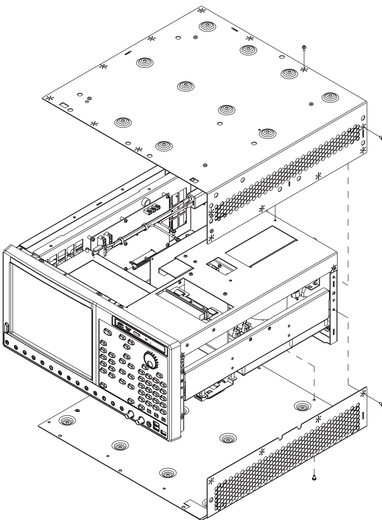
Figure 4-4: EMI covers removal
