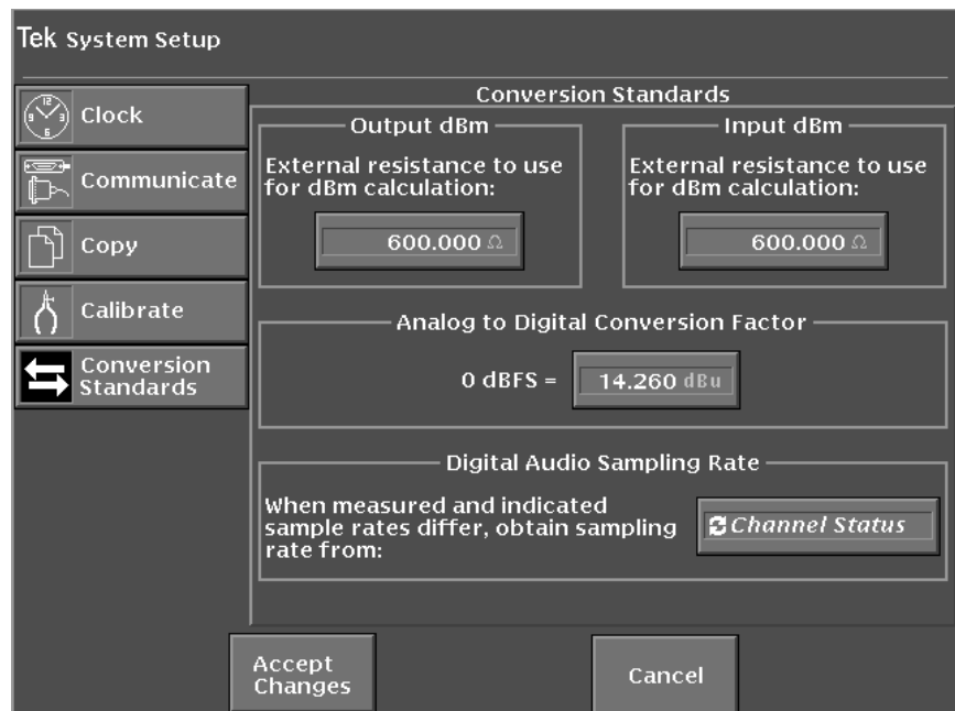
Figure 3-13: System Setup Conversion Standards menu
