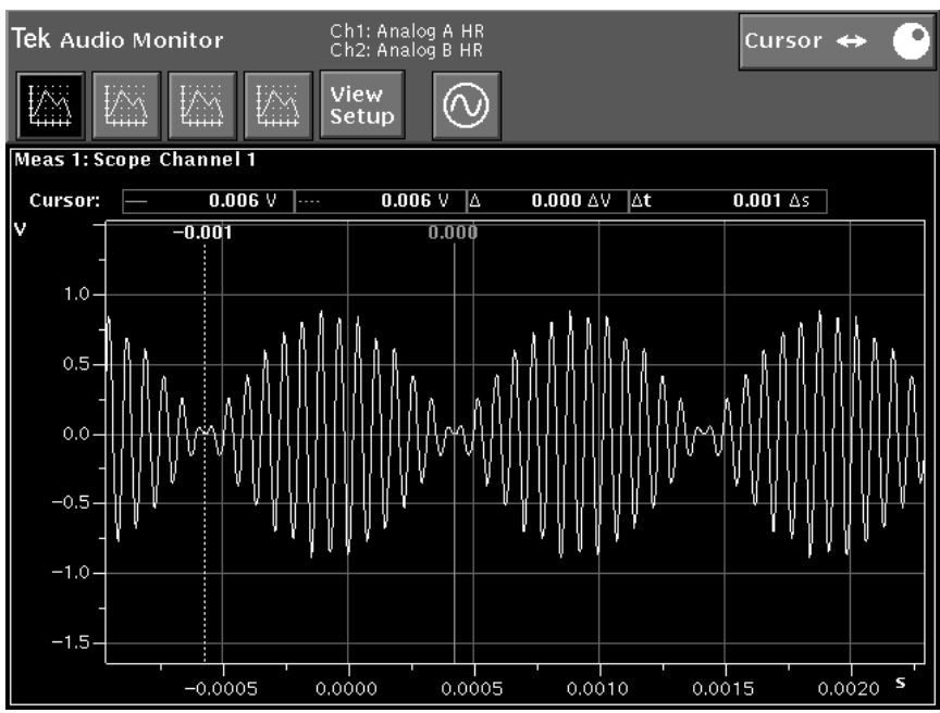
Figure 4-52: Use of Cursors to measure pulse time
