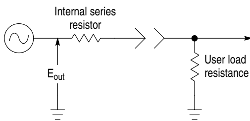
Figure 3-14: AM700 generator output voltage divider for dBm calculations
