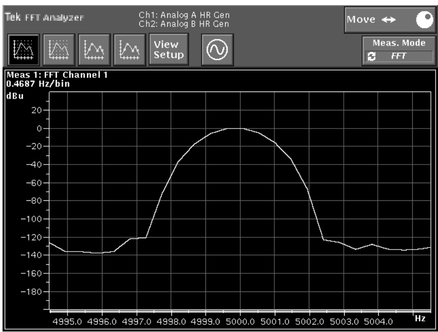
Figure 4-41: Zoomed FFT display showing maximum expansion of the trace
