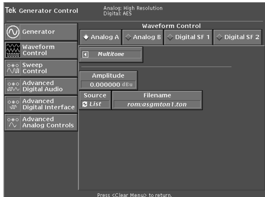
Figure 4-42: Generator Waveform Control setup for multitone detection
