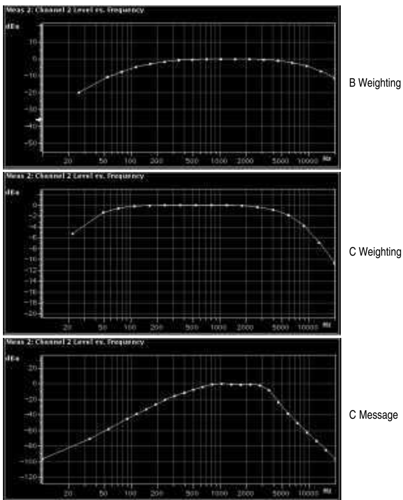
Figure 4-34: Filter Curves: B Weighting, C Weighting, and C Message
