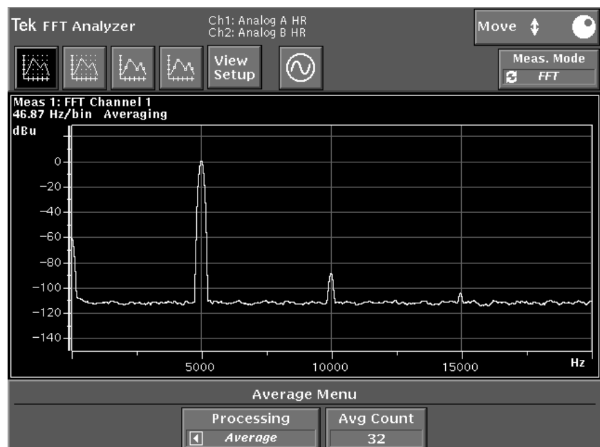
Figure 2-9: Average menu and FFT trace with averaging applied
