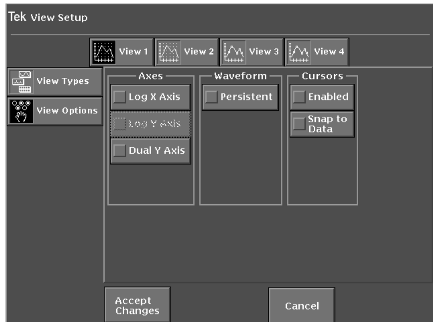
Figure 3-7: FFT Analyzer View Options in the View Setup controls
