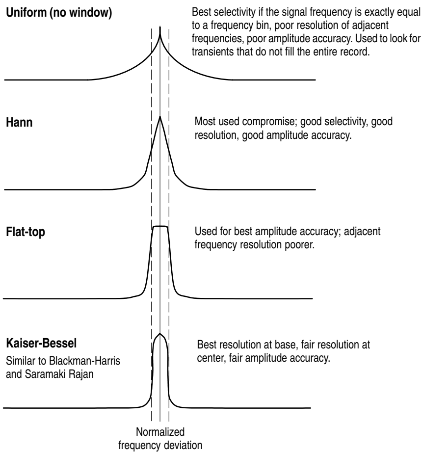
Figure 4-38: Effects of Window selections
