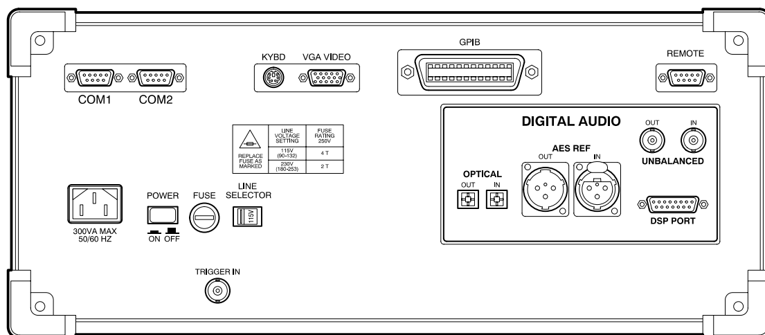
Figure 2-25: AM700 rear panel
