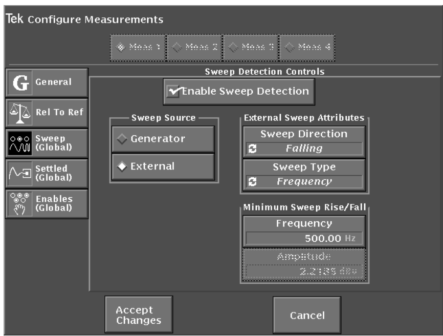
Figure 4-25: Sweep detection controls
