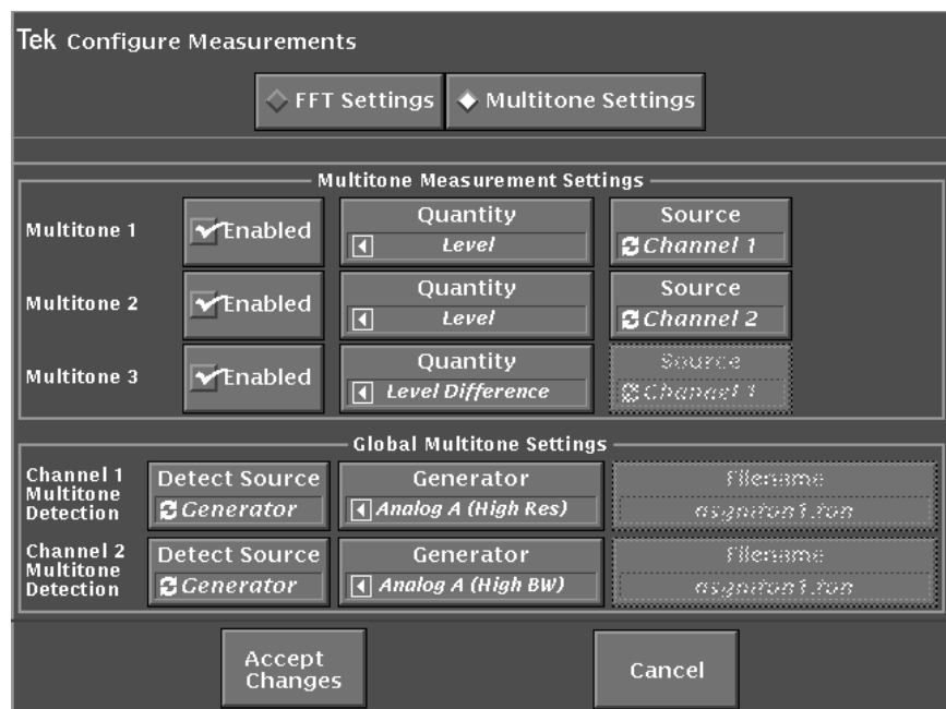
Figure 4-43: Multitone measurement settings in the Configure Measurements menu
