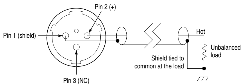
Figure 2-23: Driving an unbalanced load with the AM700 generator
