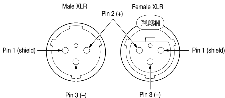
Figure 2-22: Analog XLR connector pin outs
