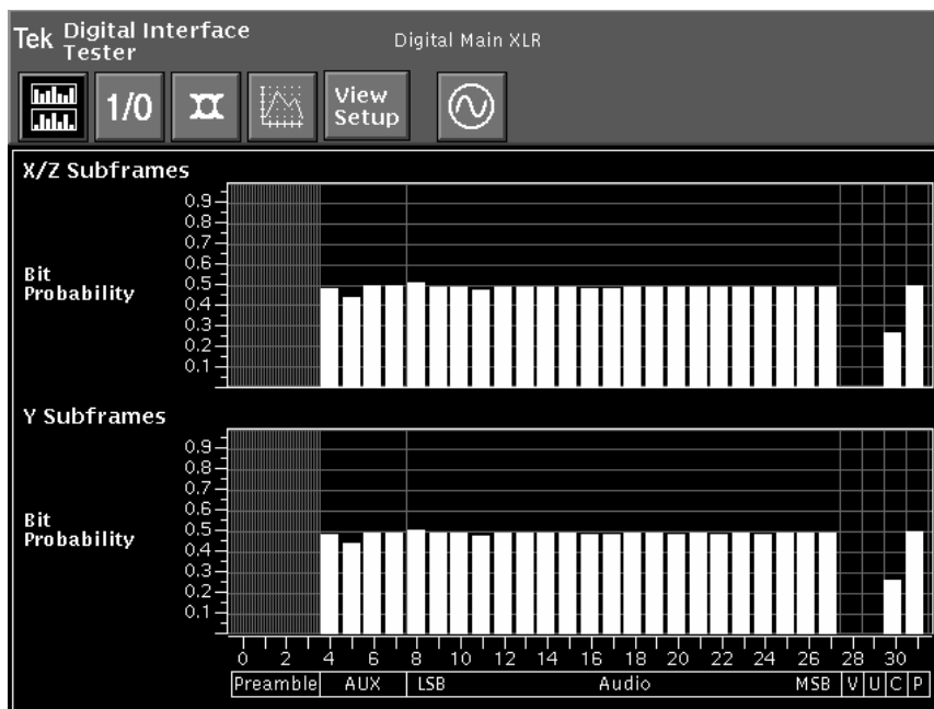
Figure 4-59: Bit Probability display with 24-bit digital data
