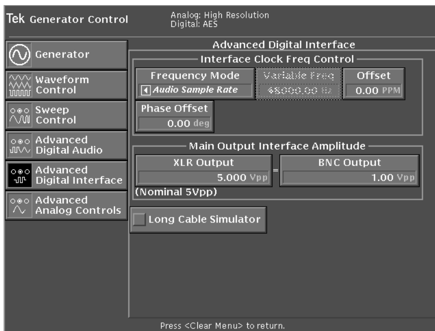
Figure 4-11: Advanced Digital Interface display
