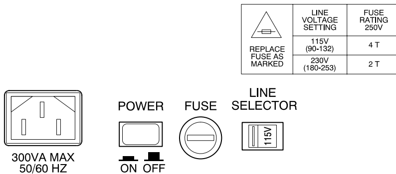
Figure 2-26: Mains connector, power switch, fuse, and line selector
