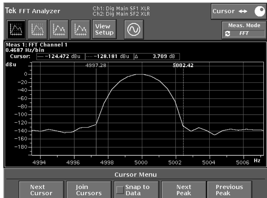
Figure 2-8: Cursor menu showing frequency and level readouts
