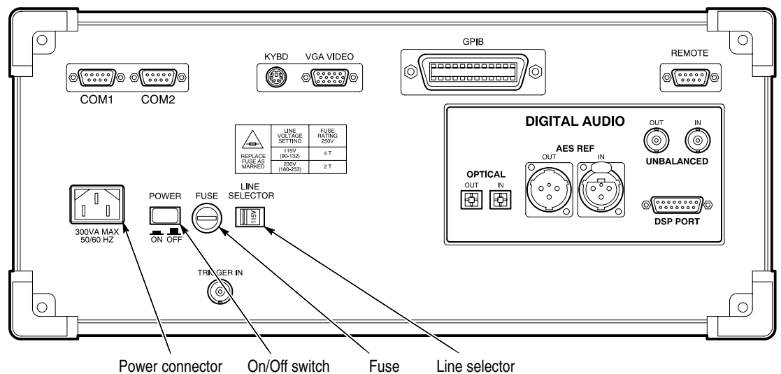
Figure 1-1: Rear panel fuse, power connector, On/Off Switch, and line selector
