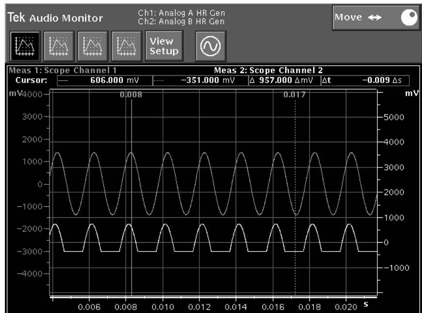
Figure 4-48: Audio Monitor display with dual Y-axis display
