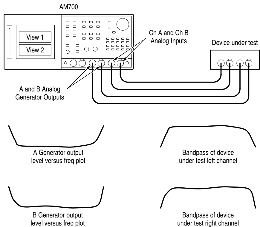
Figure 4-19: Regulation mode bandpass measurement of level versus frequency
