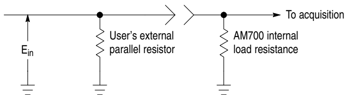
Figure 3-15: AM700 input circuit for dBm calculation
