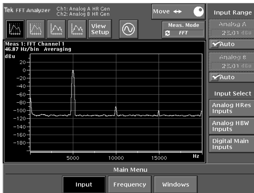
Figure 4-40: FFT Input Select and Input Range menus
