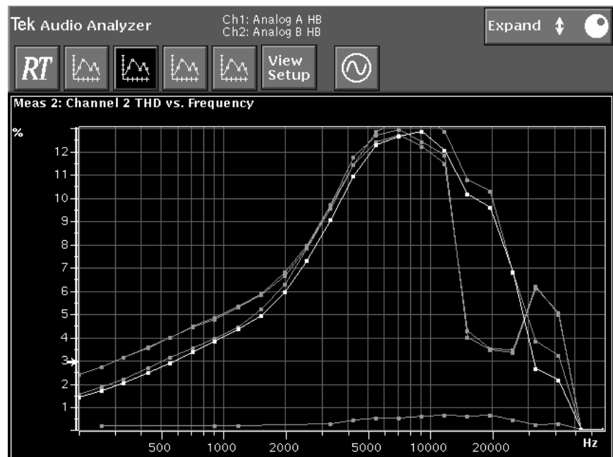
Figure 4-20: History display of Channel 2 THD versus frequency obtained using closed-loop operation
