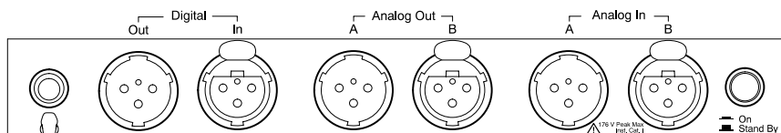
Figure 2-21: Front-panel signal connectors
