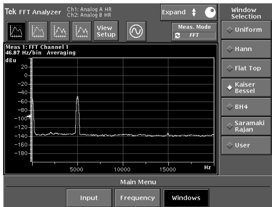
Figure 4-37: FFT Analyzer Window menu display
