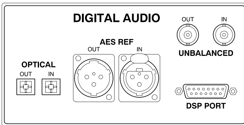
Figure 2-32: Digital audio connectors
