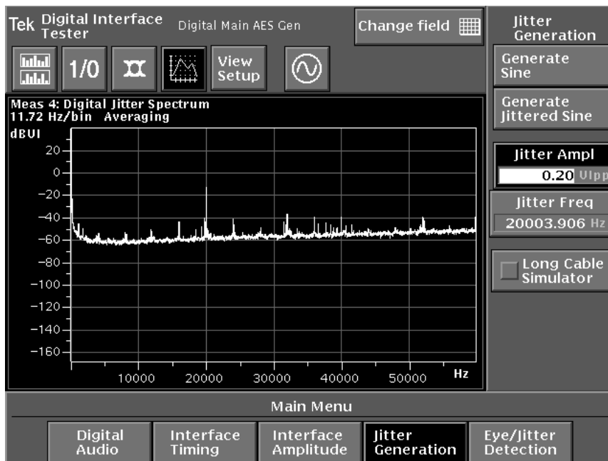
Figure 4-68: Digital Interface Tester Main Menu with Jitter Spectrum submenus
