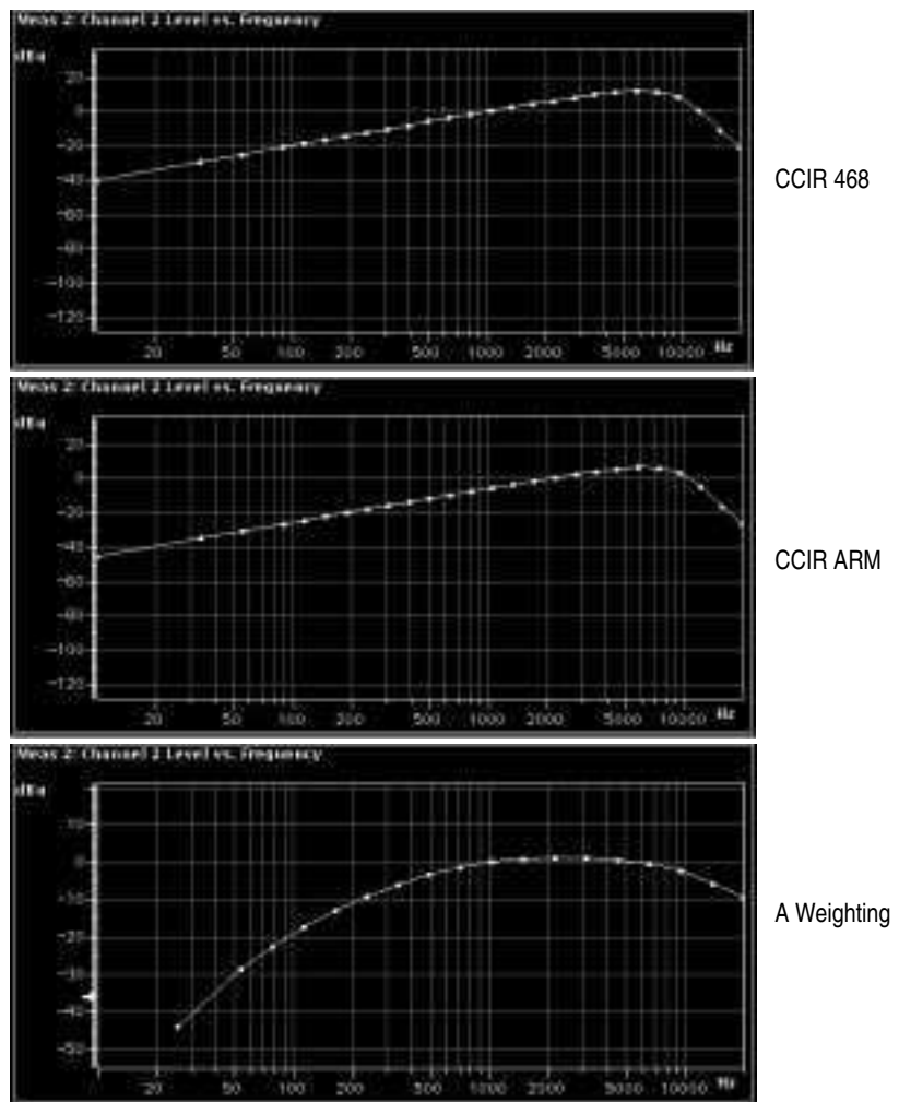
Figure 4-33: Filter curves: CCIR 468, CCIR ARM, and A Weighting
