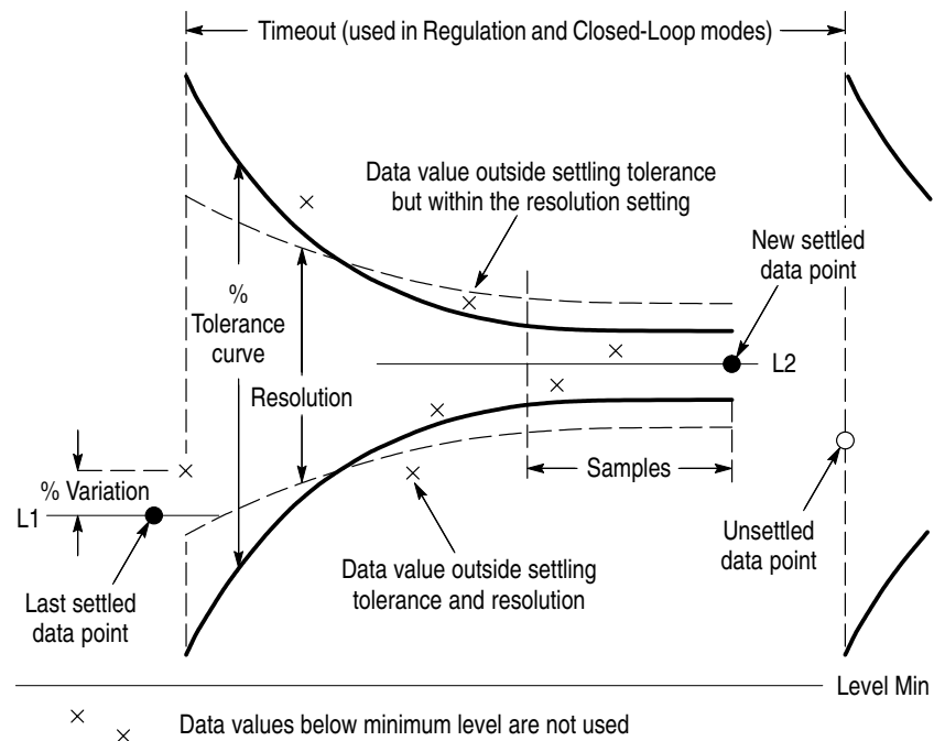
Figure 4-28: Exponential settling in Audio Analyzer
