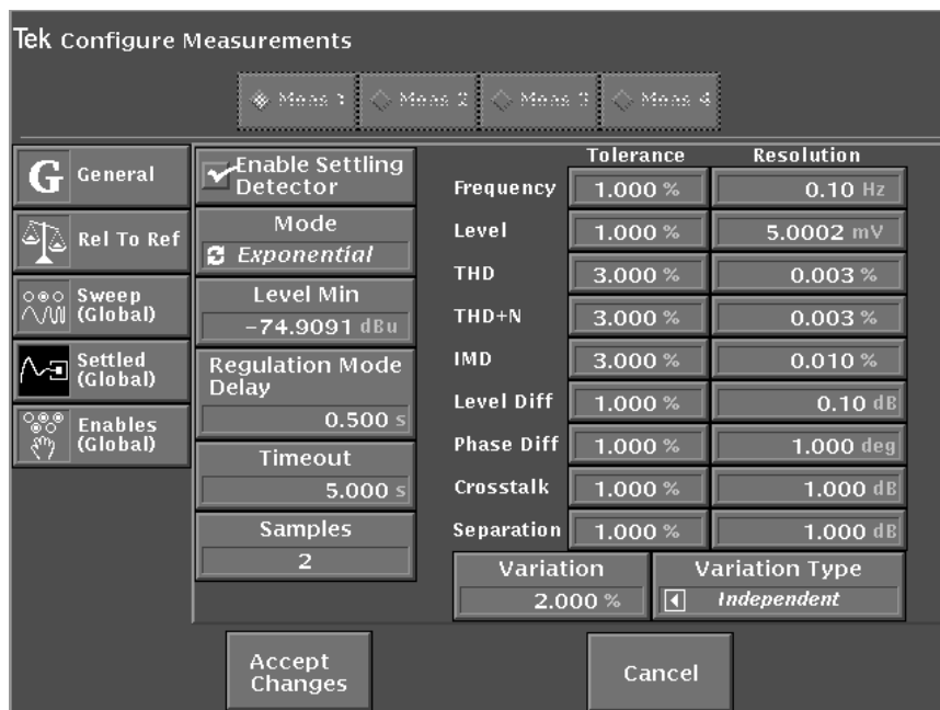
Figure 4-27: Settled data point detection controls display
