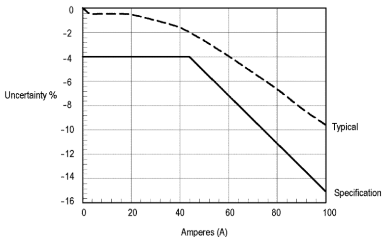
Figure 8: DC signal linearity in the 10 mV/A range, typical
