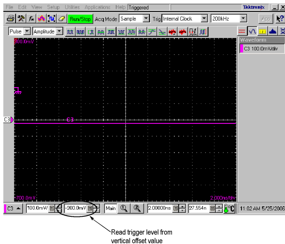
Figure 12: Trigger offset indicator
