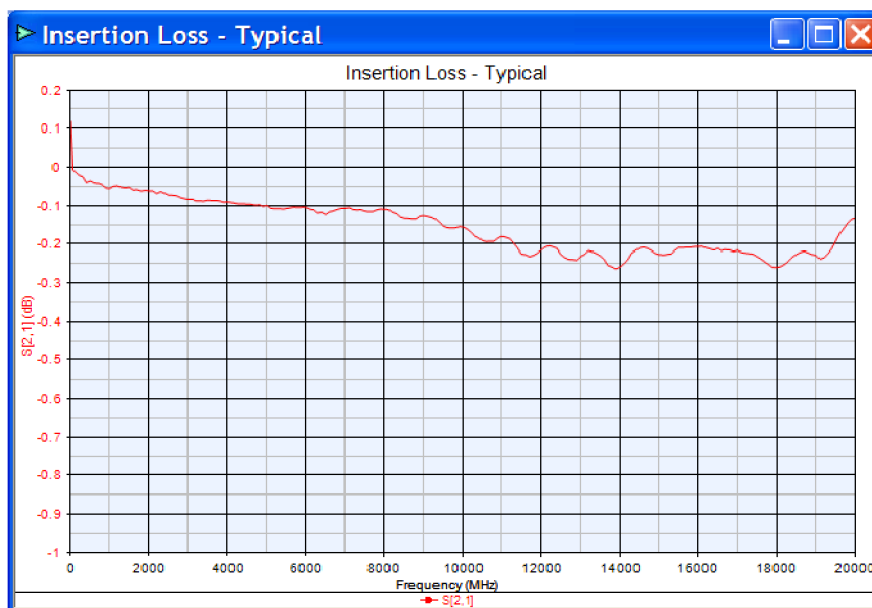
Figure 14: Insertion loss
