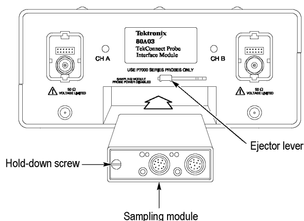
Figure 4: Installing the sampling module into the TekConnect Probe Interface Module
