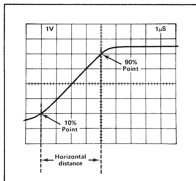
Fig. 1-14. Measuring risetime.
