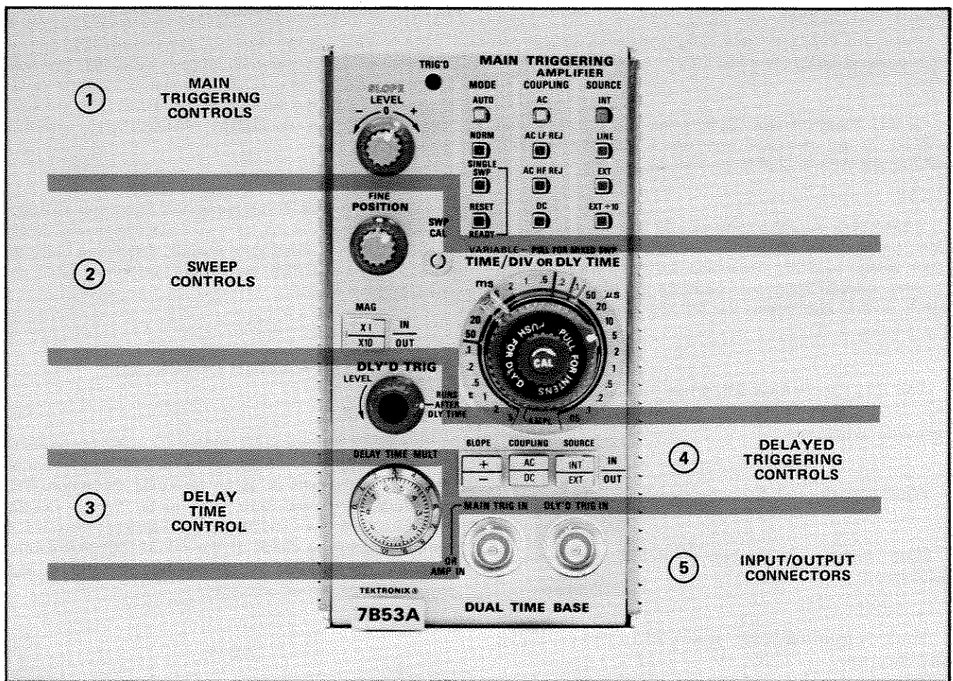
Fig. 1-4. Front-panel controls and connectors.
