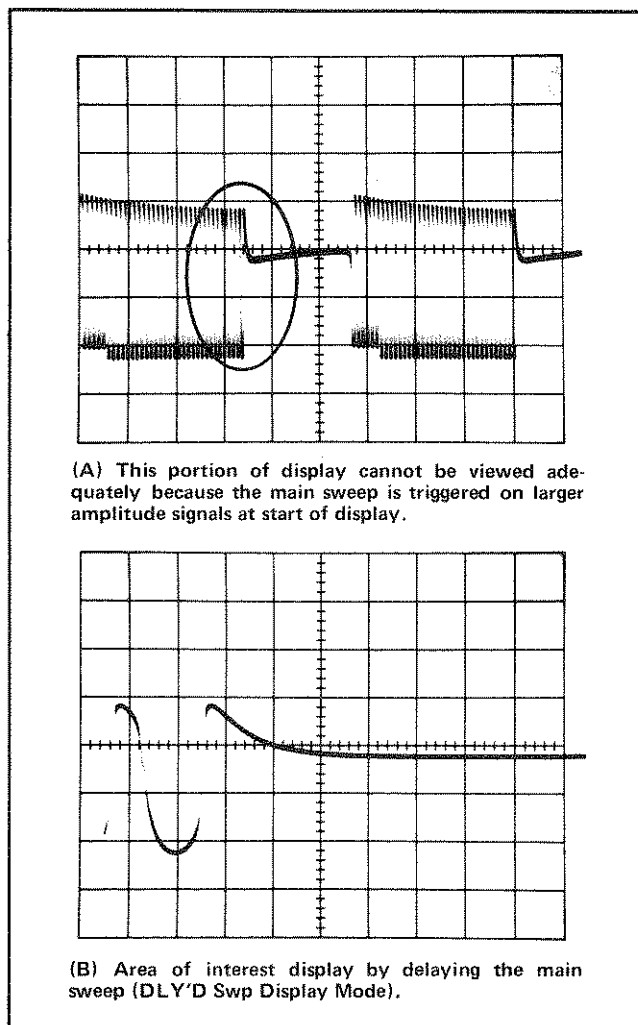
Fig. 1-17. Displaying a complex signal using delayed sweep.
