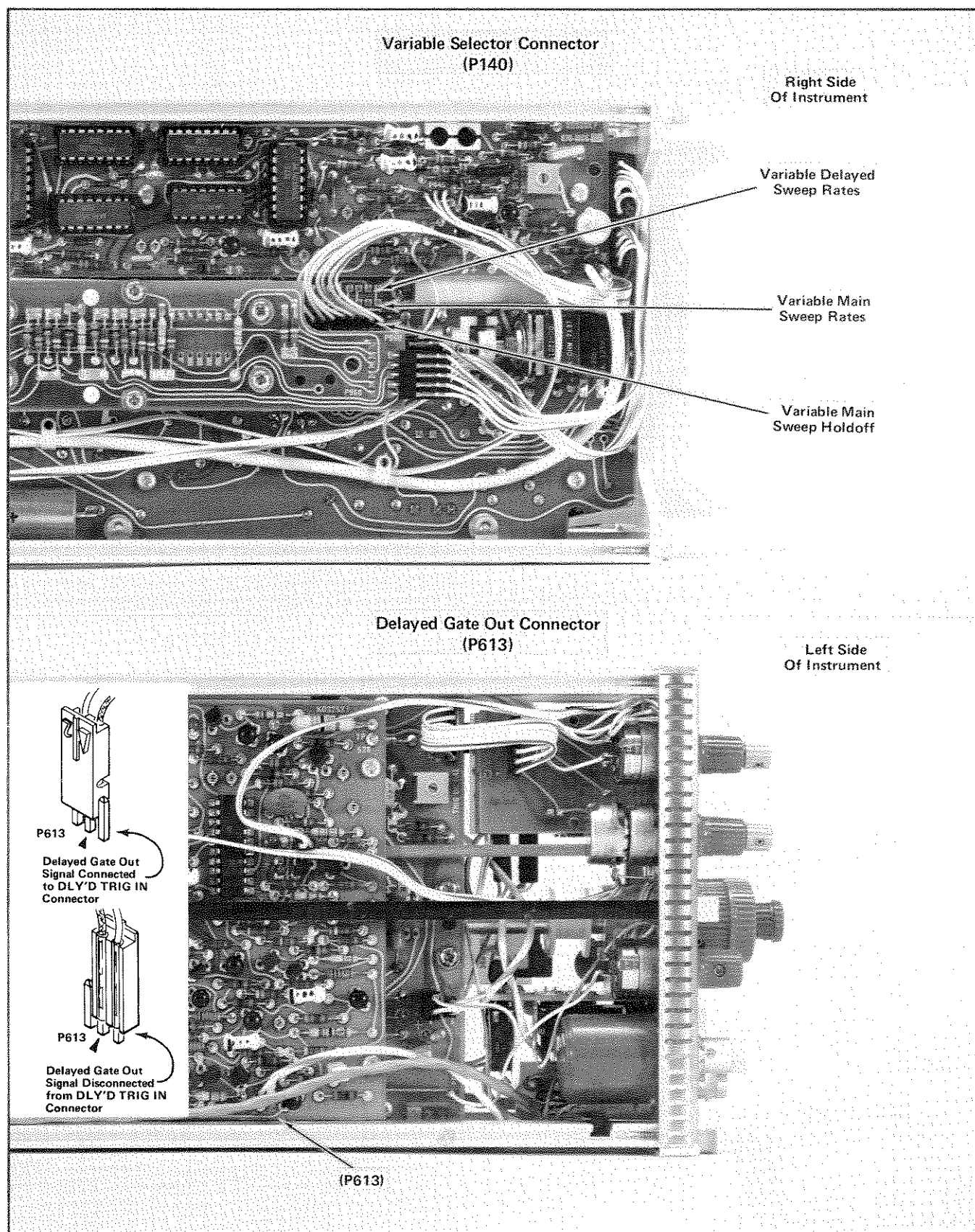
Fig. 1-3. Location of Delayed Gate Out and Variable Selector multi-pin connectors.
