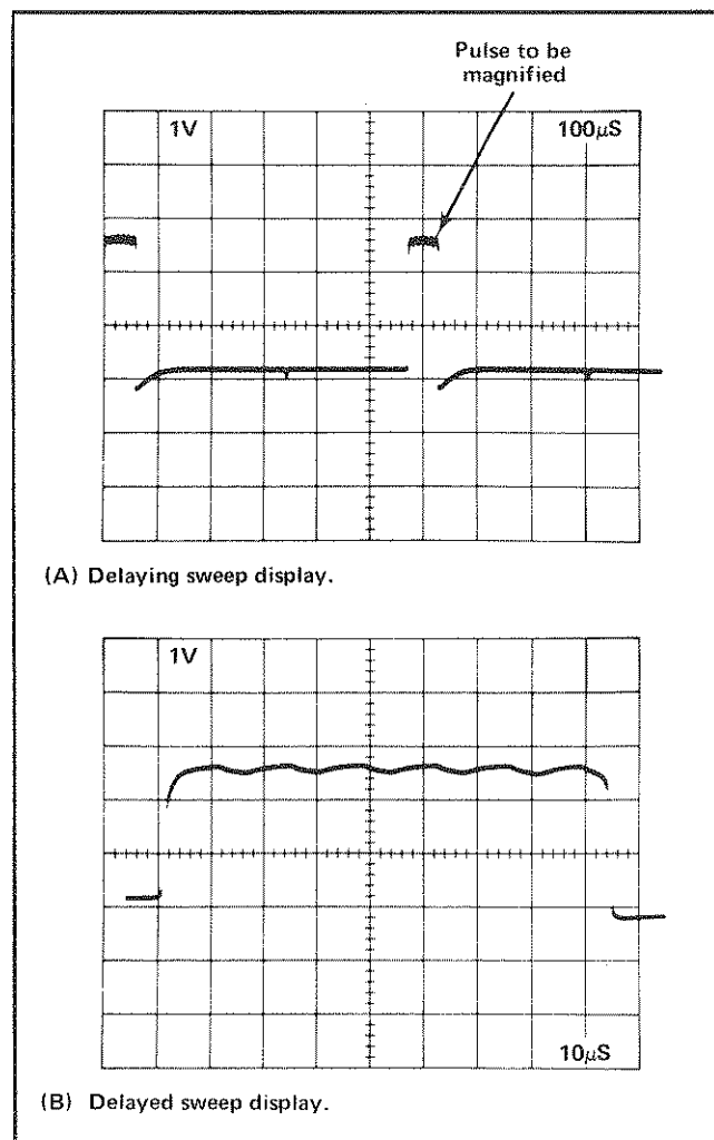
Fig. 1-16. Using delayed sweep for magnification.
