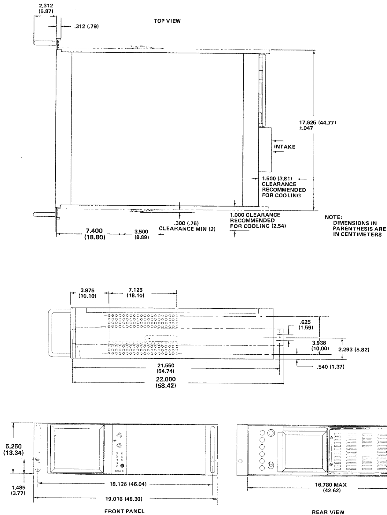
Fig. 3-6. Dimensional drawing.
