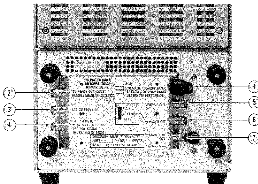
Rear Panel
