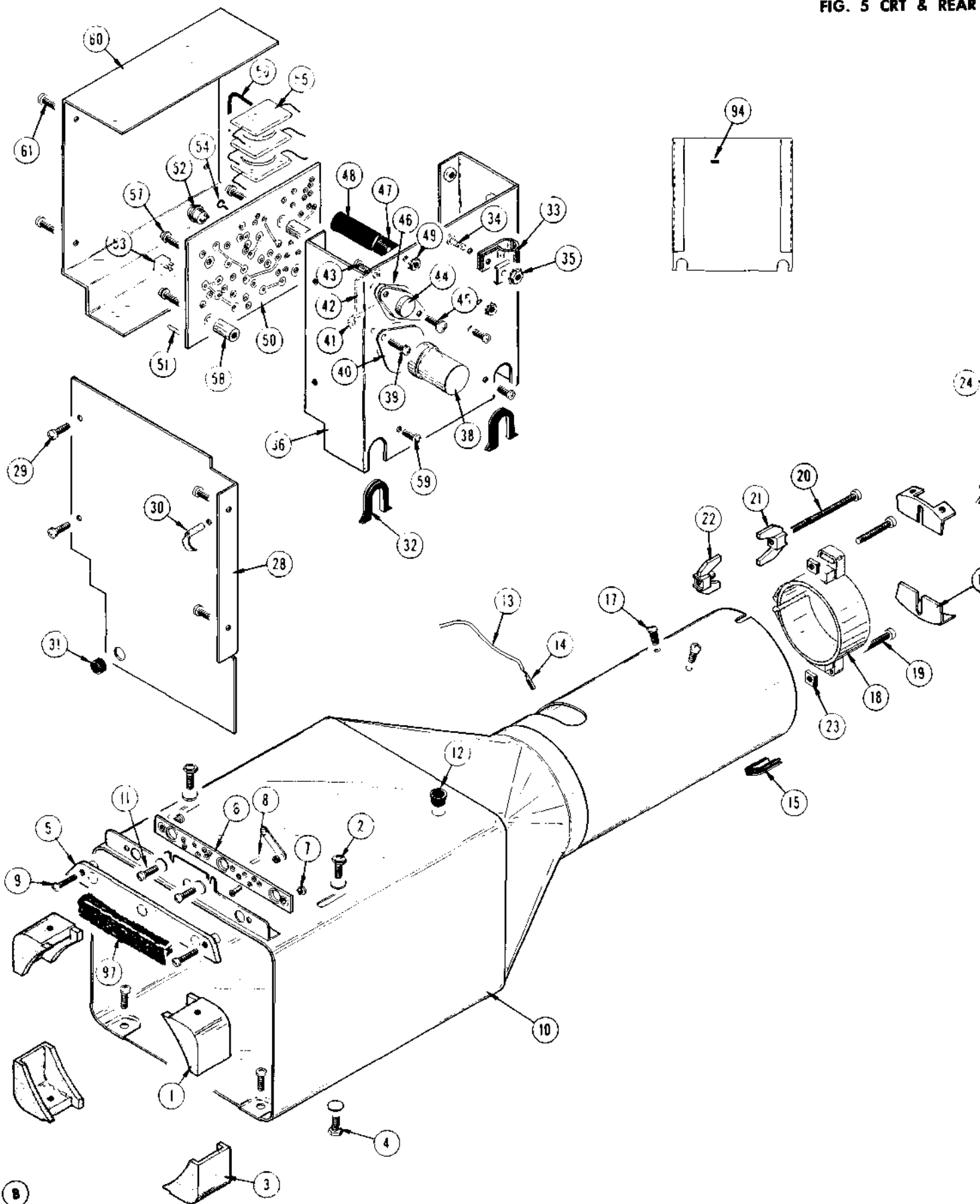
FIG. 5 CRT & REAR
