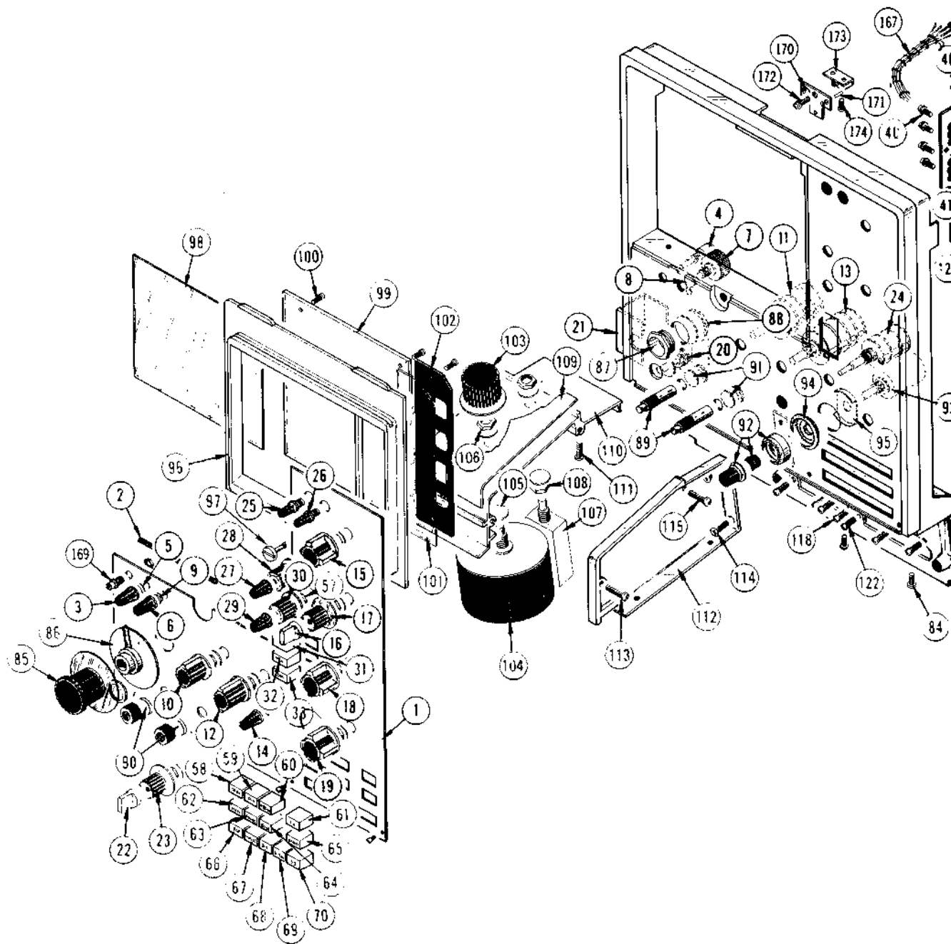
FIG. 1 FRONT
