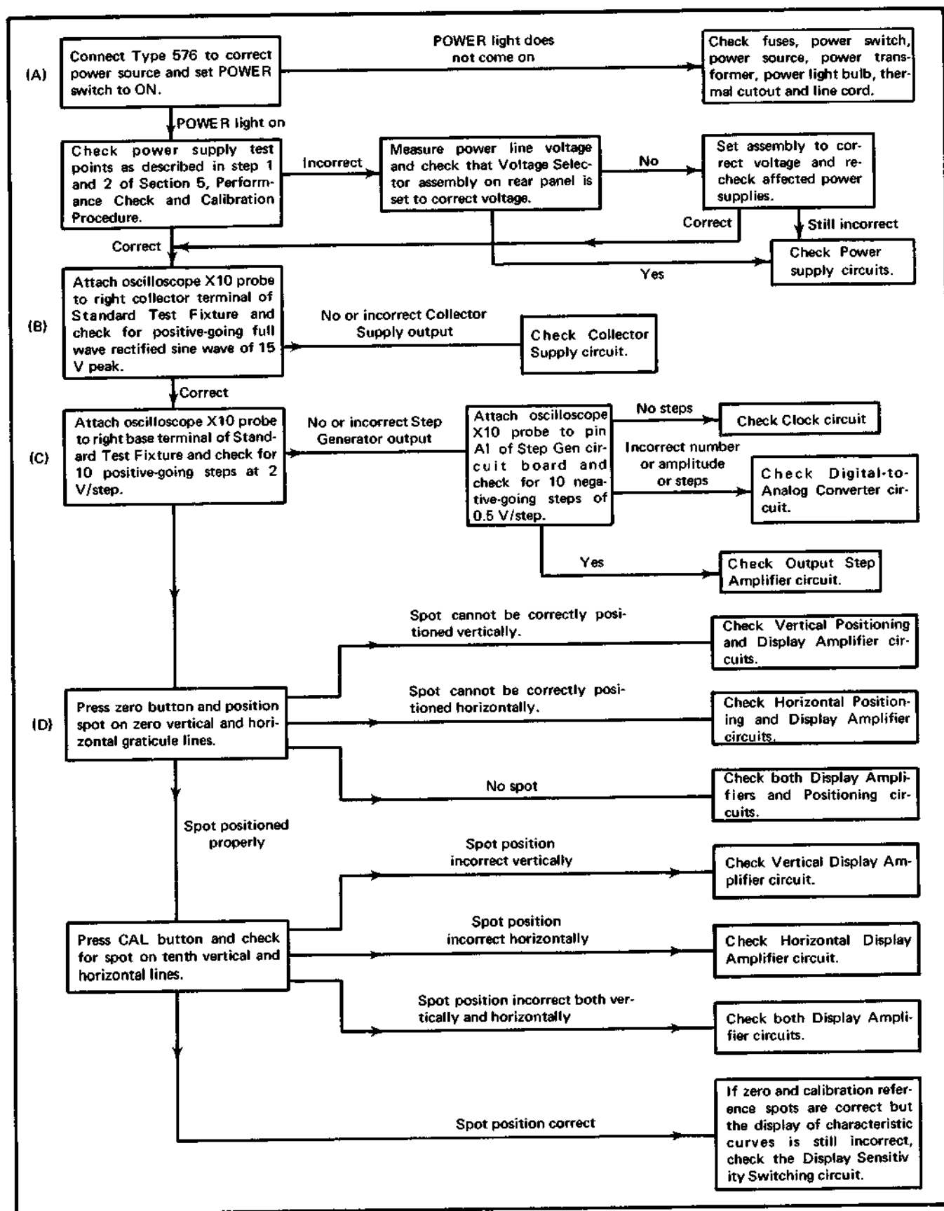
Fig. 4-3. Troubleshooting chart.
