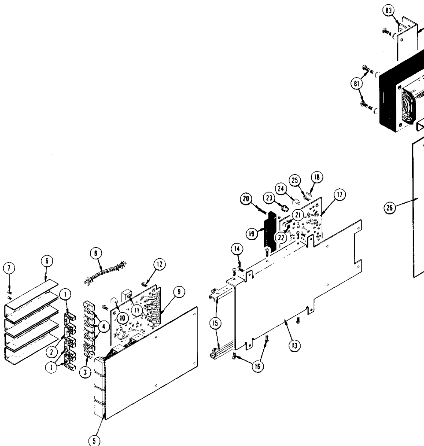
FIG. 3 CHASSIS
