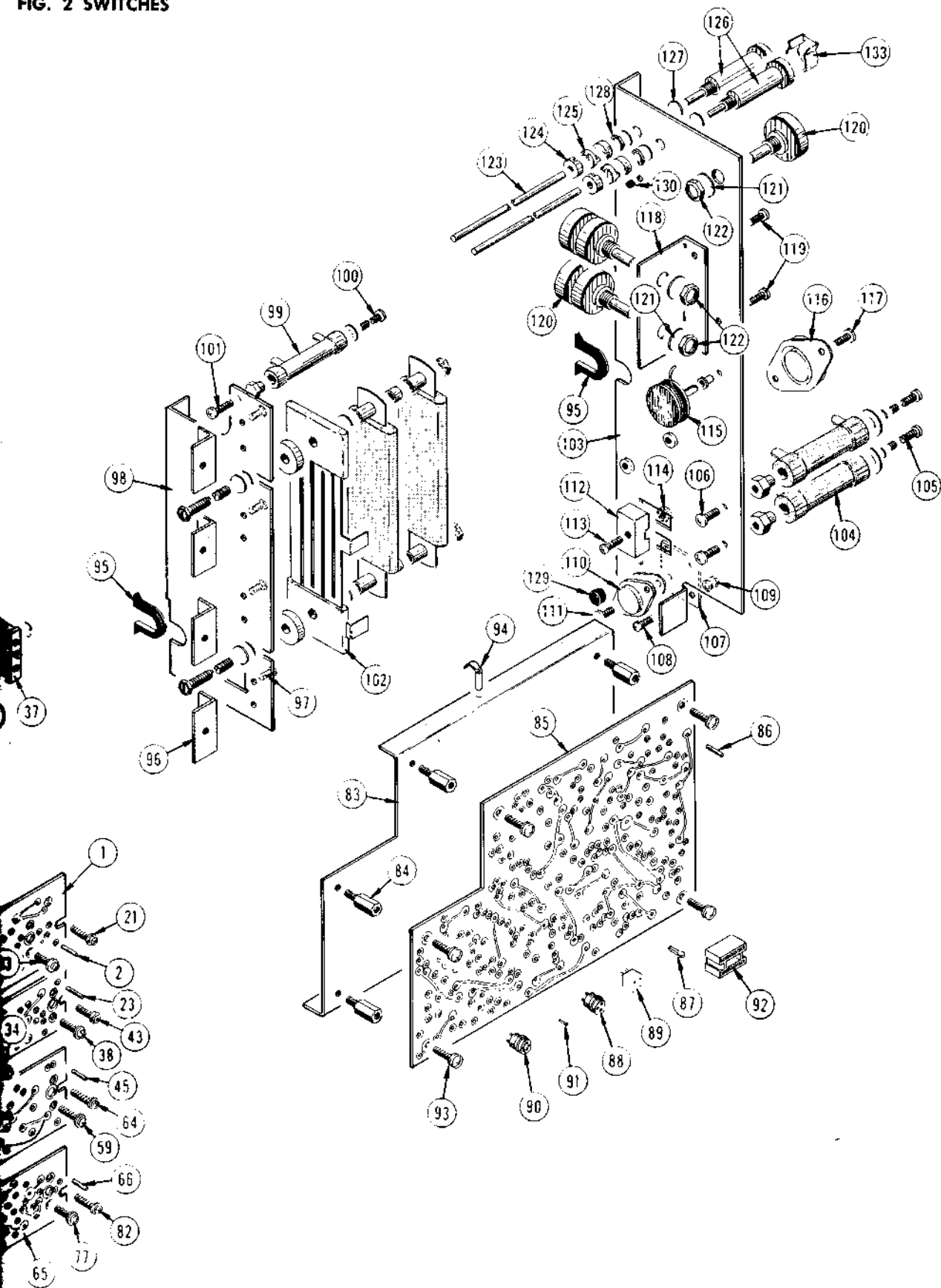
FIG. 2 SWITCHES
