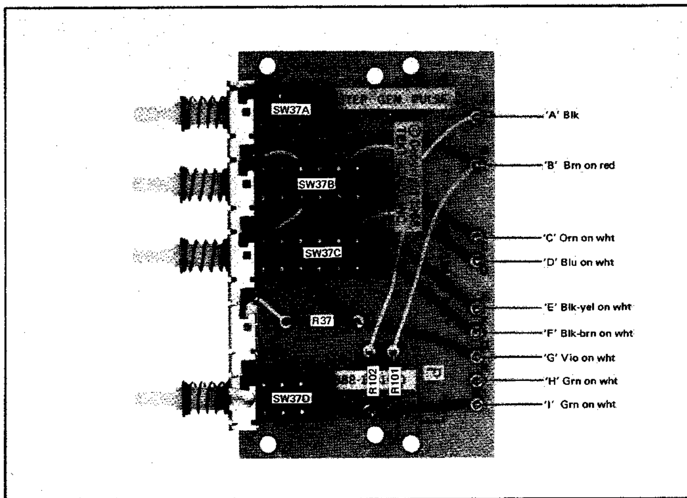
Fig. 4-10. Component locations and wiring color codes on Step Gen Pulse circuit board.
