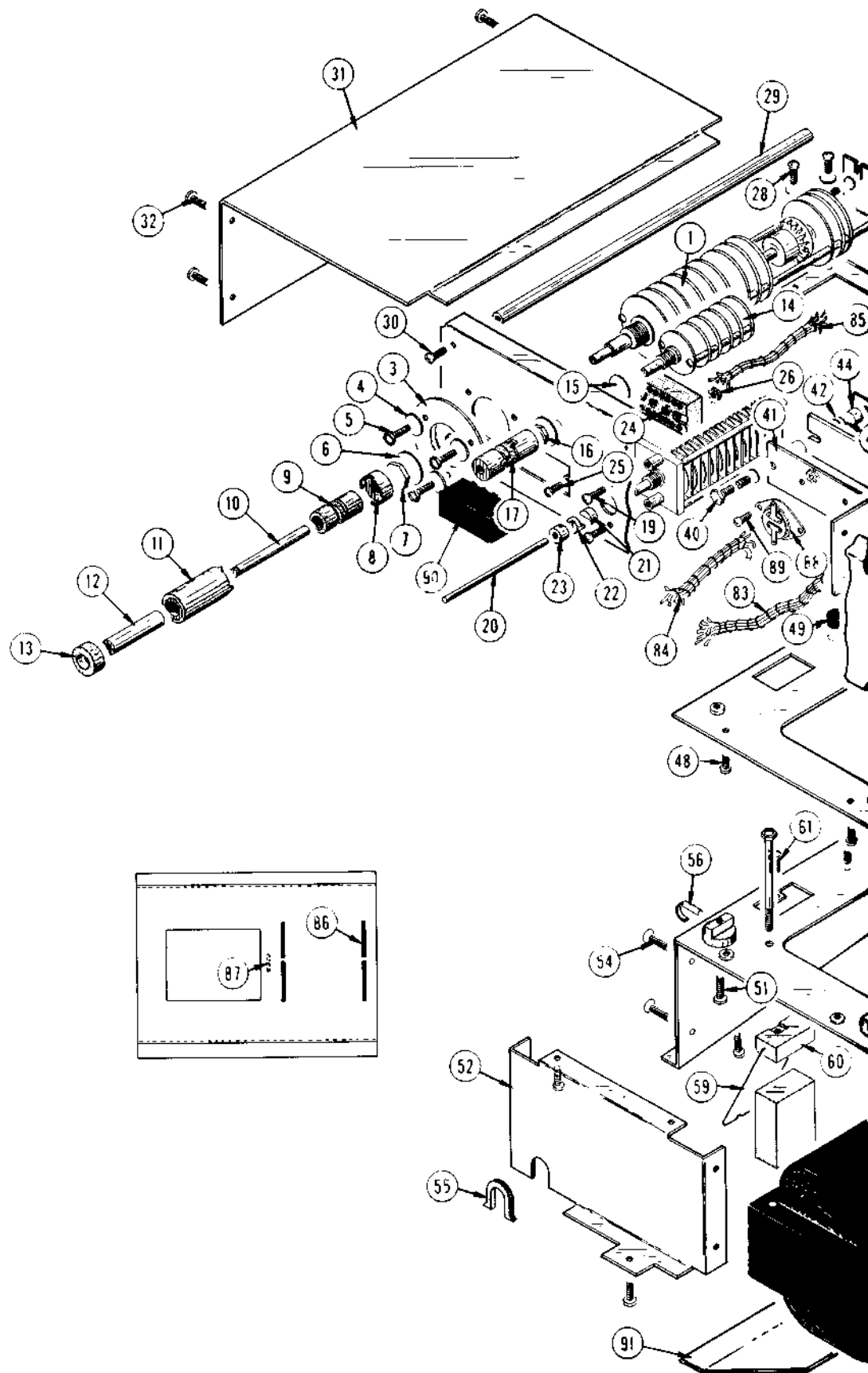
FIG. 4 COLLECTOR SUPPLY
