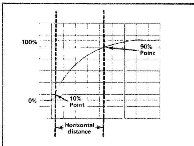
Fig. 1-9. Measuring risetime.
