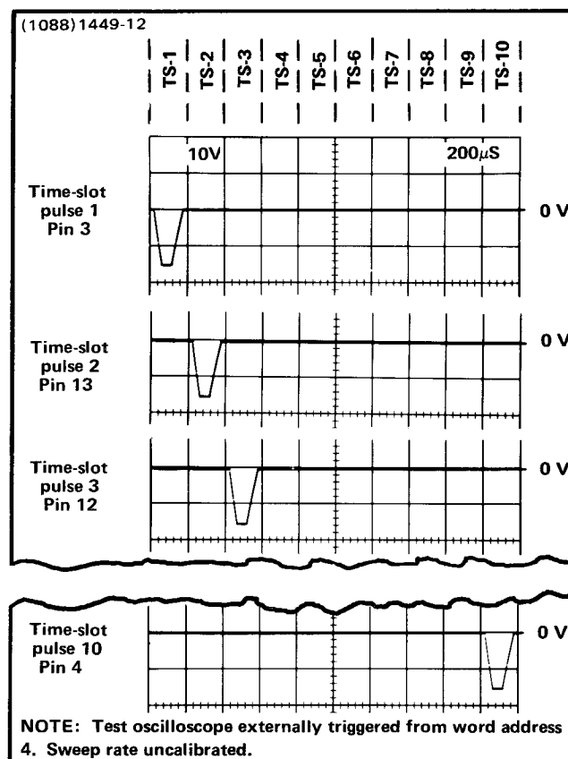
Fig. 3-5. Time relationship of the time-slot (TS) pulses produced by U1025.
