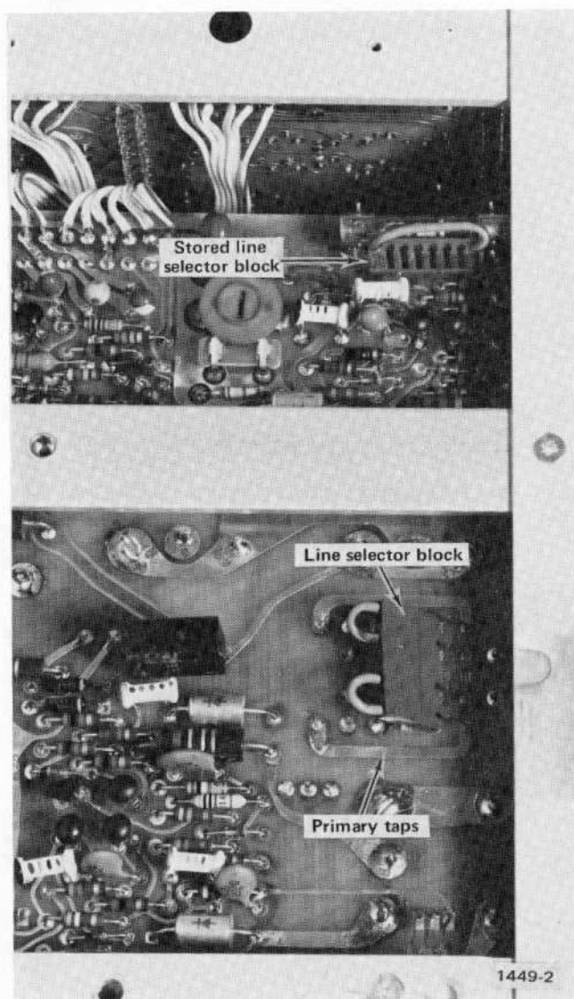
Fig. 1-3. Location of the line-selector block on the Power Supply circuit board.
