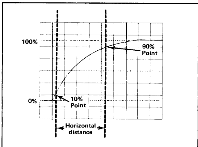
Fig. 1-9. Measuring risetime.
