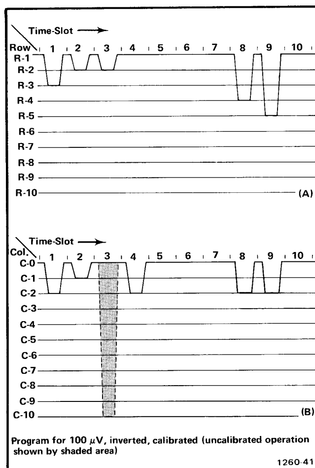
Fig. 3-7. Idealized current waveforms of: (A) Row analog data, (B) Column analog data.
