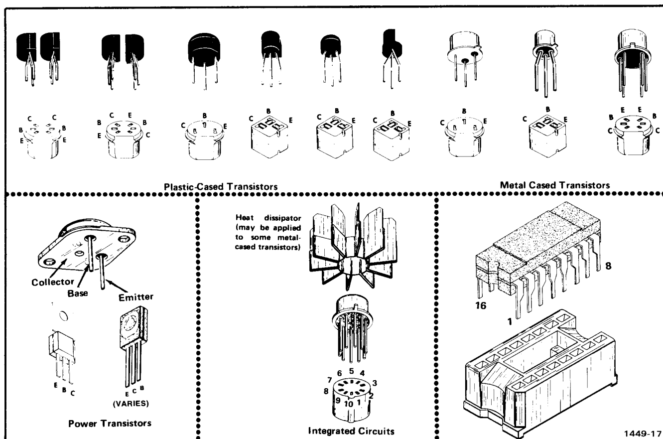
Fig. 4-2. Electrode configuration data for semiconductor devices.
