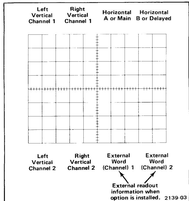
Fig. 1-2. Location of readout on the crt identifying the originating plug-in unit and channel (and external, if Option 3 is installed).
