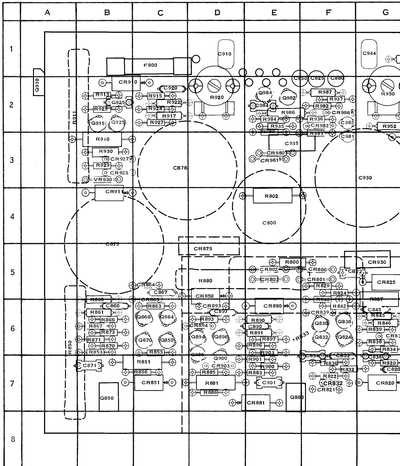
A6—Low Voltage &amp; Calibrator circuit board.
