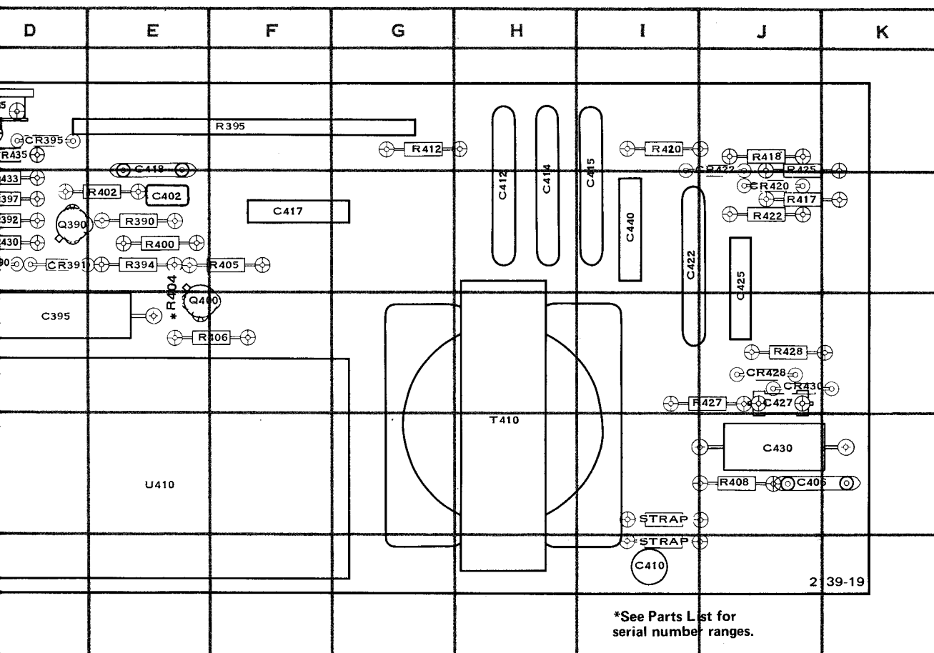
A5—High Voltage circuit board.
