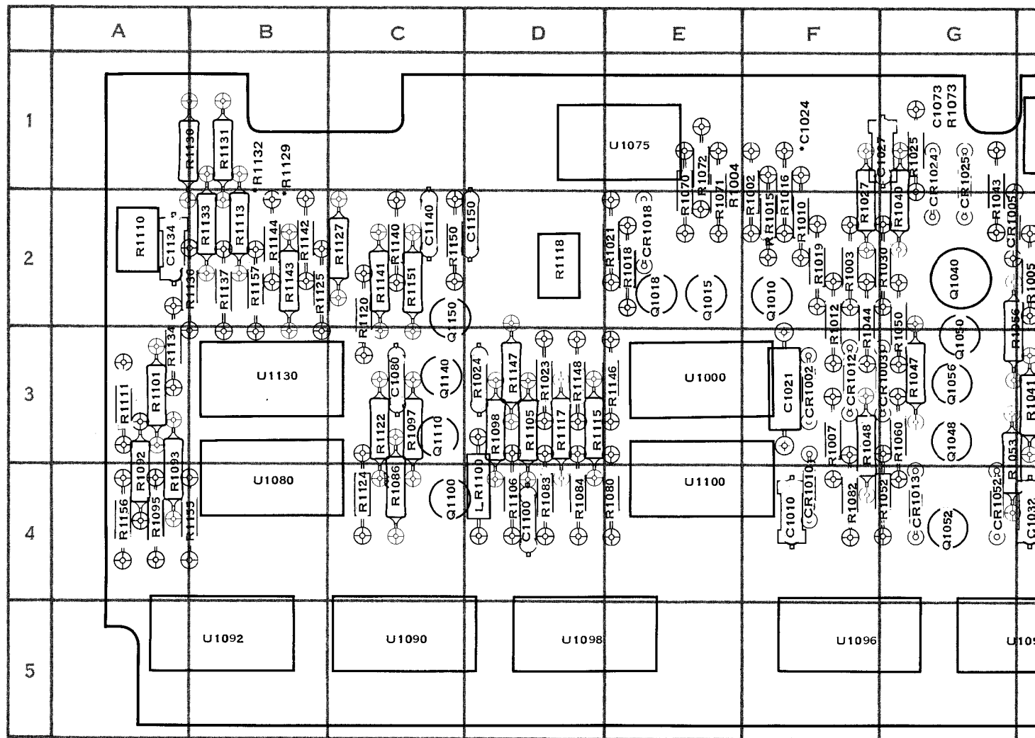
A7—Readout circuit board.
