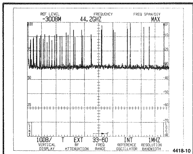
Figure 6-4. Typical display generated by a signal into the waveguide mixer.
