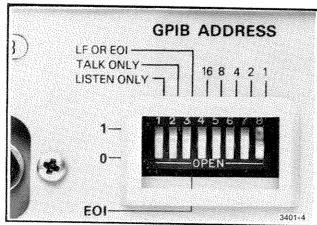
Figure 6-12. GPIB ADDRESS switch on the rear panel.
