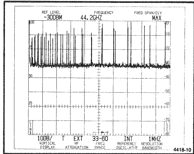
Figure 6-9. Typical display from an external mixer.
