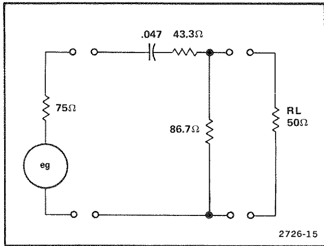
Figure 6-2. Circuit of a 75 to 50 \Omega matching pad (ac coupled).
