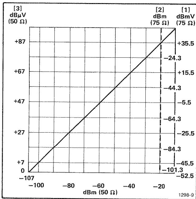
Figure 6-3. Graph to illustrate the relationship between dBm, dBmV and dB \mu V (matching attenuator included where necessary).
