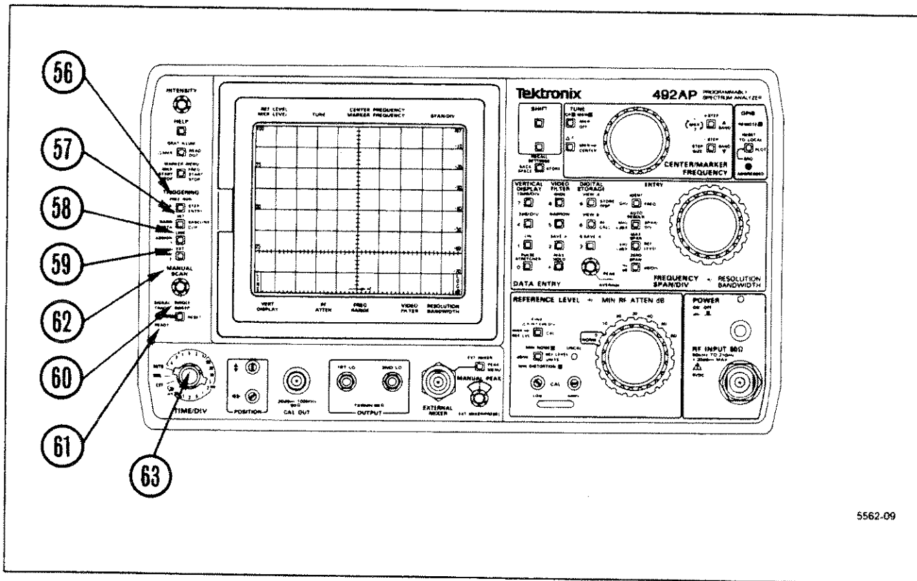
Figure 4-10. Sweep.
