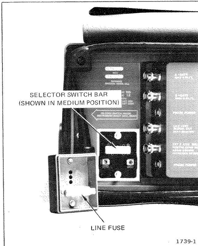
Fig. 1. Regulating range selector and line fuse.
