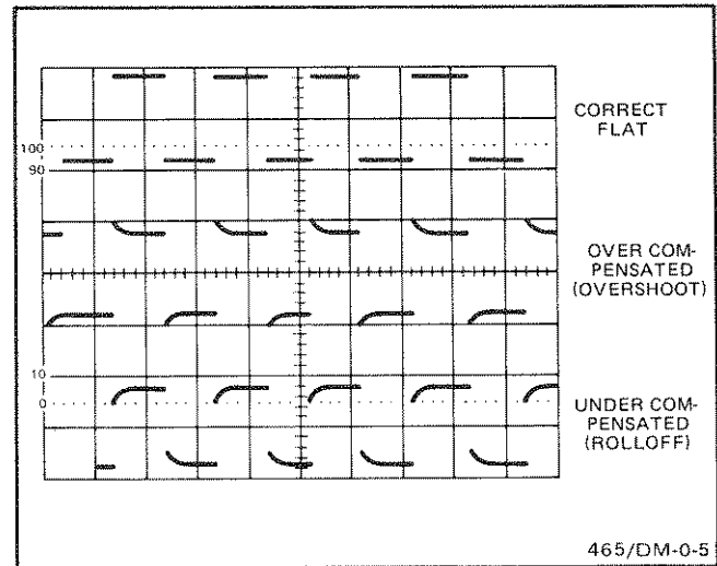
Fig. 11. Probe compensation.
