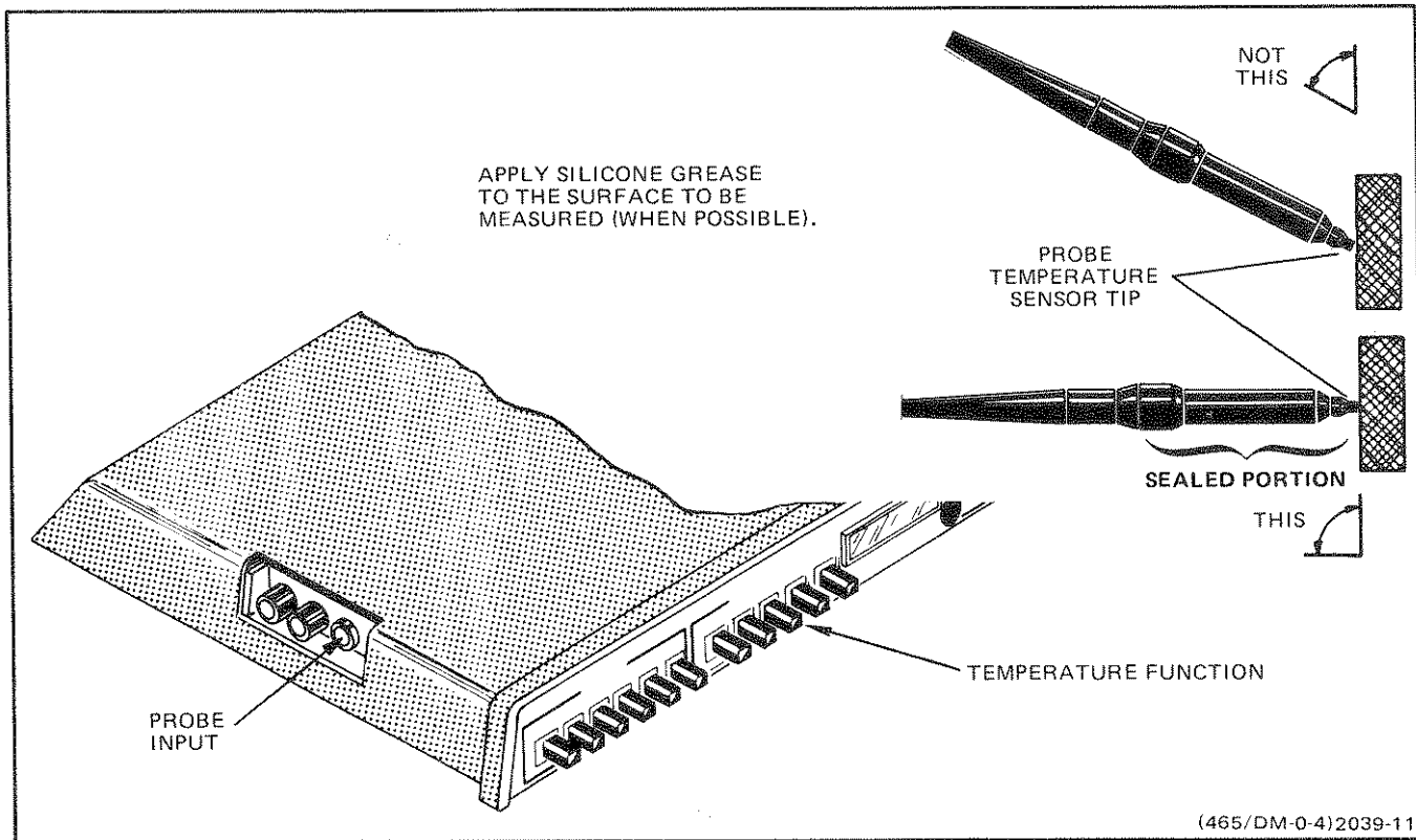
Fig. 10. Temperature.
