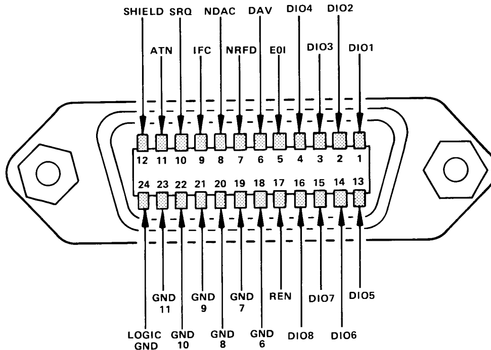
Figure 50. GPIB connector and pin assignments.
