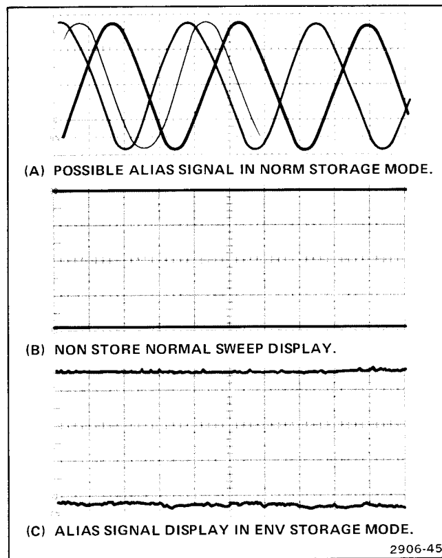
Figure 29. Anti-aliasing.
