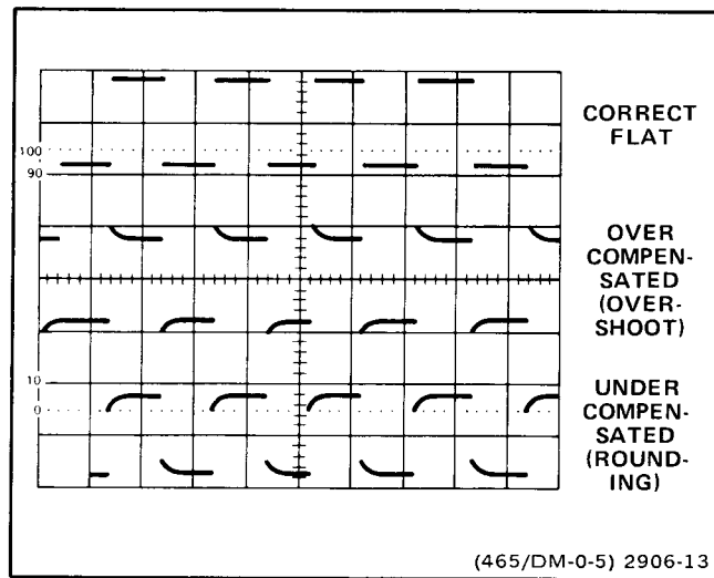
Figure 13. Probe compensation.
