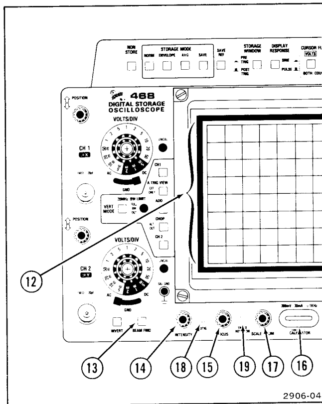
Figure 4. Display controls and CALIBRATOR.
