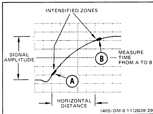
Figure 45. Rise time, differential time method.
