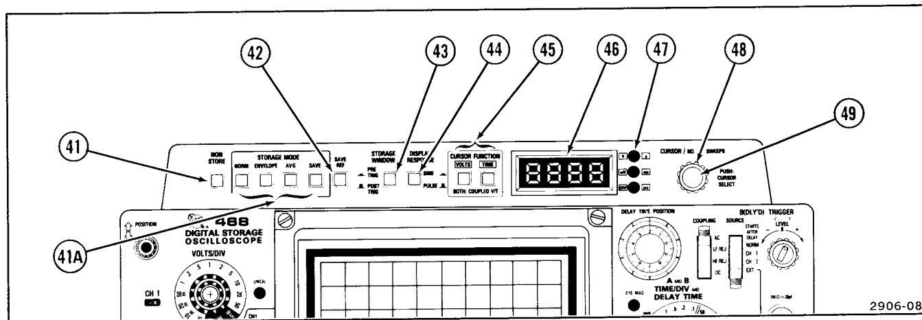
Figure 8. Digital storage controls and indicators.
