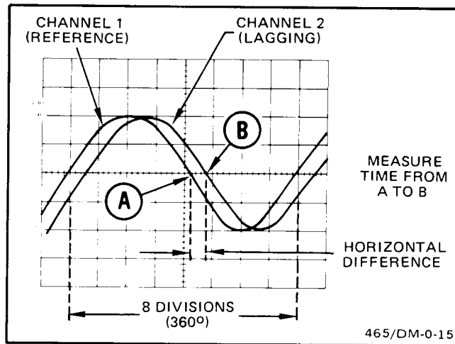
Figure 40. Phase difference.
