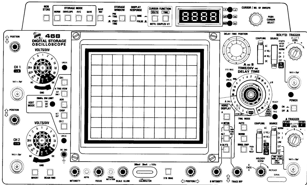
Figure 52. The 468 Oscilloscope with Option 05.
