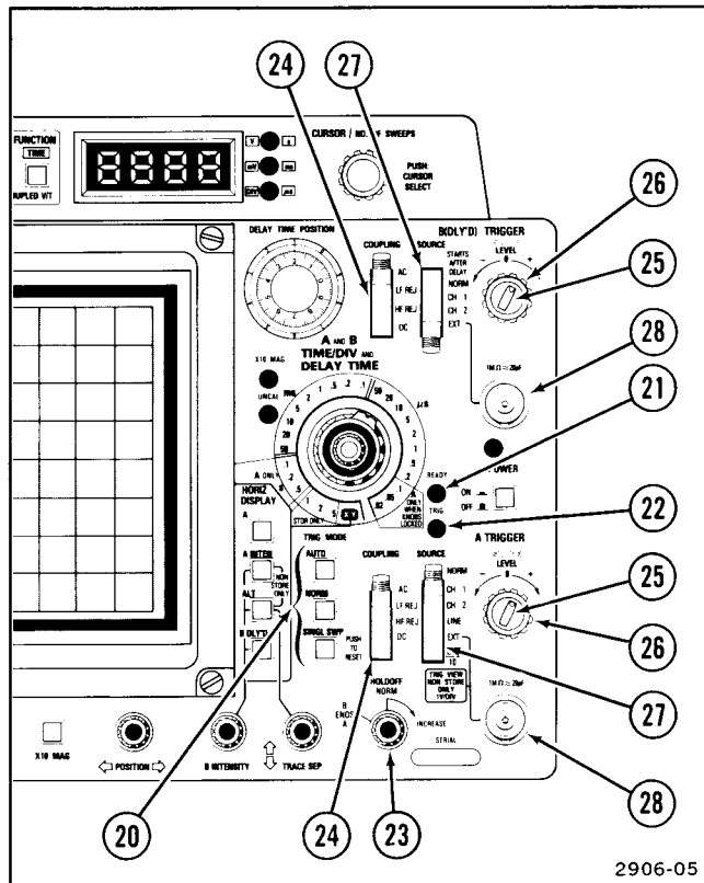
Figure 5. Trigger controls, connectors, and indicators.
