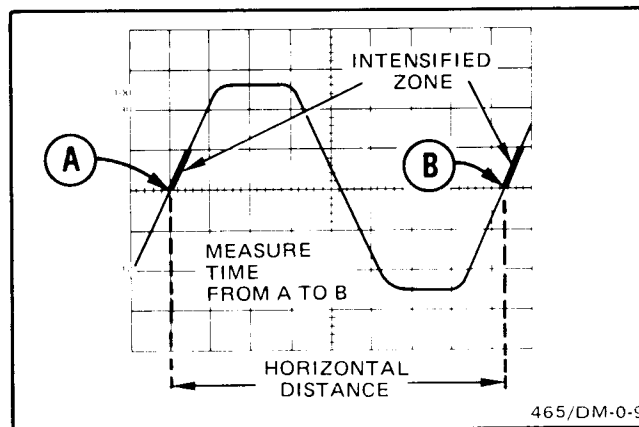
Figure 43. Time duration using delayed sweep.
