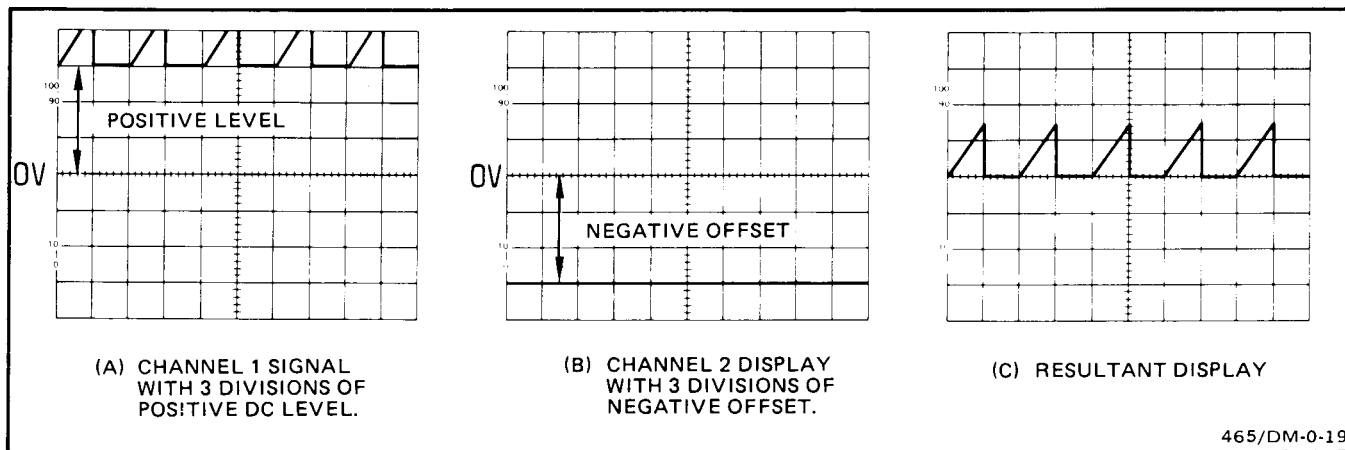
Figure 35. Algebraic addition.
