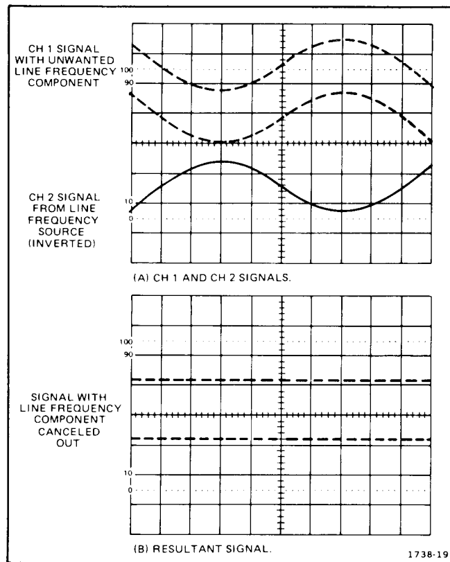
Figure 36. Common-mode rejection.
