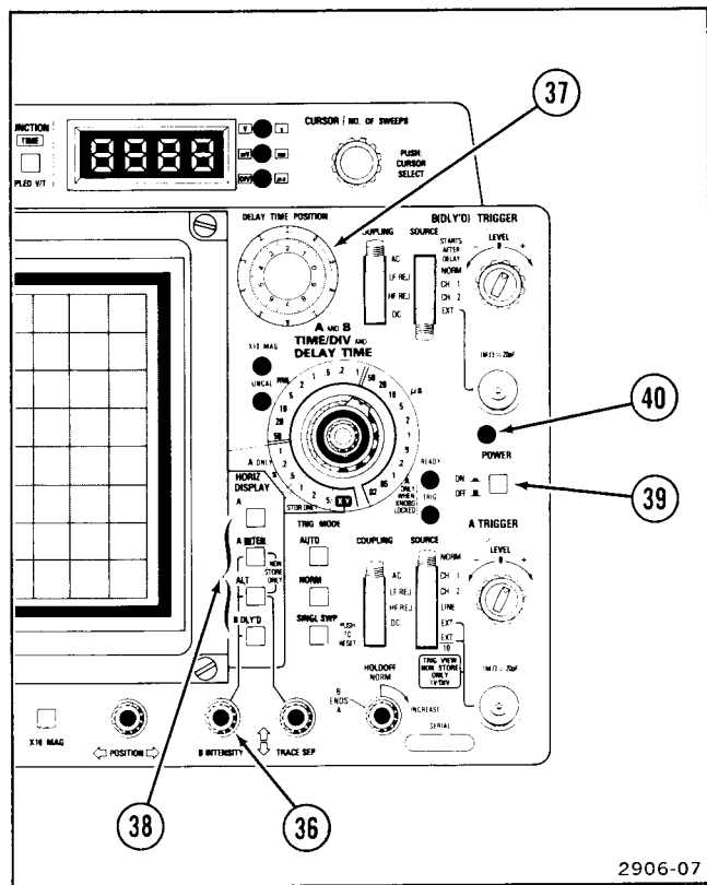
Figure 7. Horizontal display, B INTENSITY, DELAY TIME POSITION, and power controls and indicator.
