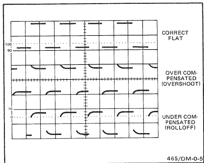
Fig. 11. Probe compensation.
