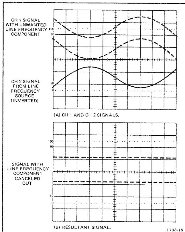
Fig. 17. Common-mode rejection.
