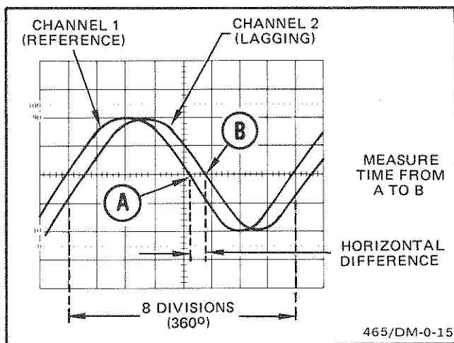
Fig. 21. Phase difference.
