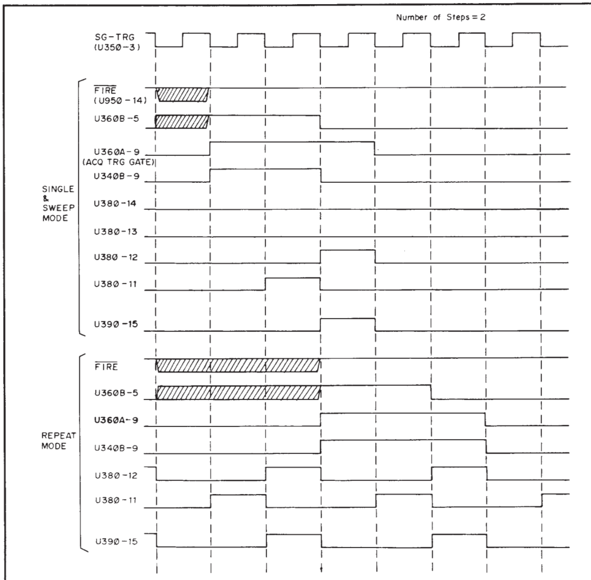
Figure 2-2. Step generator timing.
