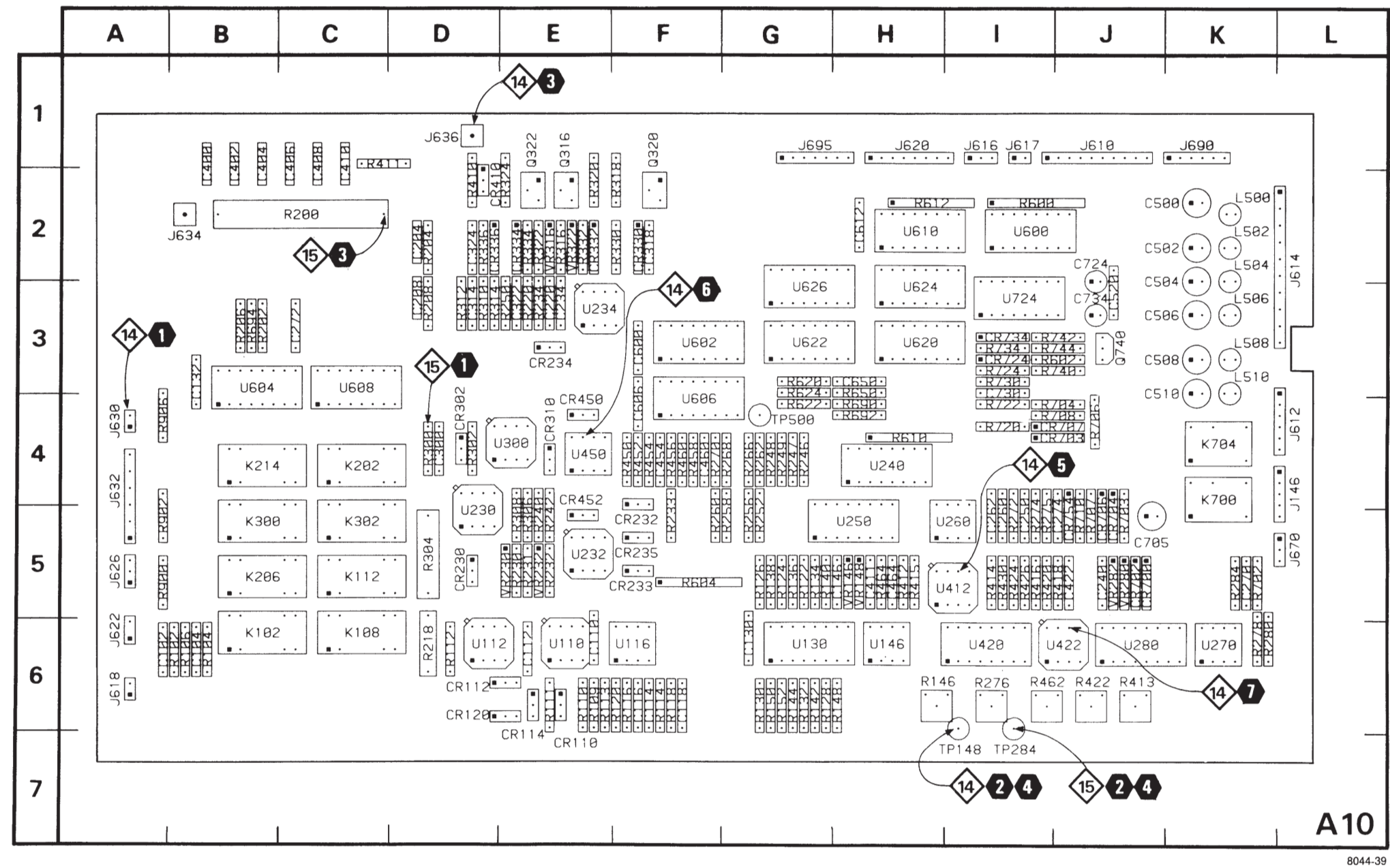
Figure 7-11. A10—Sense circuit board assembly.
