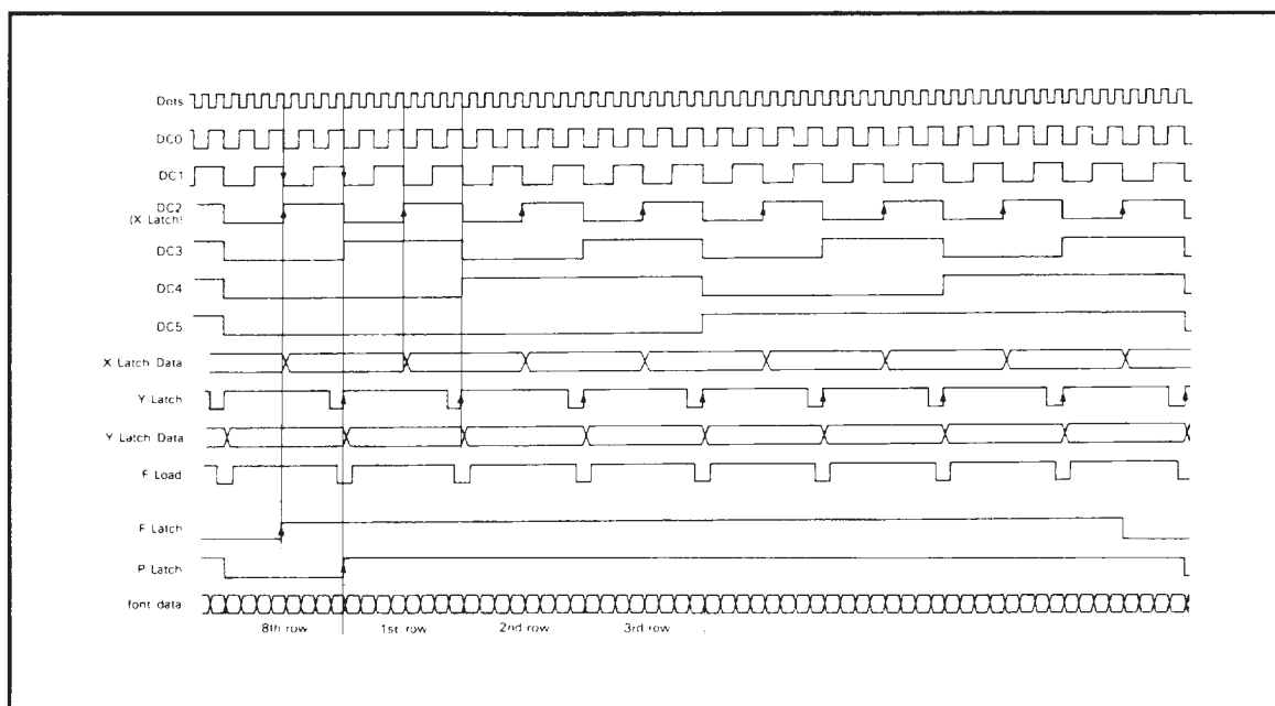
Figure 2-6. Display timing.
