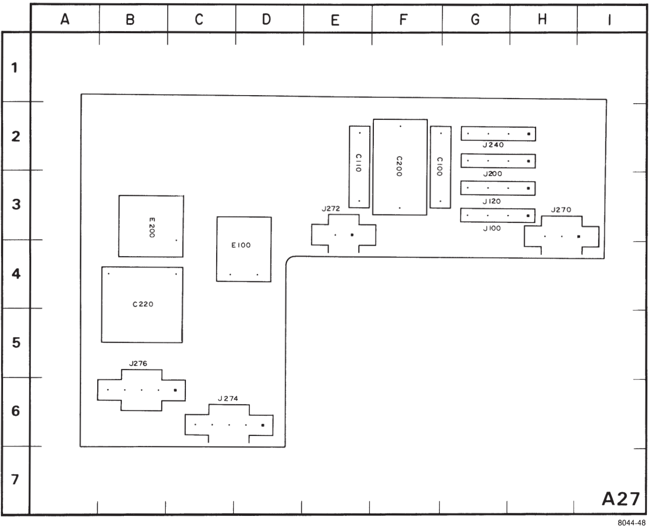
Figure 7-21. A27—Primary circuit board assembly.
