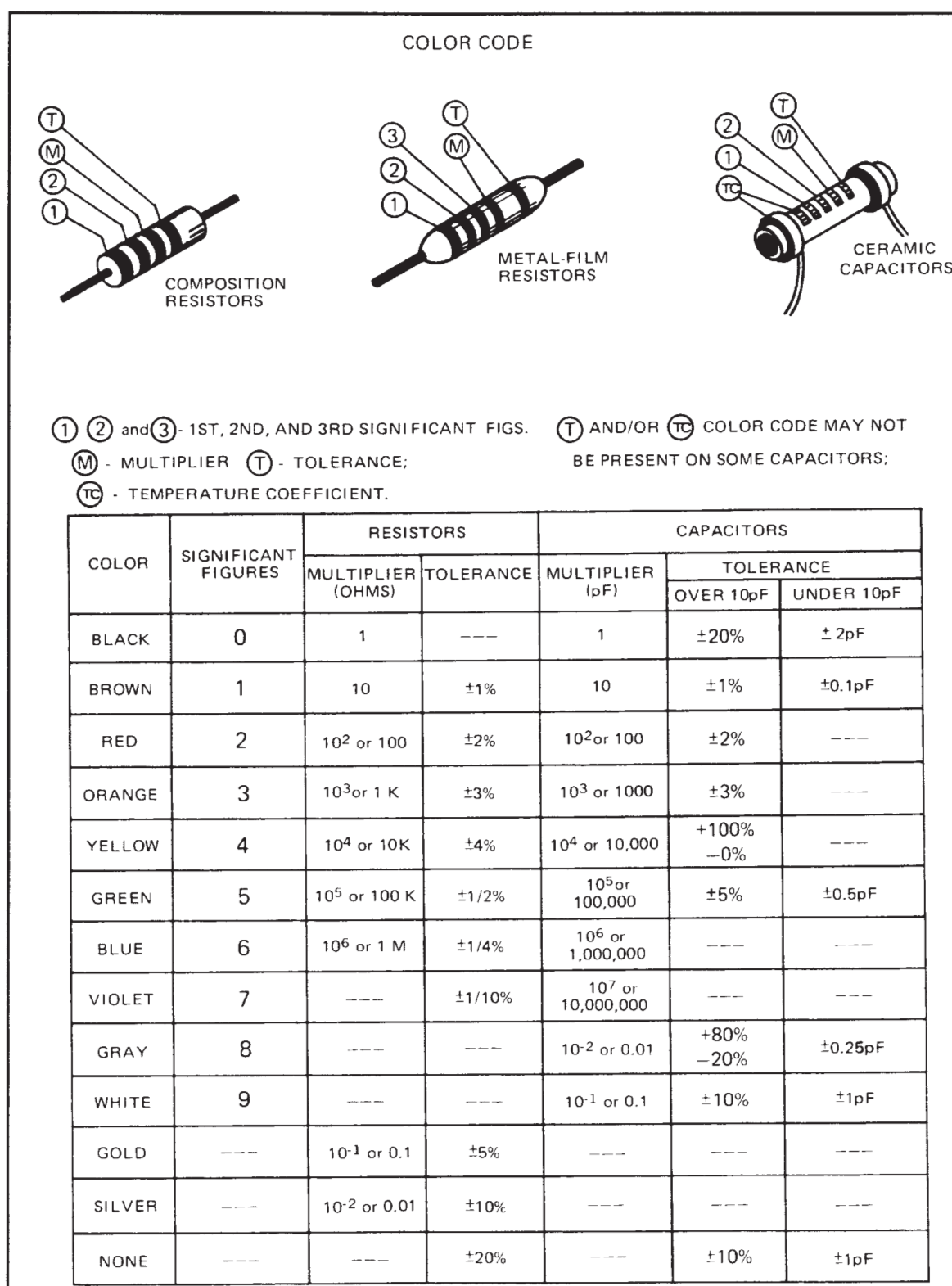
Figure 3-1. Resistor and capacitor color coding.
