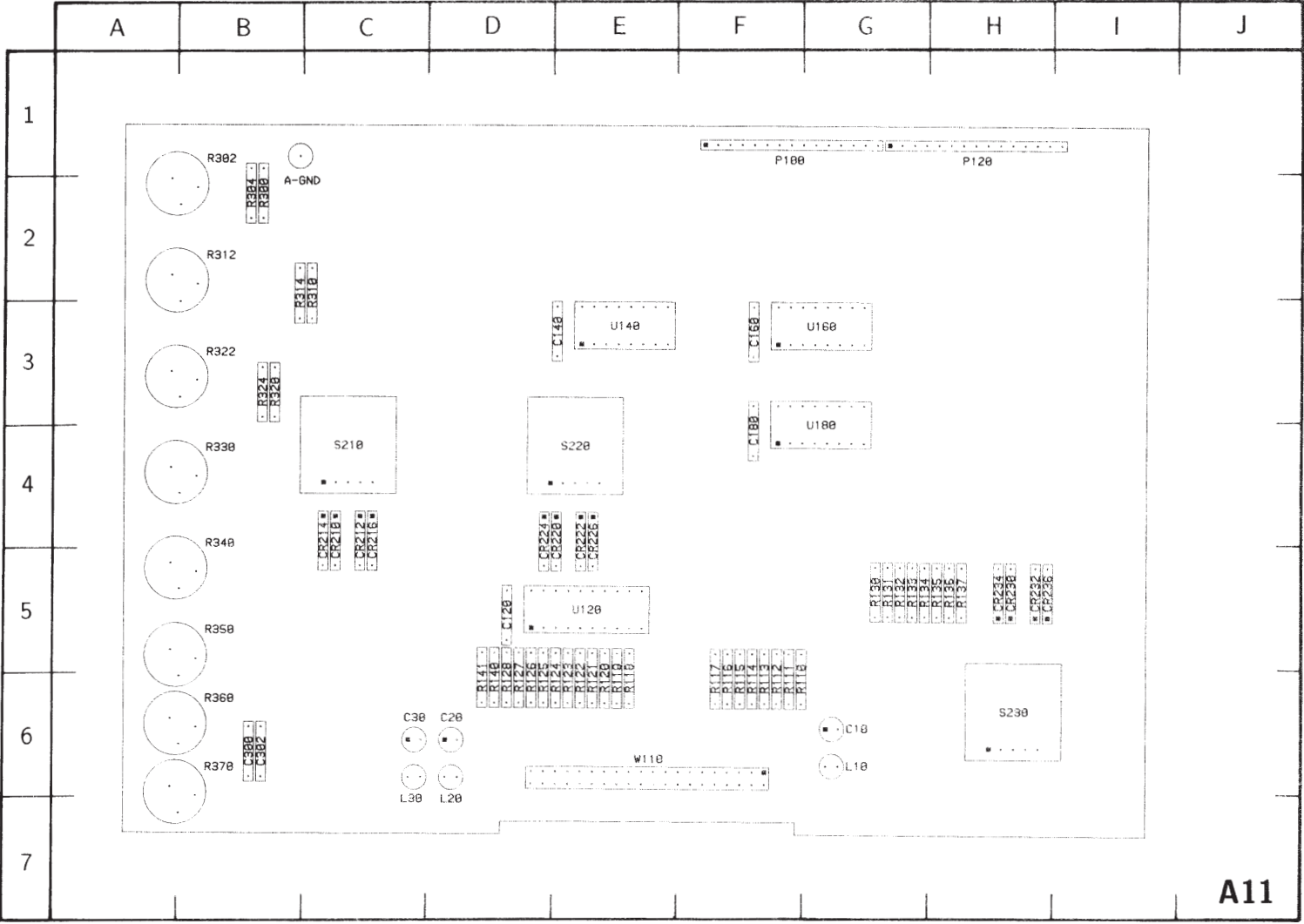
Figure 7-12. A11—Main Key circuit board assembly.
