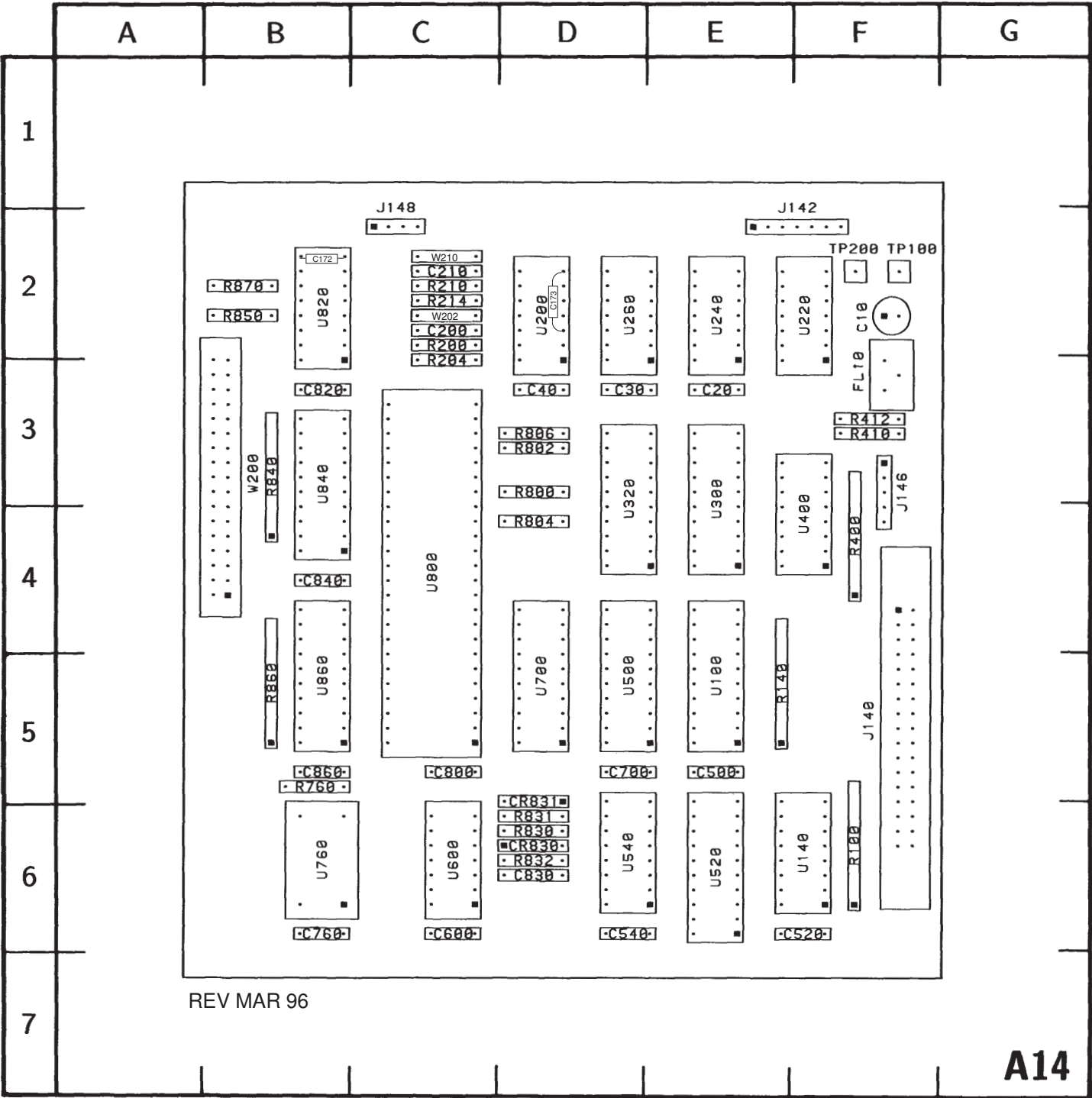
Figure 7-14. A14—Lower Key & FDD circuit board assembly.
