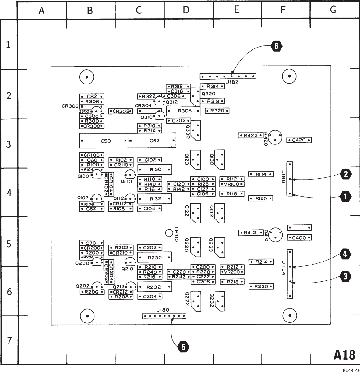
Figure 7-17. A18—CRT Output circuit board assembly.
