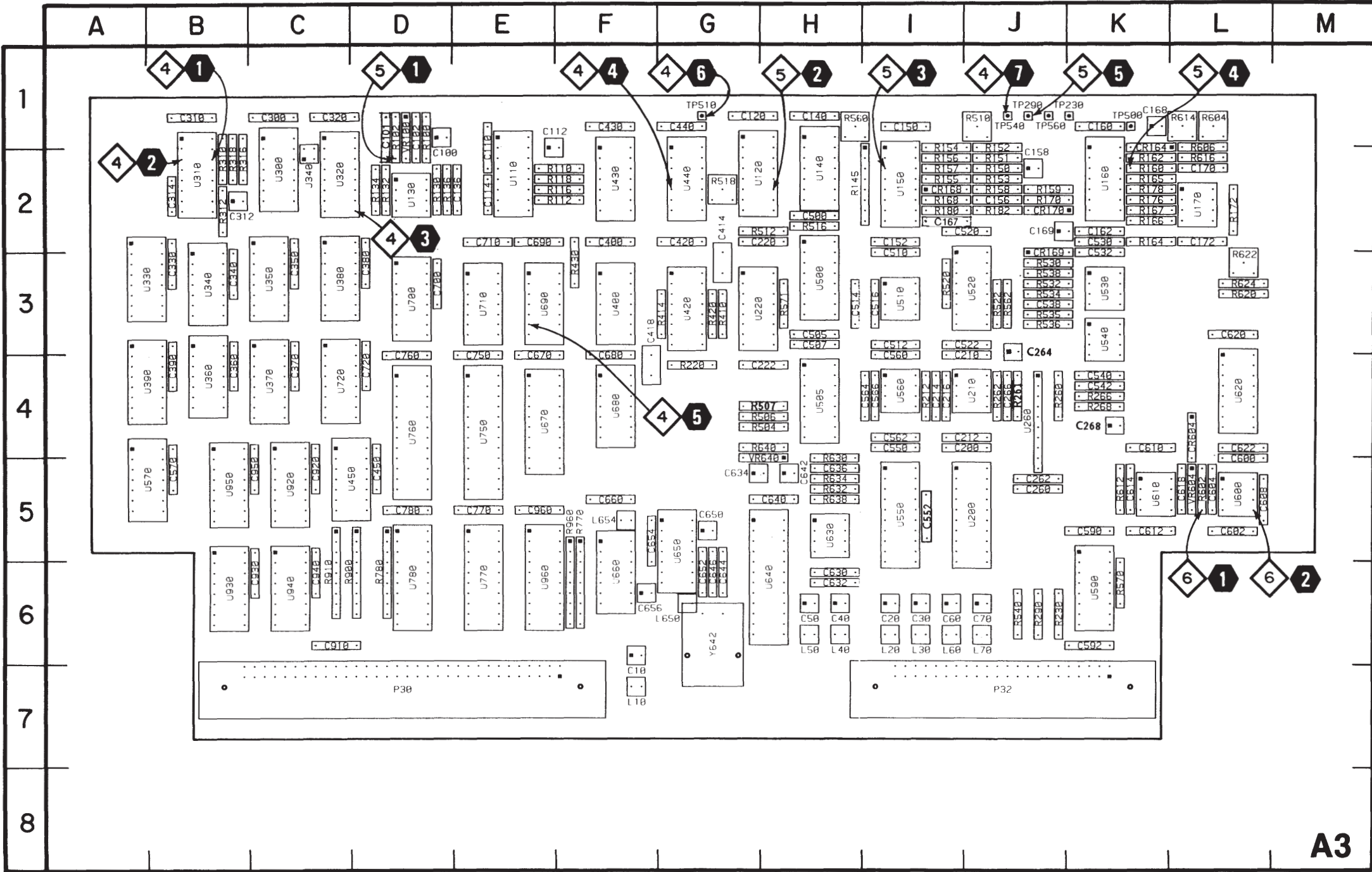
Figure 7-5. A3—A/D circuit board assembly.
