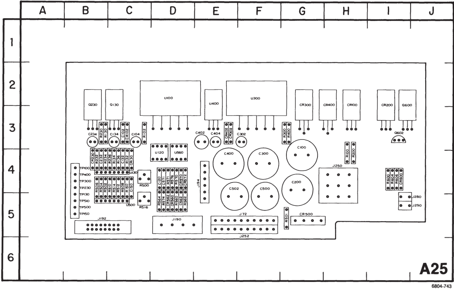
Figure 7-20. A25—Main Power Supply circuit board assembly.
