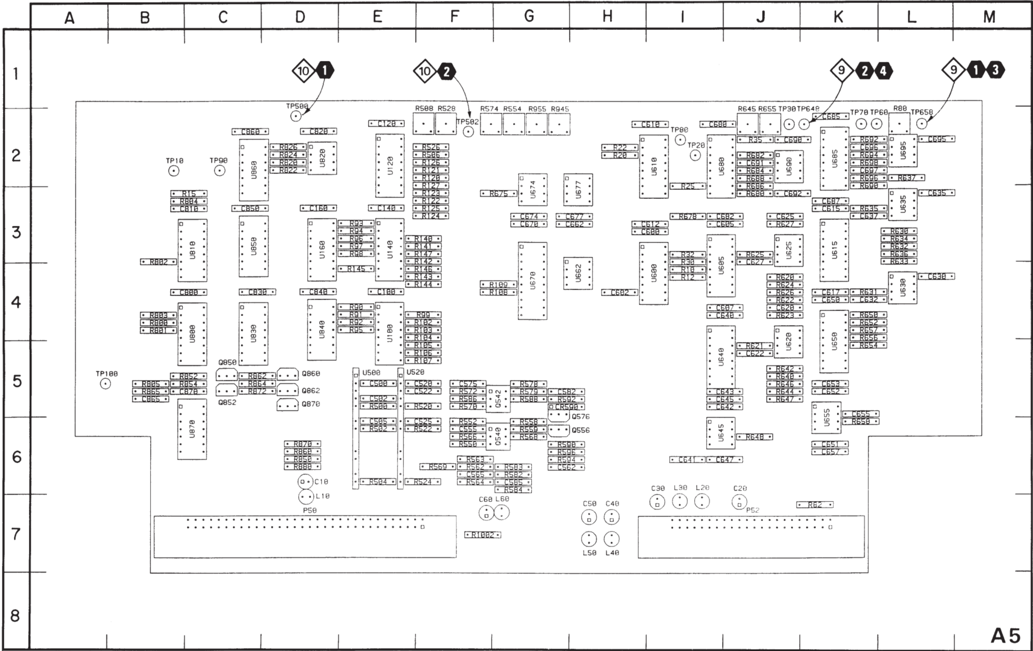
Figure 7-7. A5—Display Control circuit board assembly.
