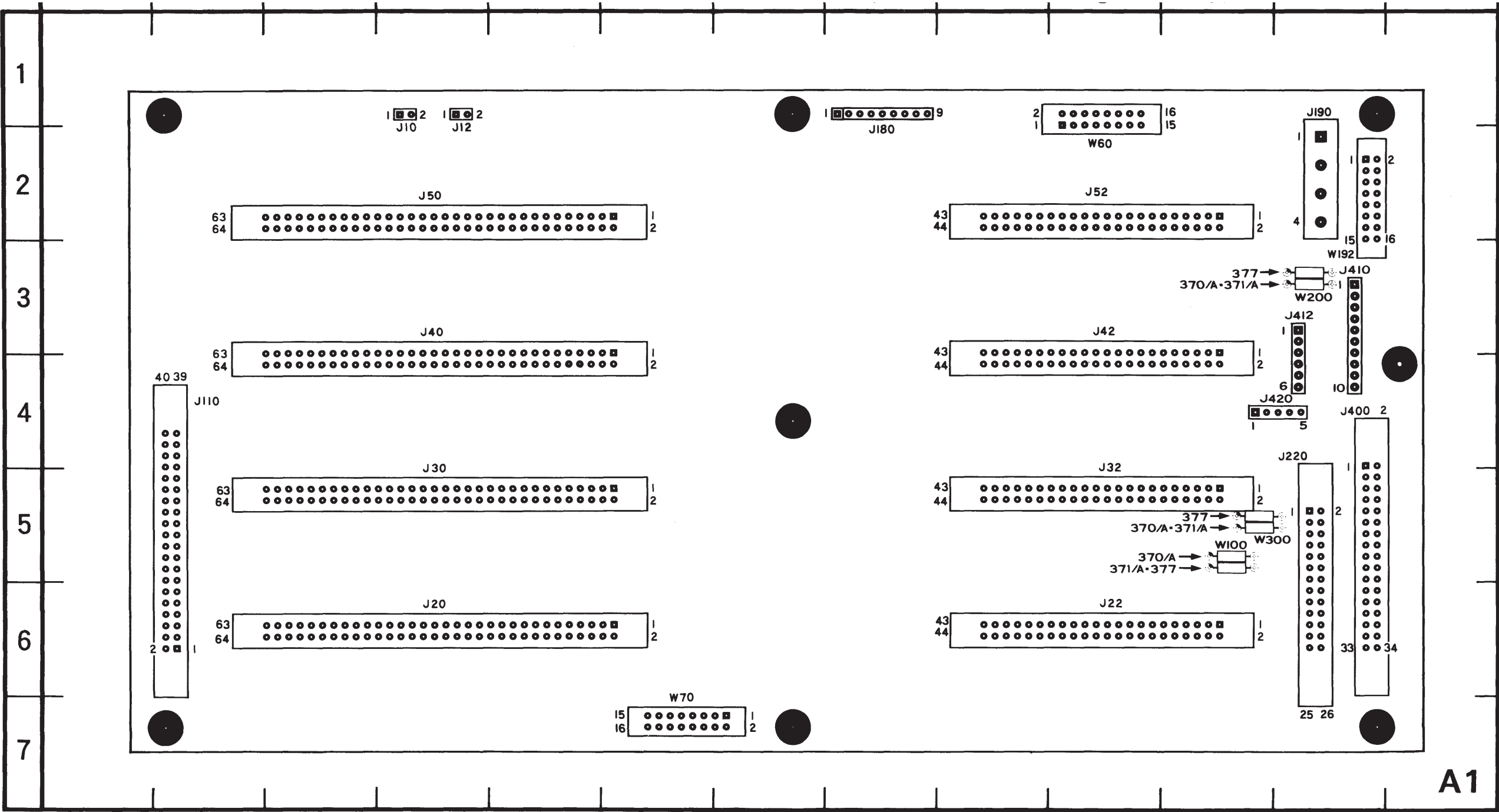
Figure 7-3. A1—Mother circuit board assembly.
