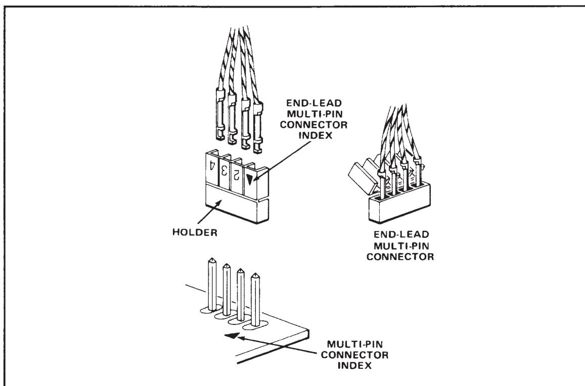
Figure 3-3. Connector pin indexing.
