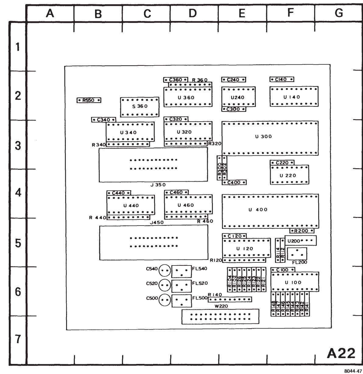
Figure 7-19. A22—Interface circuit board assembly.
