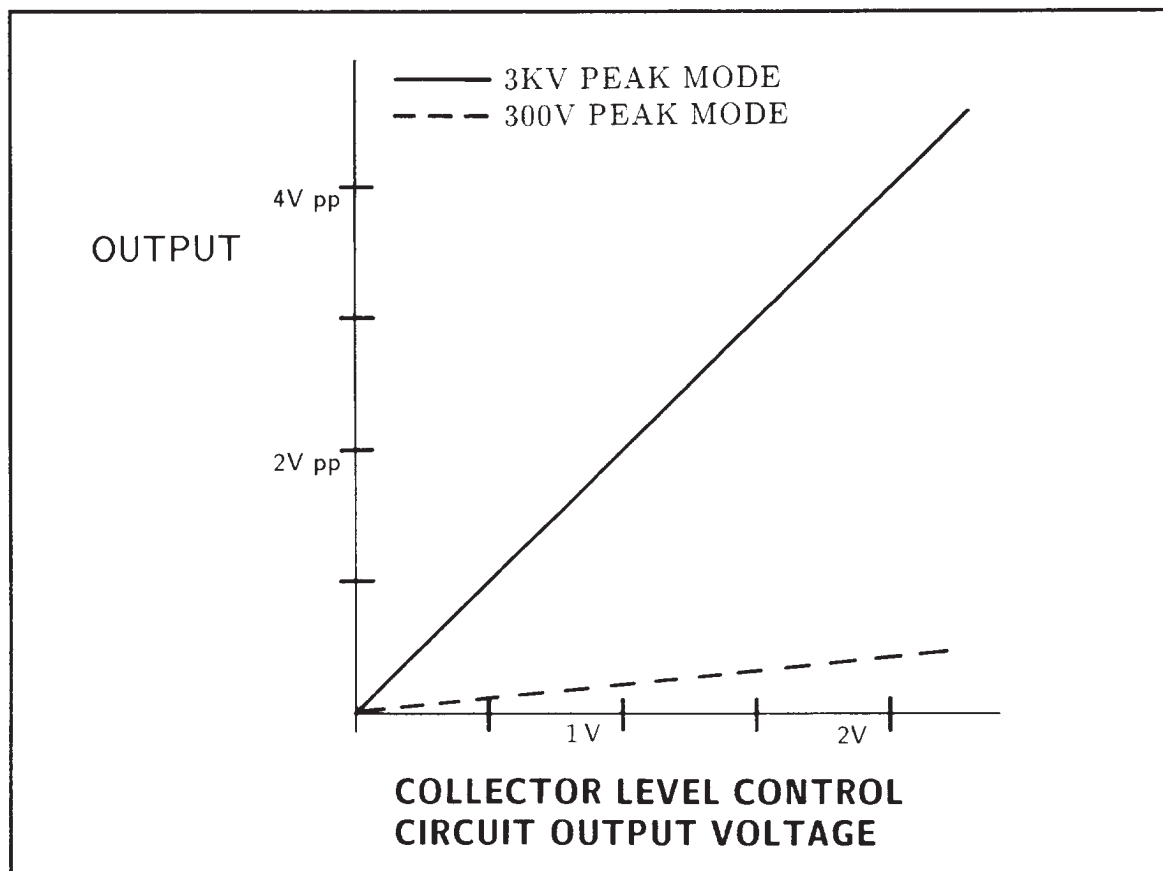
Figure 2-4. VCA characteristic.
