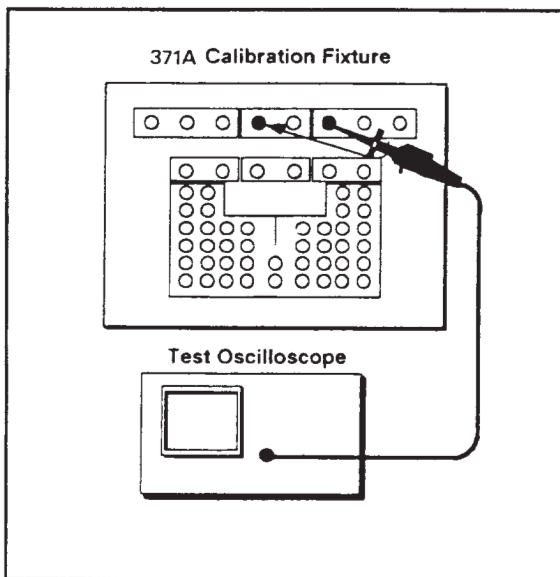
Figure 4-13. Calibration Fixture connections for checking ripple pulse noise of voltage source mode.
