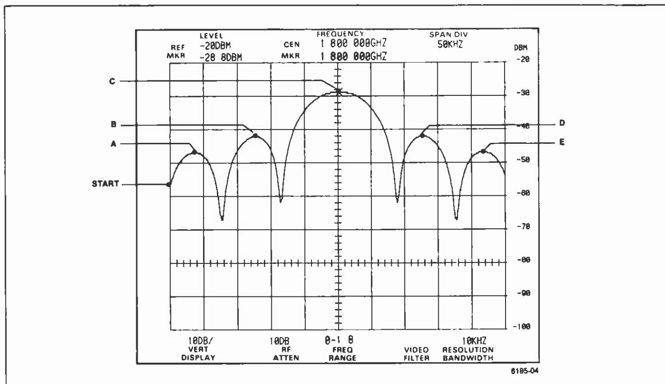
Figure 5-6. Signal finding example.
