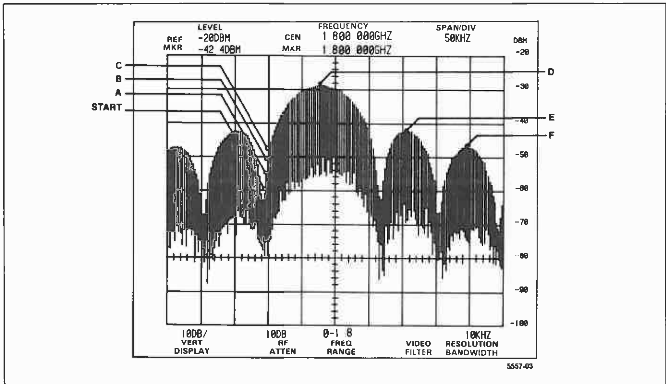
Figure 5-3. Signal finding example.
