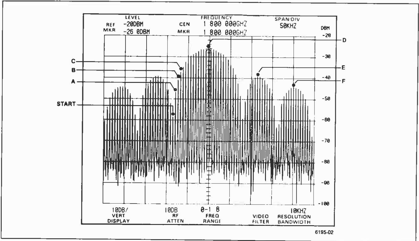
Figure 5-4. Signal finding example.
