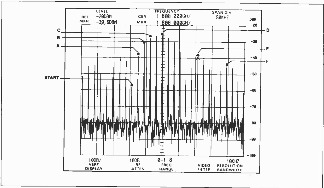
Figure 5-5. Signal finding example.
