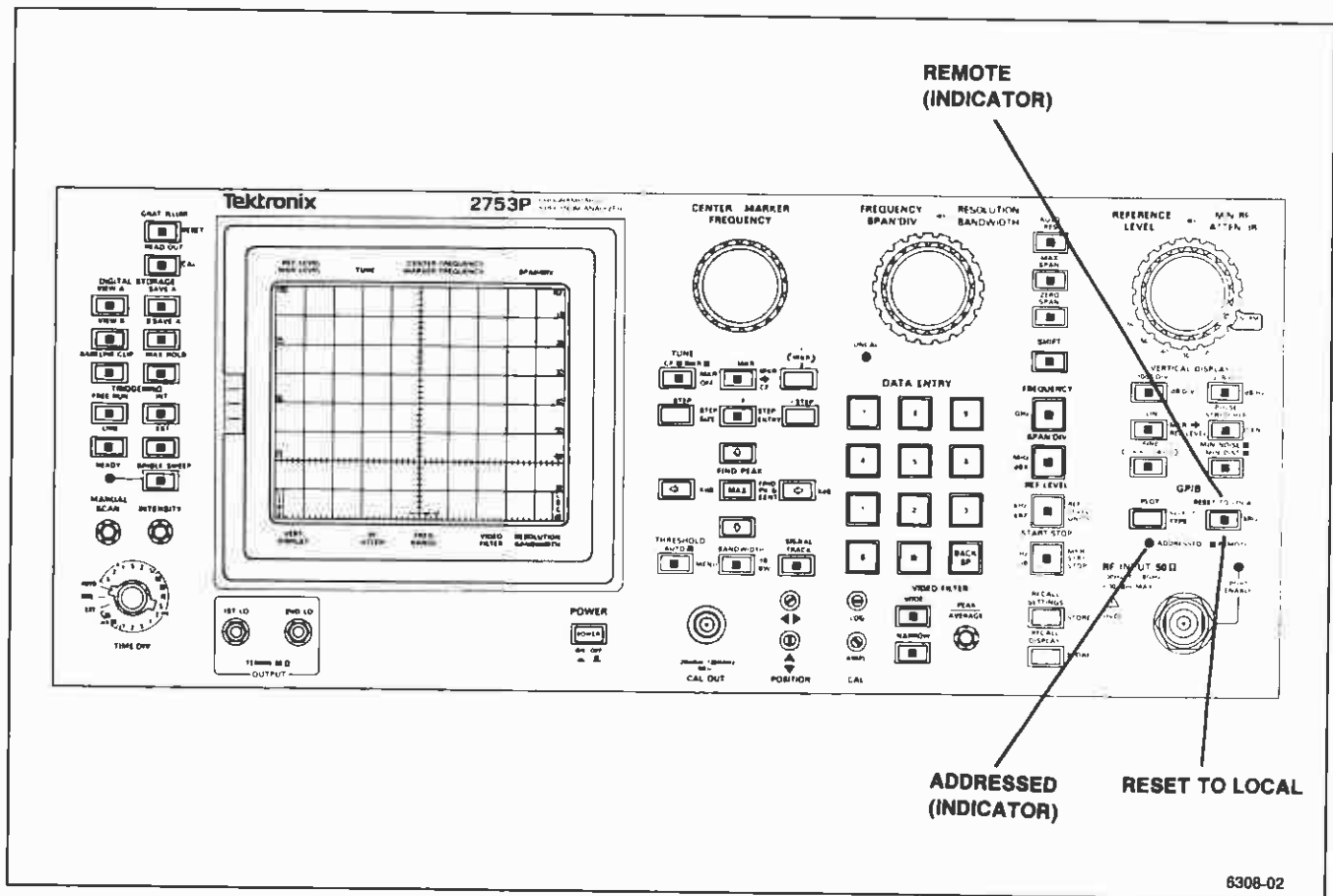
Figure 1-1. GPIB pushbutton and indicators.
