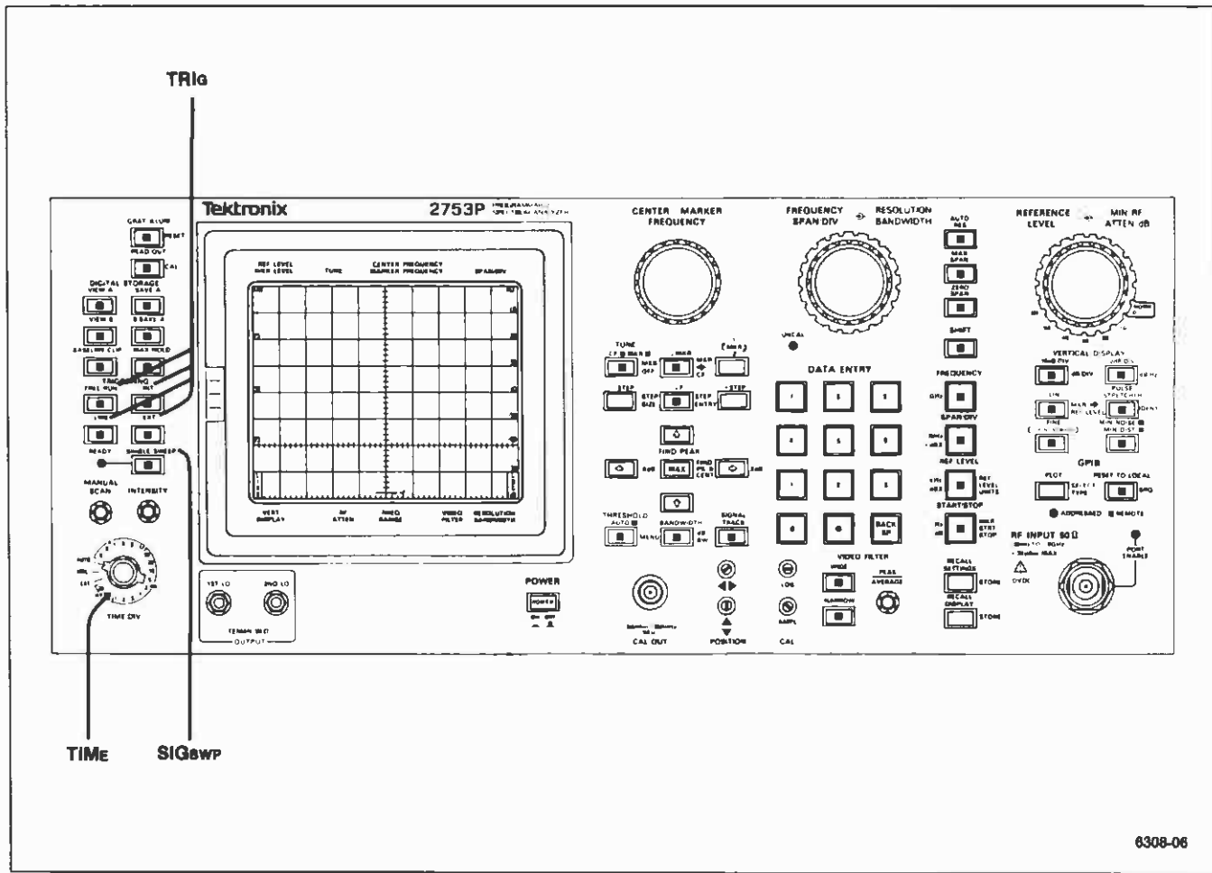
Figure 4-4. Front-panel Sweep Control commands.
