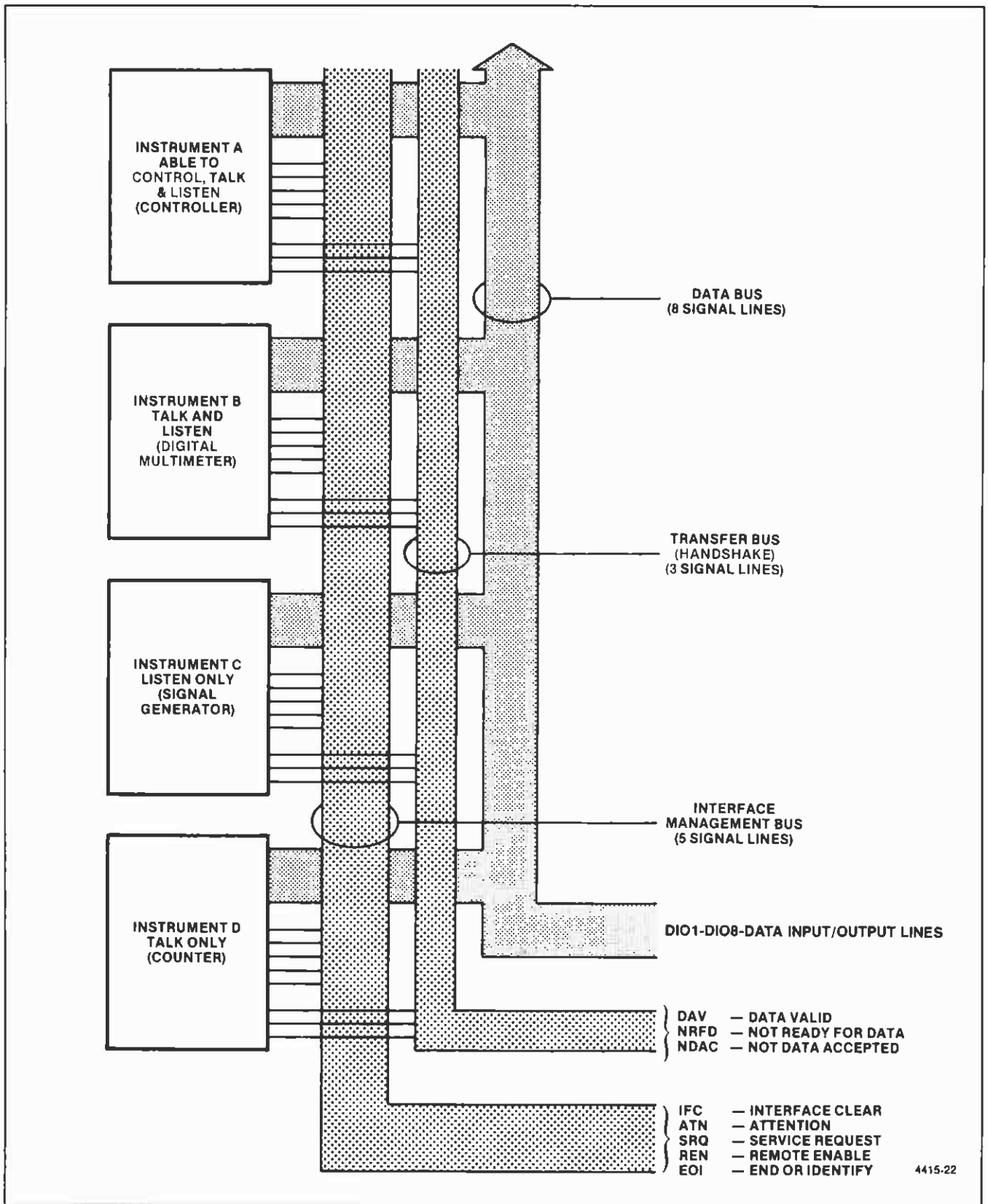
Figure A-2. A typical GPIB system.
