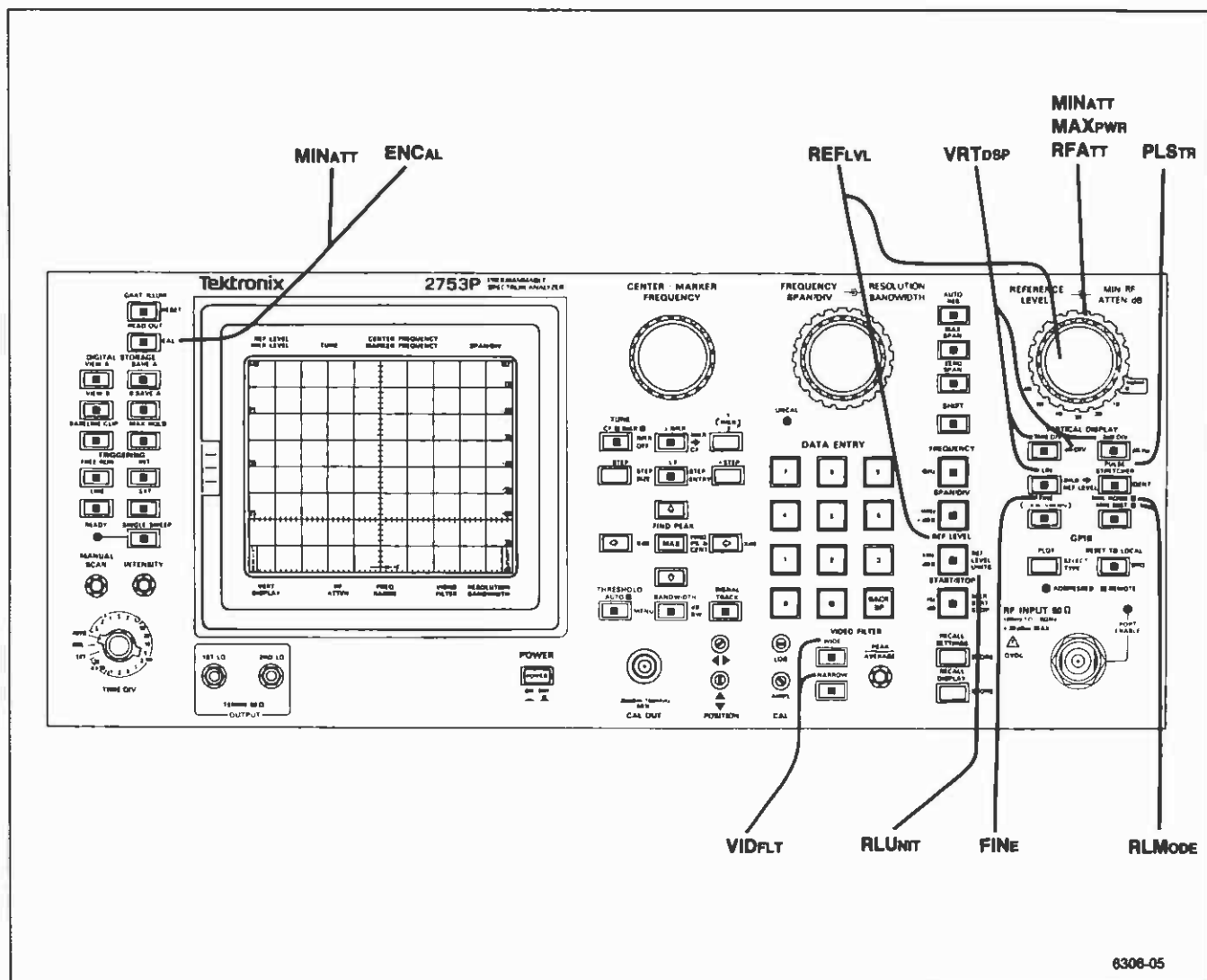
Figure 4-3. Front-panel Vertical Display and Reference Level commands.
