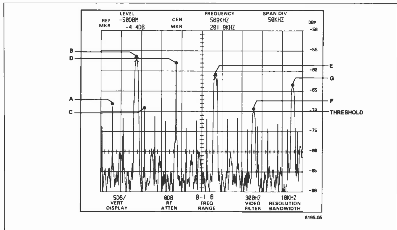
Figure 5-7. Signal finding example.
