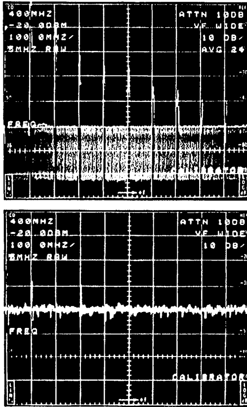
Figure 6-6. Average signal plus noise and average signal-plus-noise subtracted from the current sweep.
