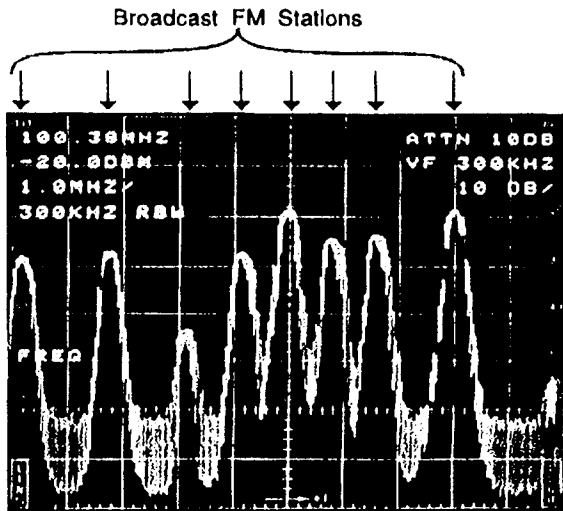
Figure 6-13. Portion of U.S. broadcast FM band.
