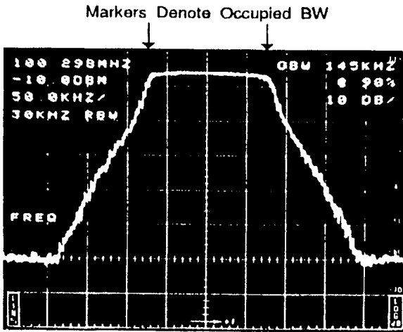
Figure 6-14. OCCUPIED BW mode with MAX HOLD.
