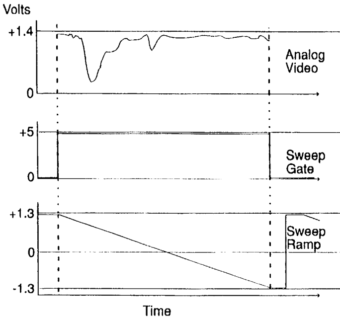
Figure 7-2. Sweep gate and ramp timing.
