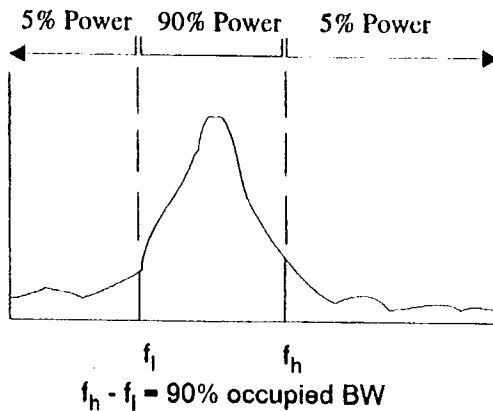
Figure 6-12. Illustration of Occupied BW measurement.
