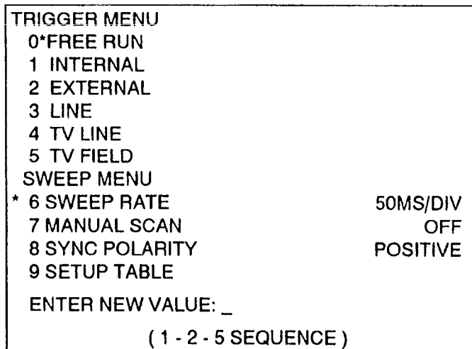
Figure 6-3. Sweep/Trigger Menu with SWEEP RATE selection chosen.
