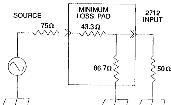
Figure 6-4. 75/50 ohm matching minimum loss pad.
