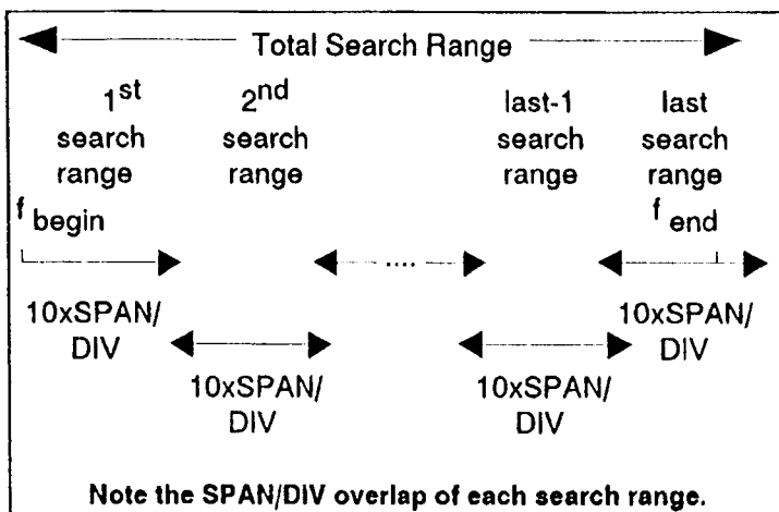
Figure 6-11. The SIGNAL SEARCH frequency range.
