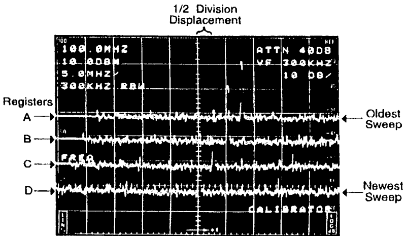
Figure 5-1. Example of a waterfall display.
