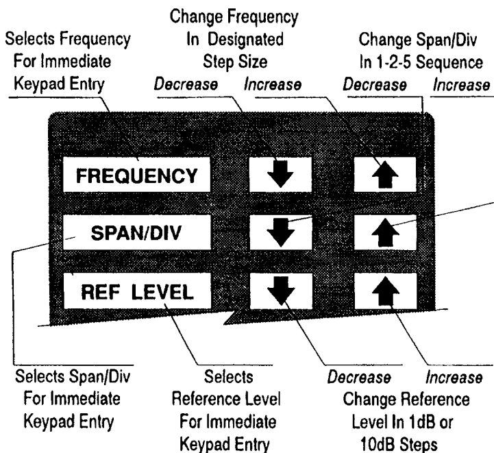
Figure 3-3. The 2712 primary controls.
