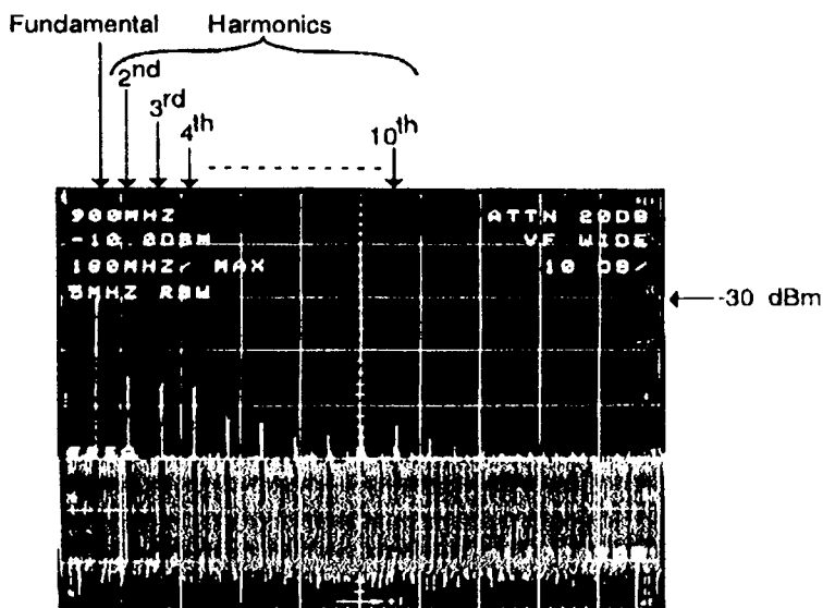
Figure 3-4. 2712 calibration signal and harmonics.
