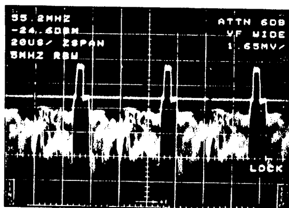
Figure 6-20. Video signal using continuous horizontal line triggering.
