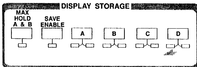
Figure 4-6. Display register control.
