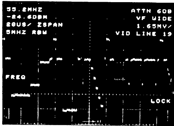
Figure 6-21. Video signal using knob-selectable horizontal line triggering (VITS visible).
