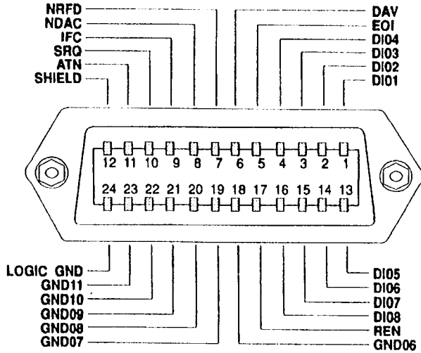
Figure 7-3. IEEE Standard 488 (GPIB) connector pin assignments.
