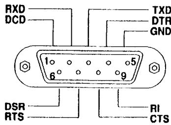
Figure 7-4. EIA Standard RS-232 (C) connector pin assignments.
