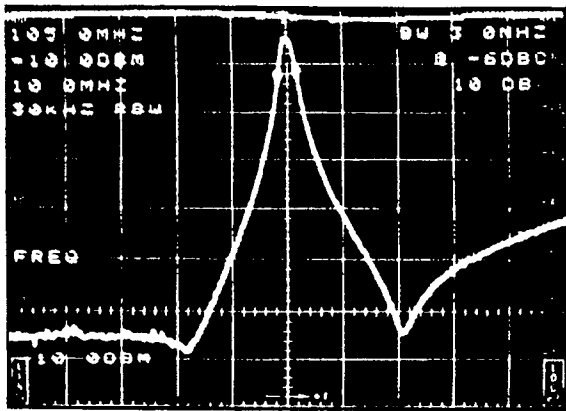
Figure 6-18. Bandpass filter response using the 2712 optional tracking generator and B,C MINUS A mode.
