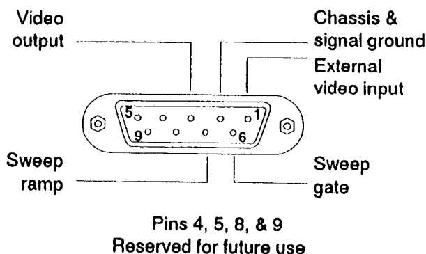
Figure 7-1. Accessory connector (J103).
