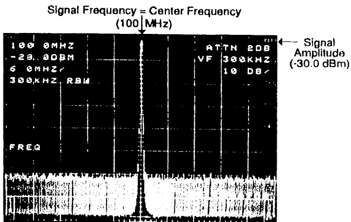
Figure 3-5. Calibration signal fundamental.
