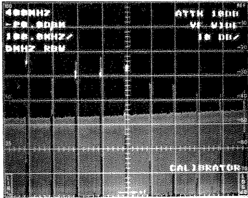
Average calibration signal plus noise
