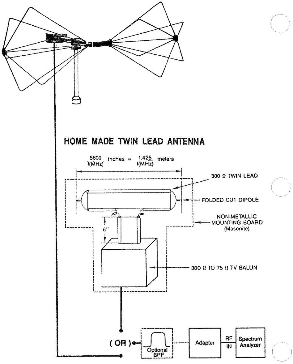
Figure 4-5. Equipment setup for field strength measurements.
