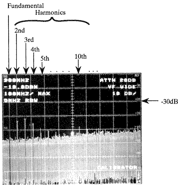
Figure 2-2. 2710 calibration signal and harmonics.
