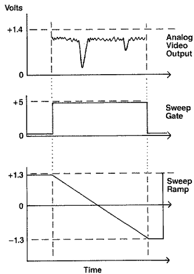
Figure 5-1. Sweep gate and ramp timing.
