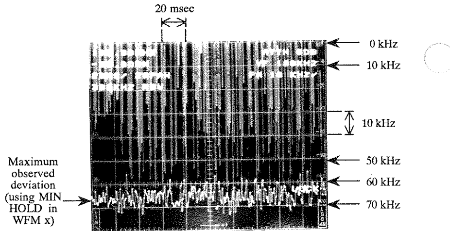
Figure 4-12. Instantaneous frequency deviation and maximum observed deviation.
