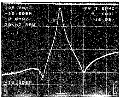
Figure 4-14B. Bandpass filter response using the 2710 optional tracking generator and B,C MINUS A mode.
