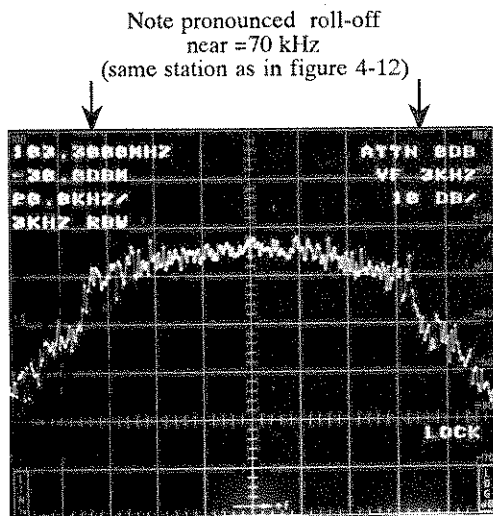
Figure 4-13. Frequency deviation by MAX HOLD technique.
