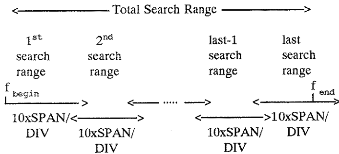
Figure 4-14. The SIGNAL SEARCH frequency range.
