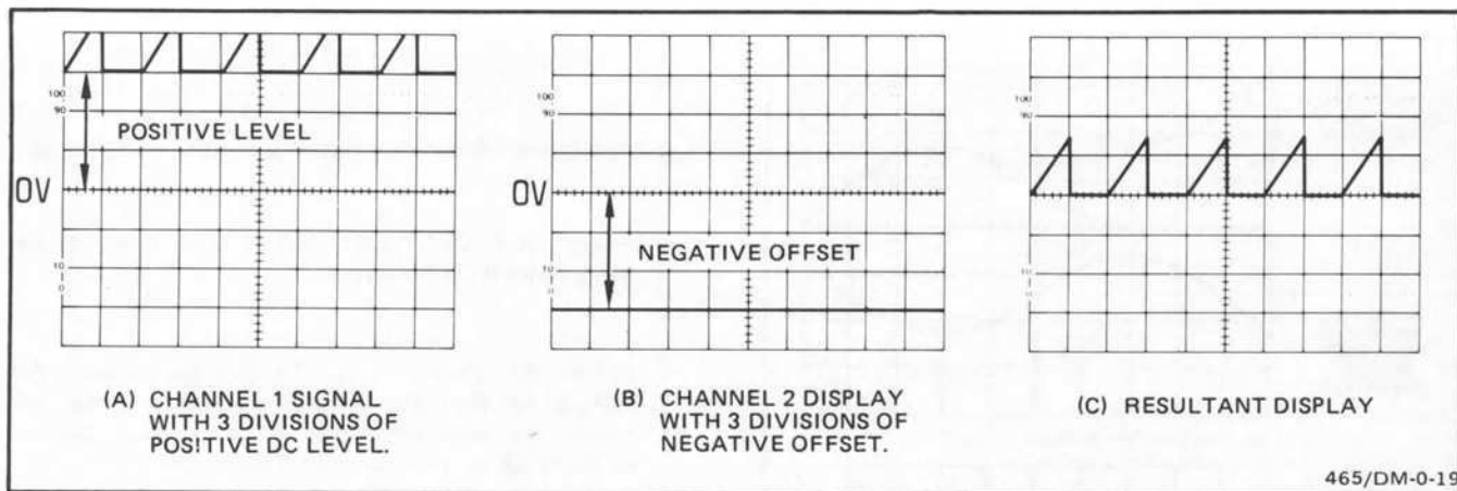
Figure 15. Algebraic addition.
