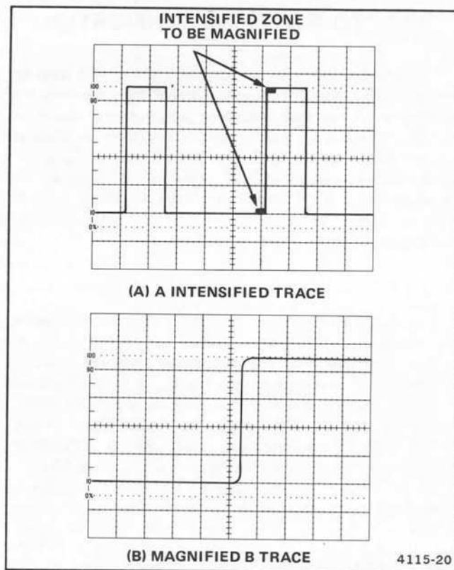
Figure 22. Delayed-sweep magnification.
