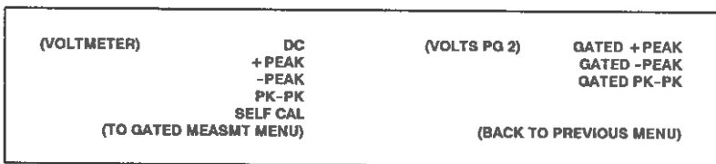
Voltmeter and Gated Voltmeter Selection Menus
