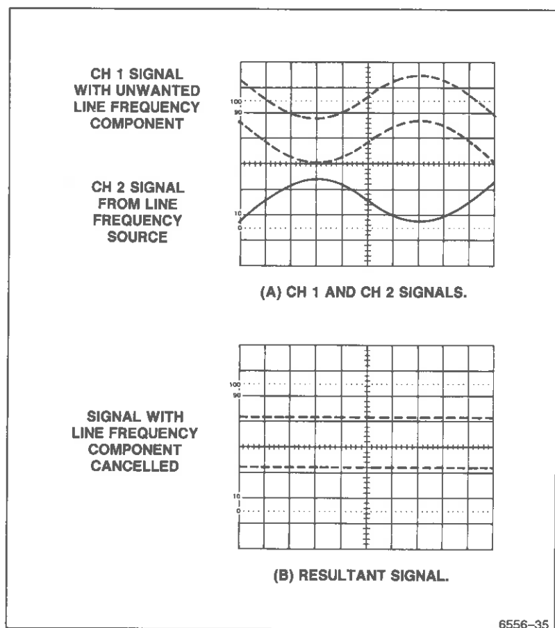
Figure 5-9. Eliminating common-mode signals.
