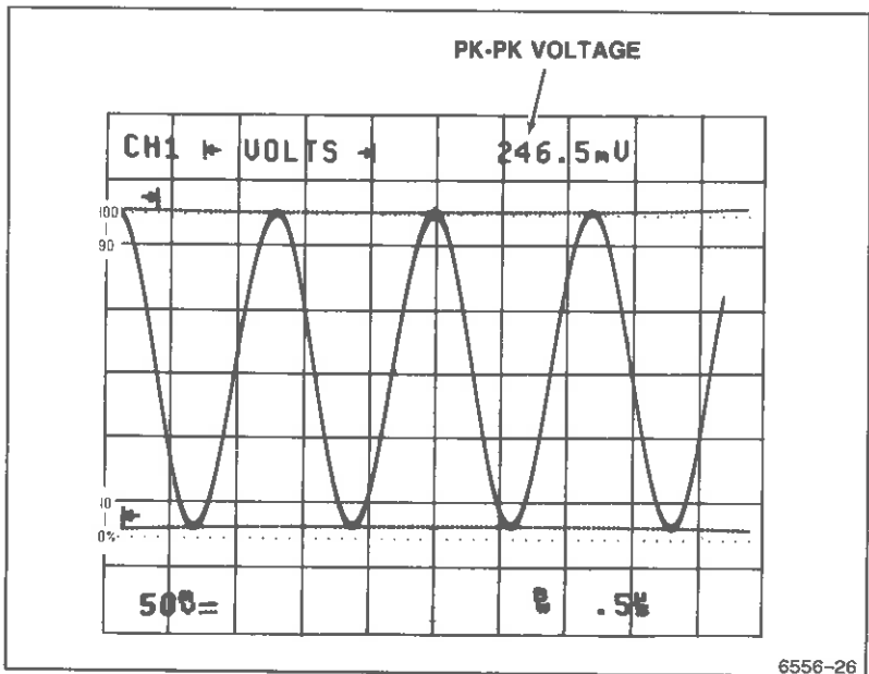
Figure 5-3. Voltage difference measurement using cursors.
