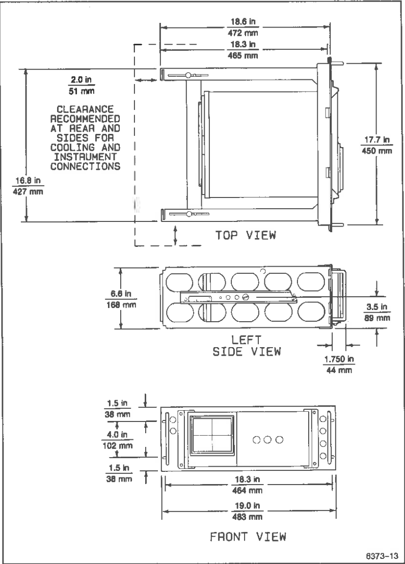
Figure 6-3. Dimensional drawing, rackmount cabinet (2240F1R).
