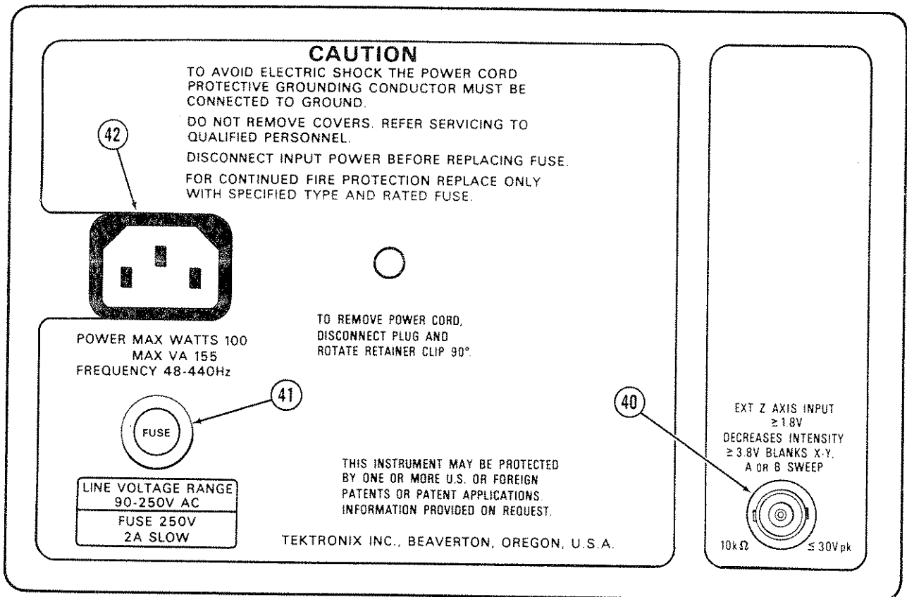
Figure 3-6. Rear Panel Connectors and Fuse.
