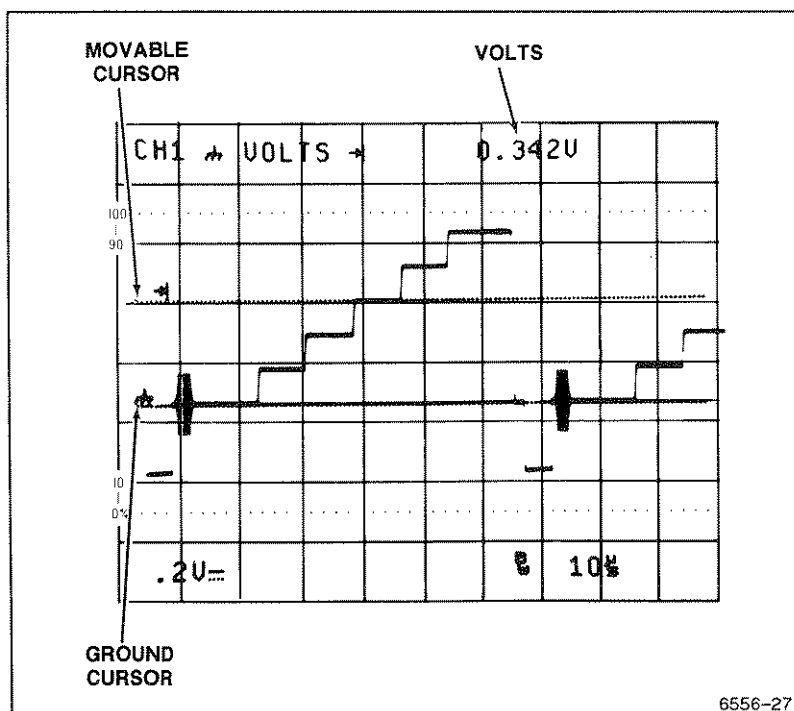
Figure 5-4. Voltage measurement.
