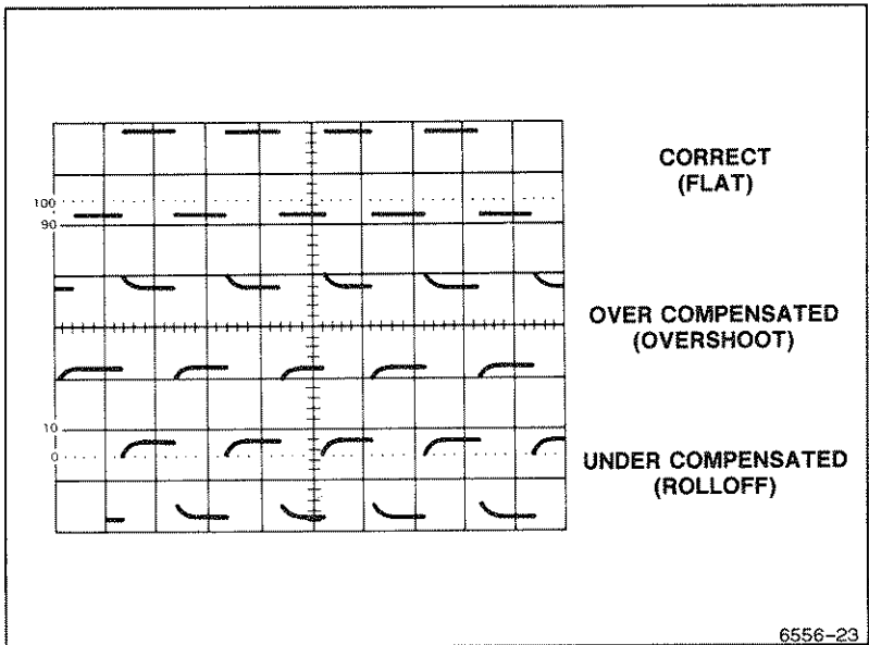
Figure 4-1. Probe compensation.
