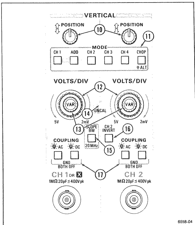
Figure 2-2. CH 1 and CH 2 vertical controls and indicators.
