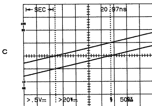
Figure 5-5. Phase difference measurement.
