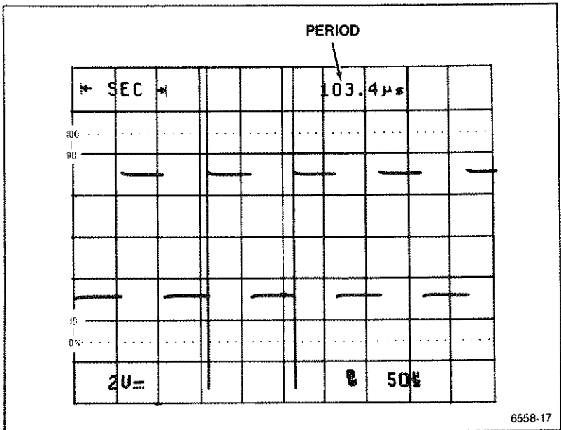
Figure 5-2. Period measurement.
