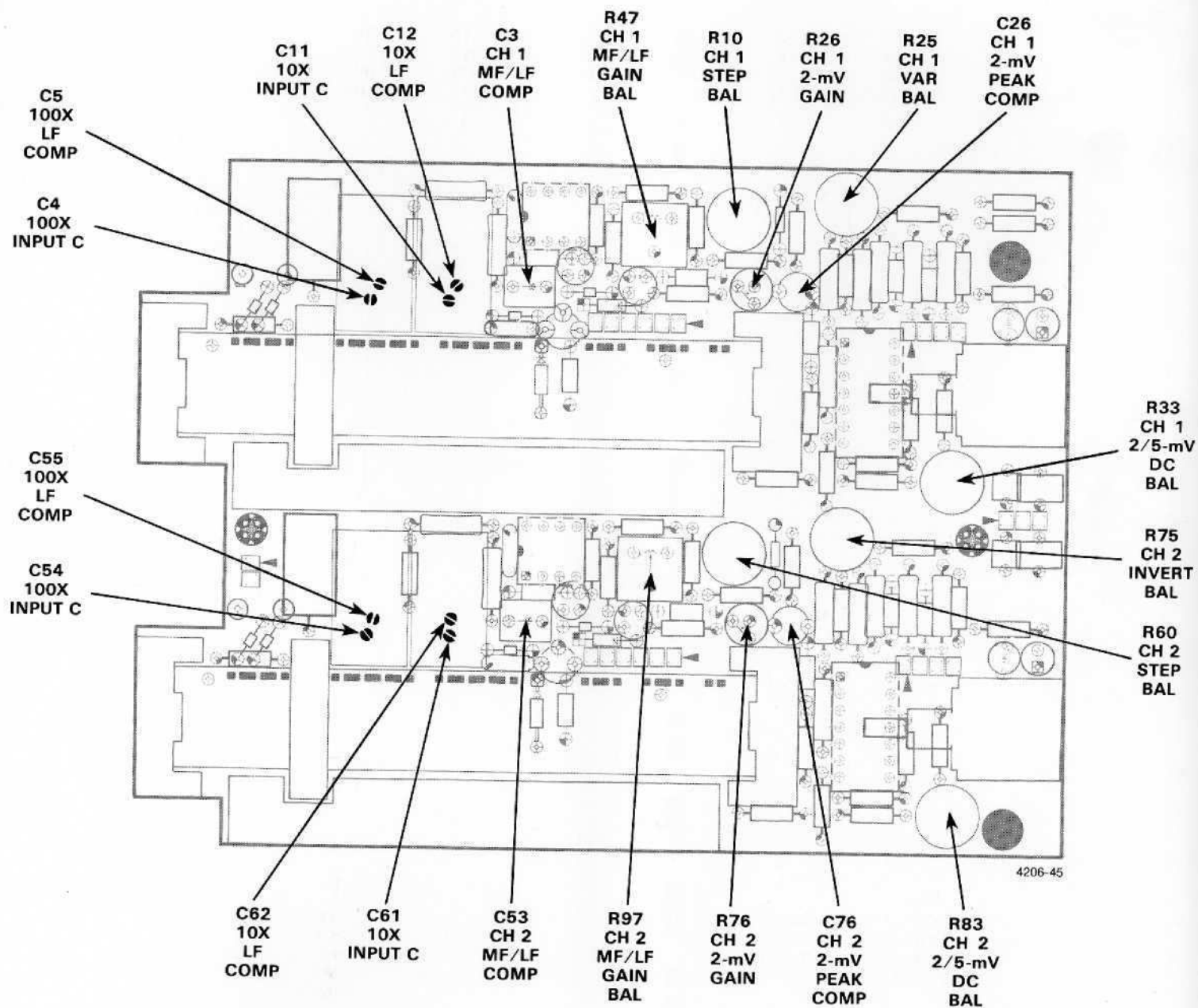
A2—ATTENUATOR BOARD ADJUSTMENT LOCATIONS
