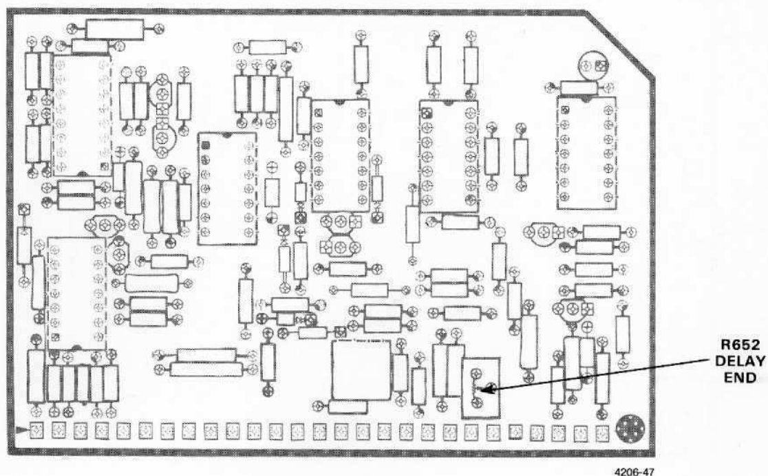
A5—ALT SWEEP LOGIC BOARD ADJUSTMENT LOCATIONS
