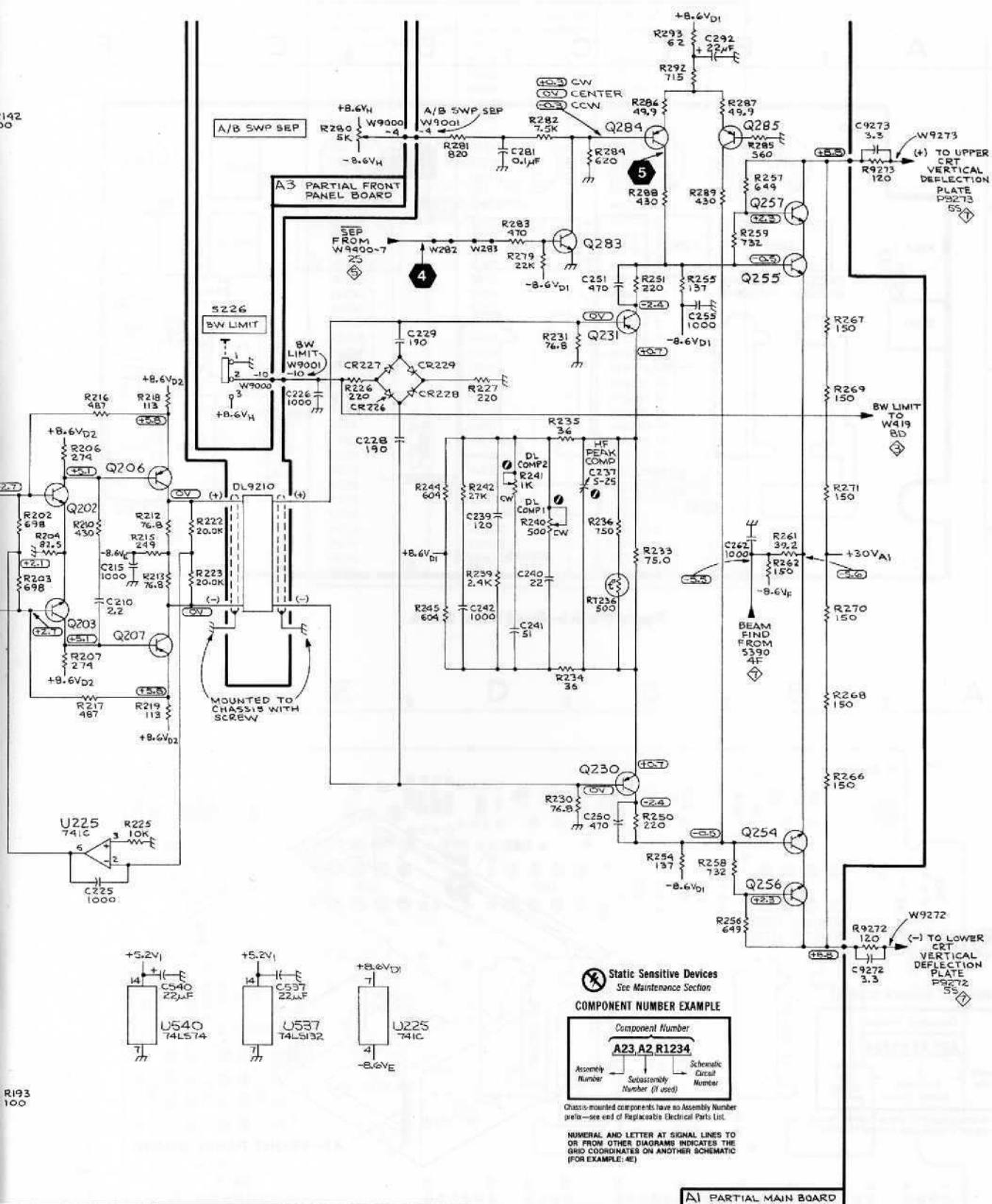
VERTICAL PREAMP &amp; OUTPUT AMPL 2
