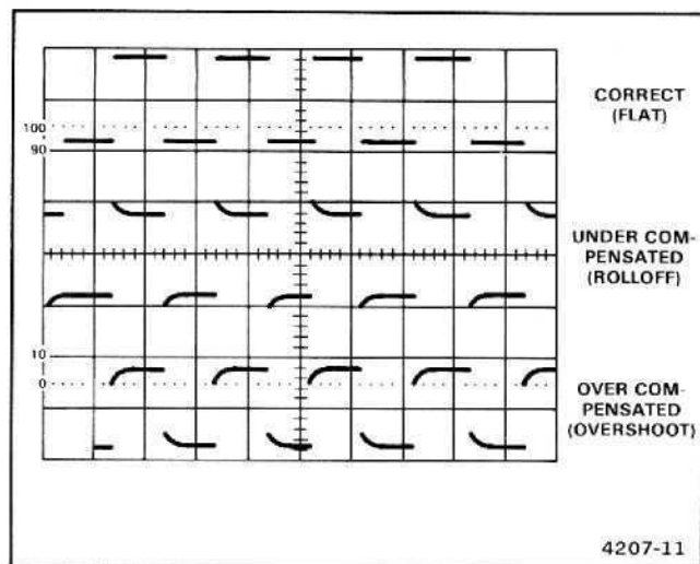
Figure 2-9. Probe compensation.
