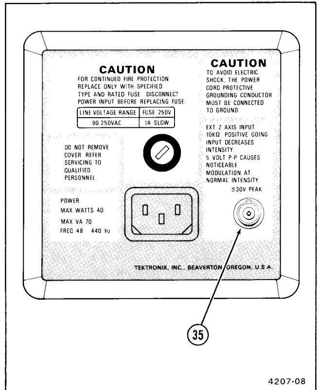
Figure 2-7. Rear-panel connector.
