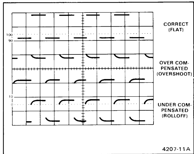
Figure 3-2. Probe compensation.
