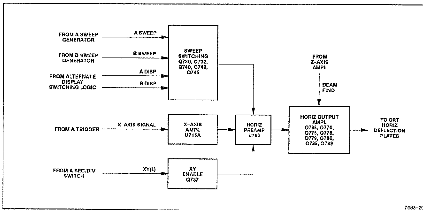
Figure 3-4. Block diagram of the Horizontal Amplifier.
