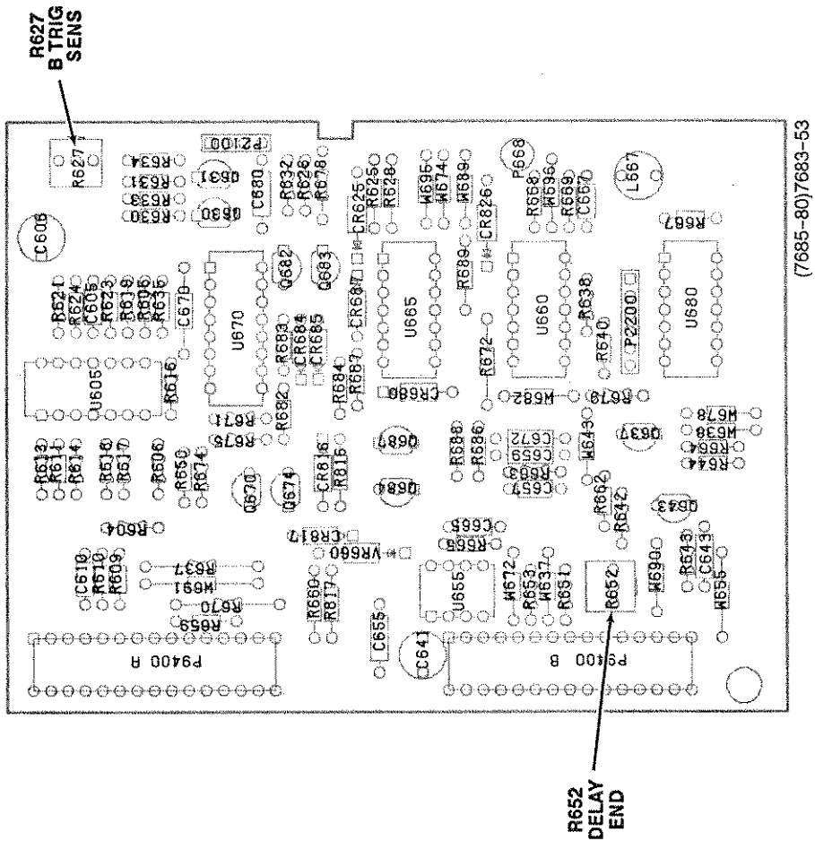
Figure 9-18. A5—Alternate Sweep board adjustment locations.
