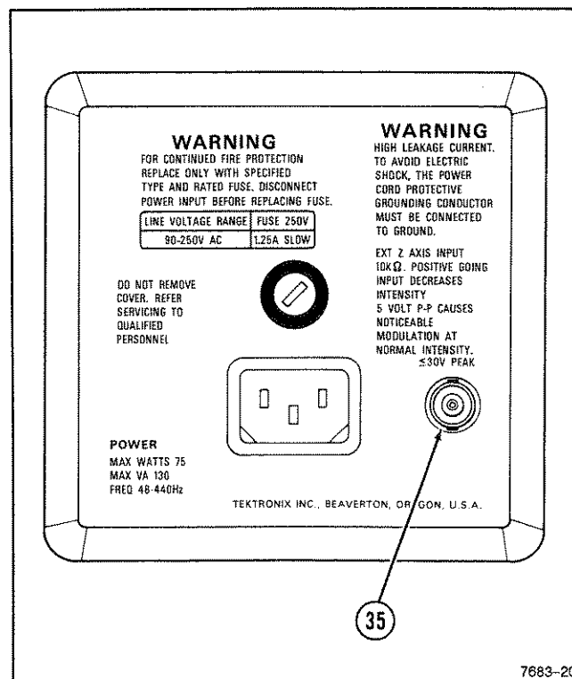
Figure 2-7. Rear-panel connector.
