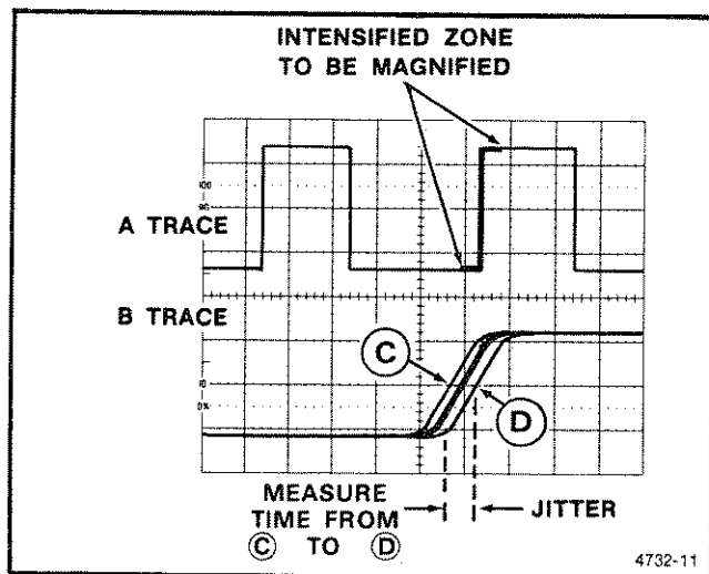
Figure 2-20. Pulse jitter.
