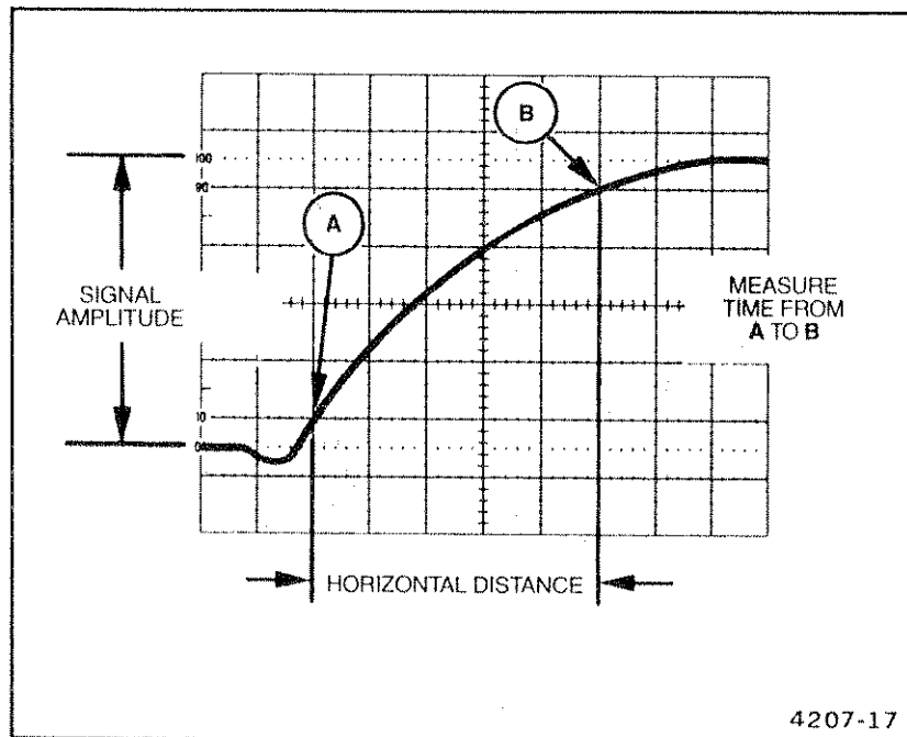
Figure 3-6. Measuring rise time.
