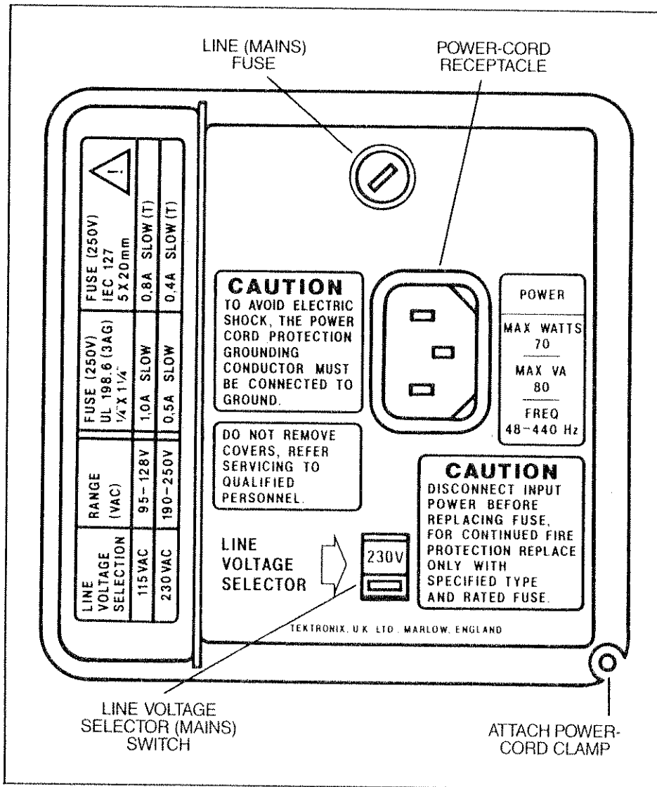
Figure 1-1. Voltage selector switch, fuse, and power-cord receptacle.
