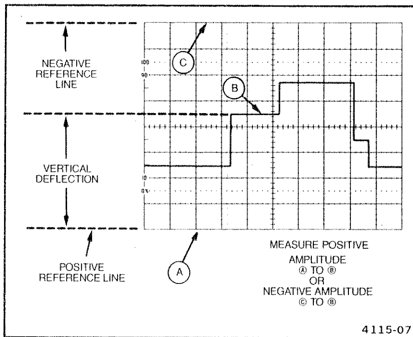
Figure 3-2. Instantaneous voltage measurement.
