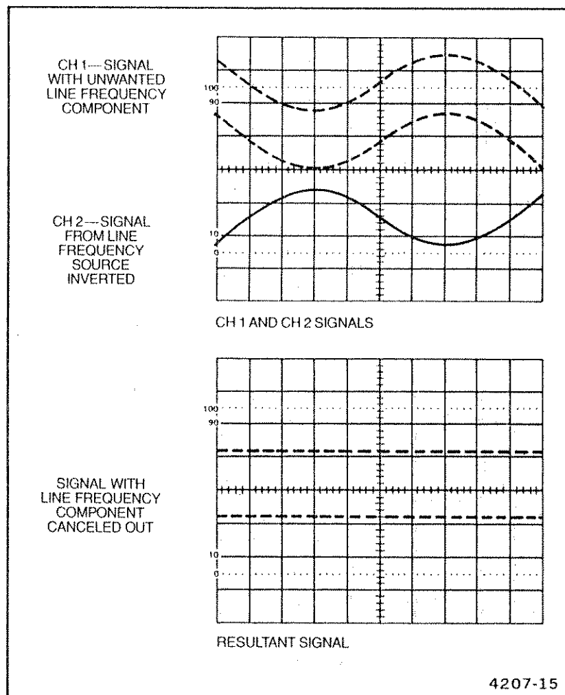
Figure 3-3. Common-mode rejection.
