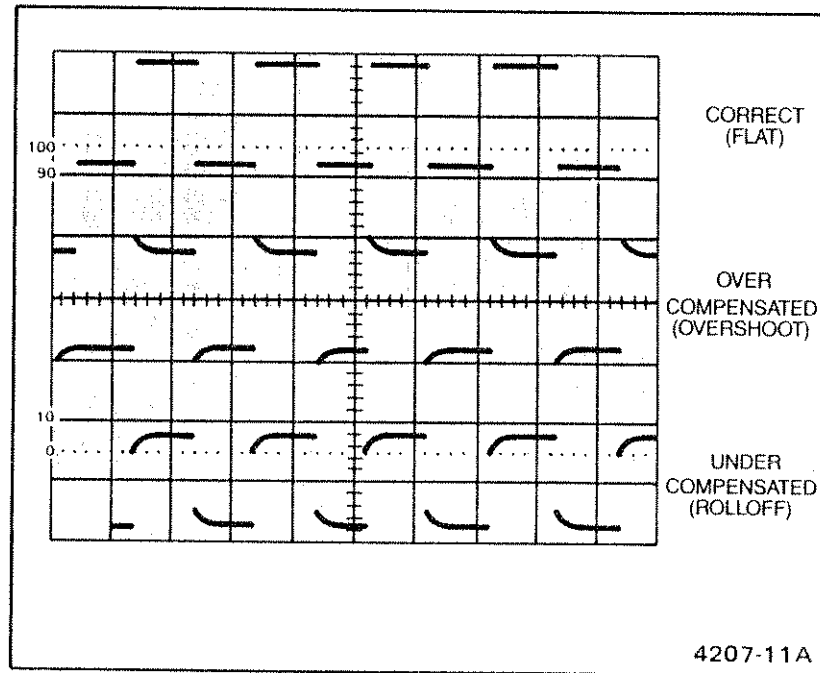
Figure 4-1. Probe compensation.
