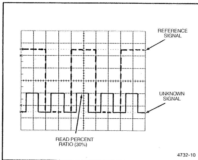
Figure 3-4. Determining voltage ratio.
