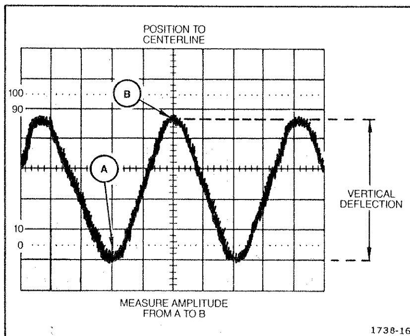
Figure 3-1. Measuring peak-to-peak voltage of a waveform.
