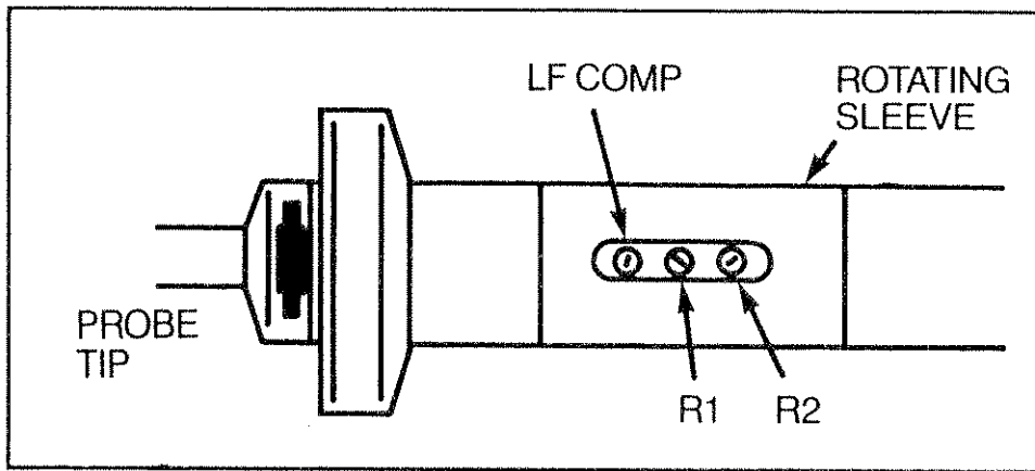
Figure 4-2. Locating the low-frequency compensation adjustment.
