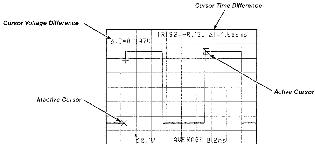
Figure 3-30: Cursor Measurements
