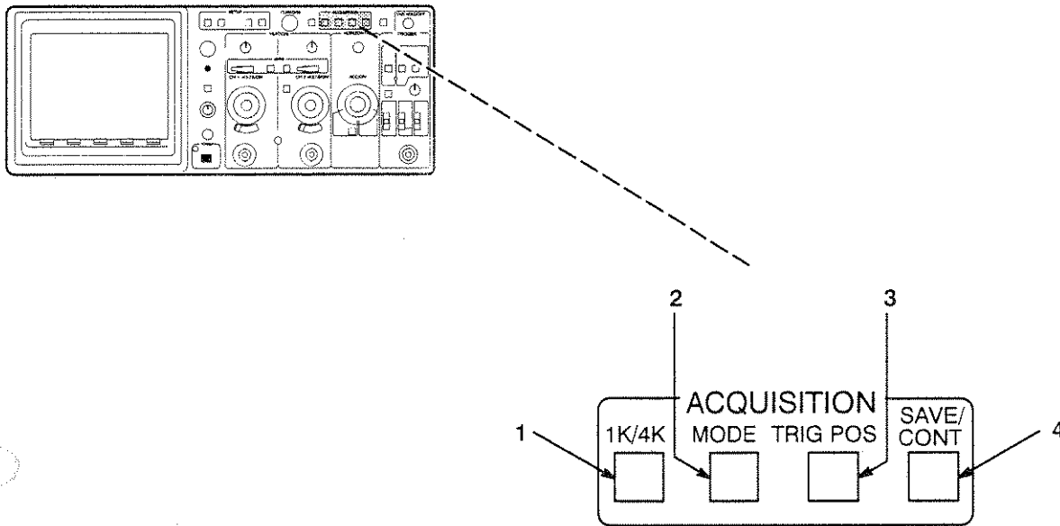
Figure 2-15: Acquisition Controls
