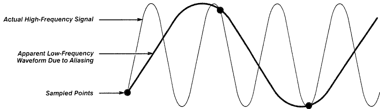
Figure 3-18: Aliasing
