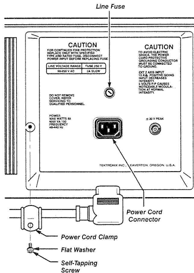
Figure 1-1: Installing the Power Cord
