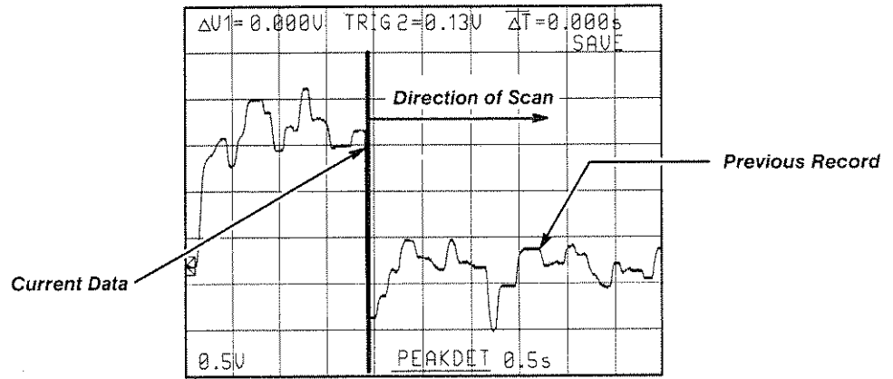
Figure 3-6: Scan Mode
