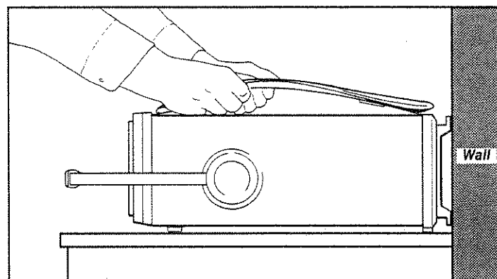
C. Bow the Plate and Slide it into the Front Trim Gap.
