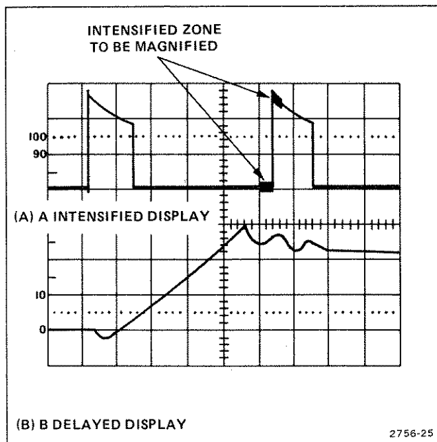
Figure 20. Delayed-sweep magnification.
