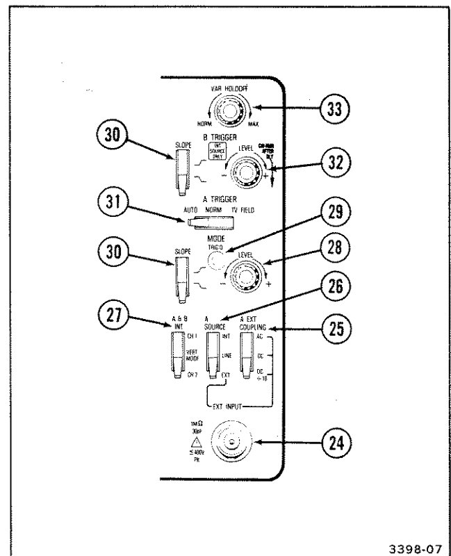
Figure 6. Trigger controls, connector, and indicator.
