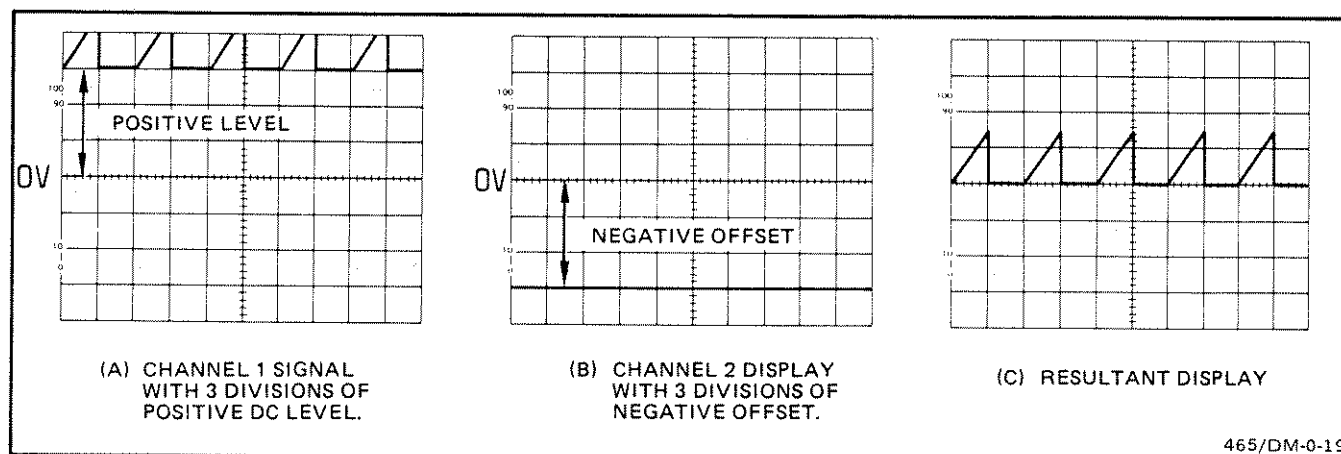
Figure 13. Algebraic addition.
