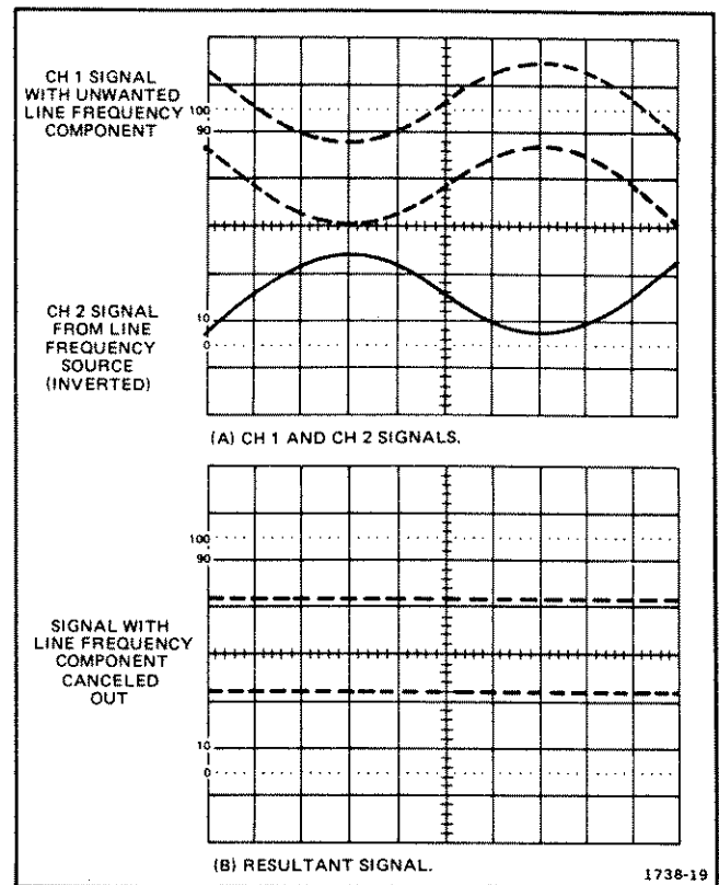
Figure 14. Common-mode rejection.
