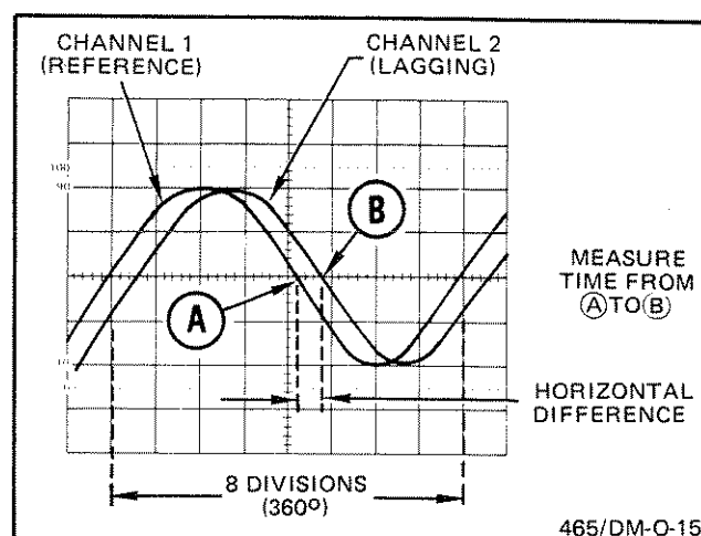
Figure 18. Phase difference.
