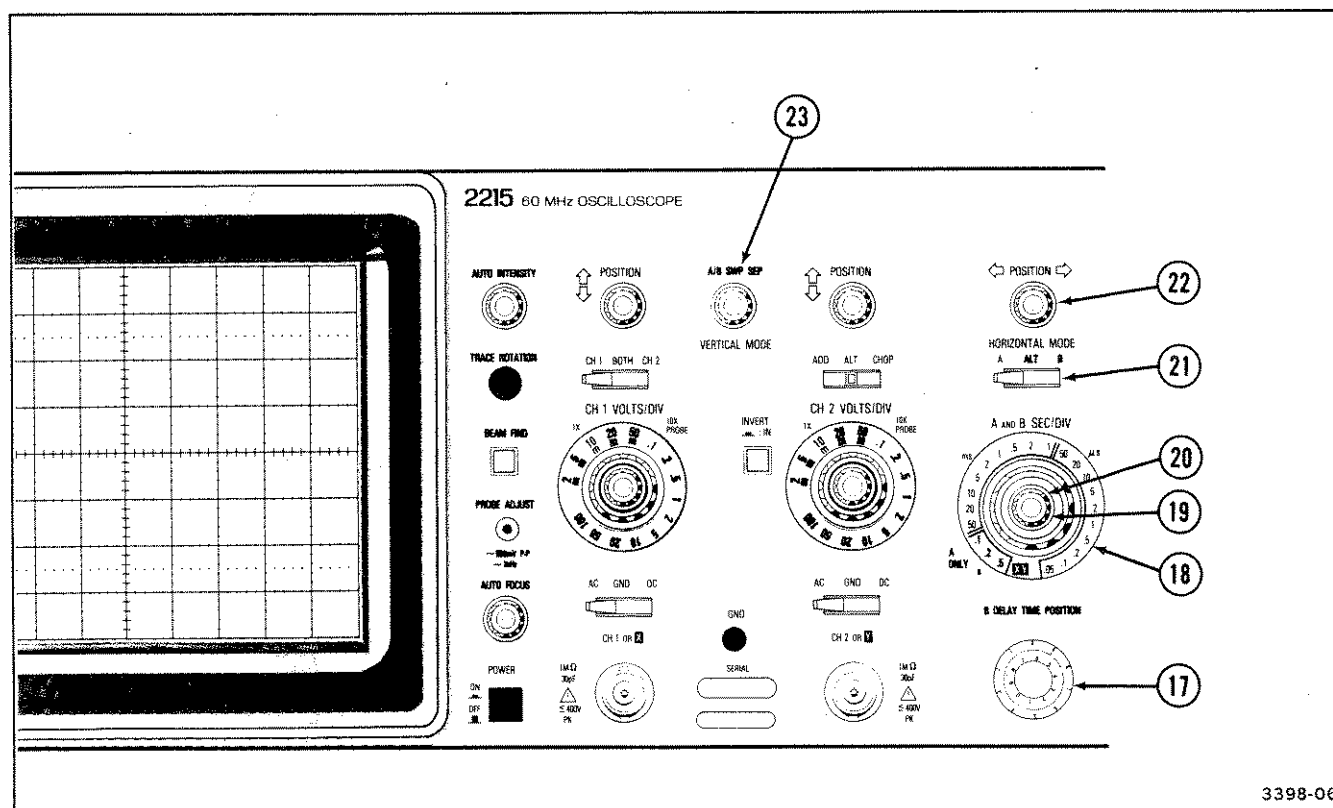
Figure 5. Horizontal controls.
