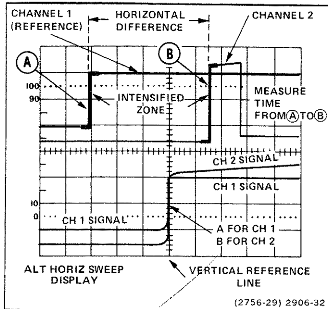
Figure 25. Time difference between two time-related pulses, differential time method.
