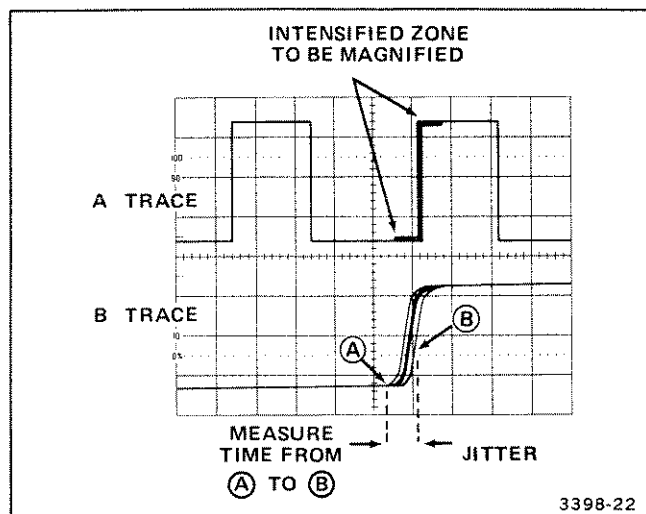
Figure 21. Pulse jitter.
