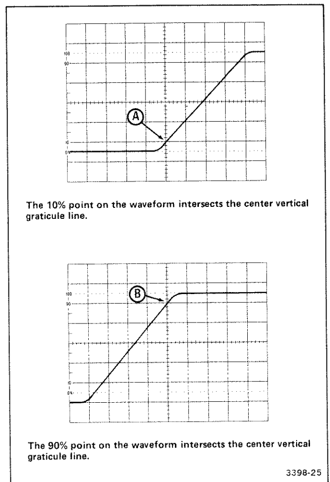
Figure 24. Rise time, differential time method.
