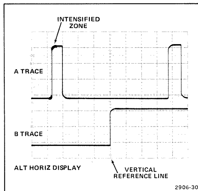
Figure 22. Time difference between repetitive pulses.
