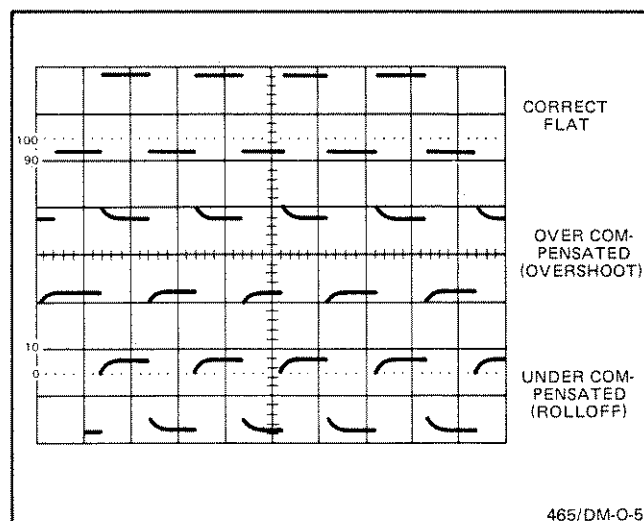
Figure 10. Probe compensation.
