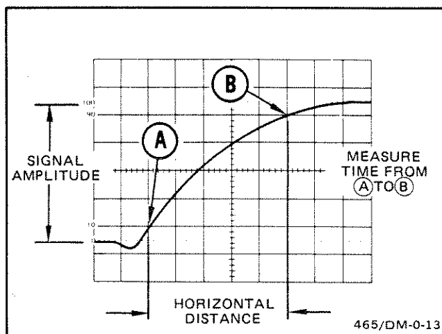
Figure 16. Rise time.
