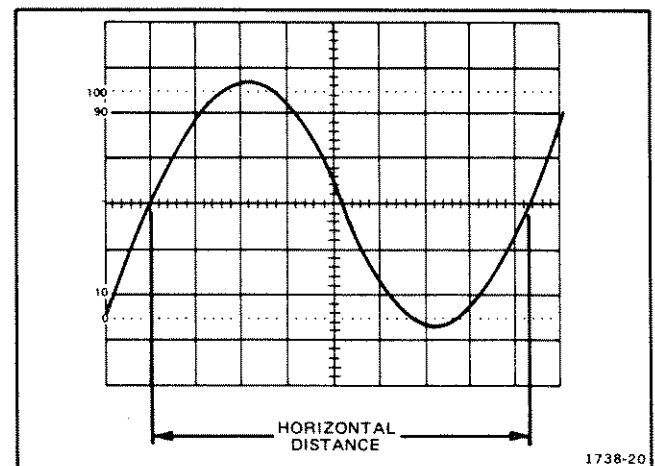
Figure 15. Time duration.
