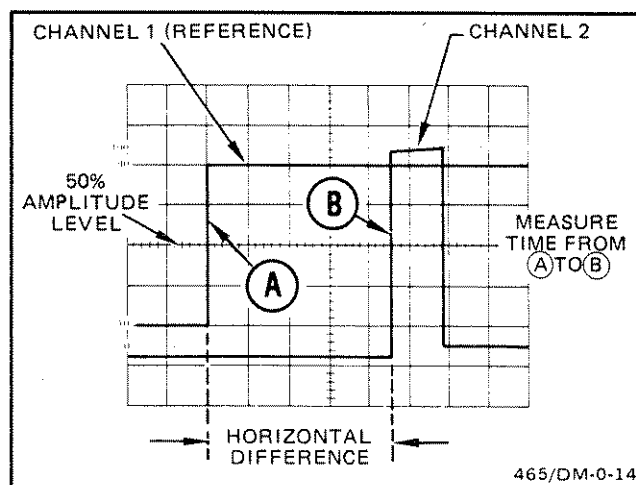
Figure 17. Time difference between two time-related pulses.
