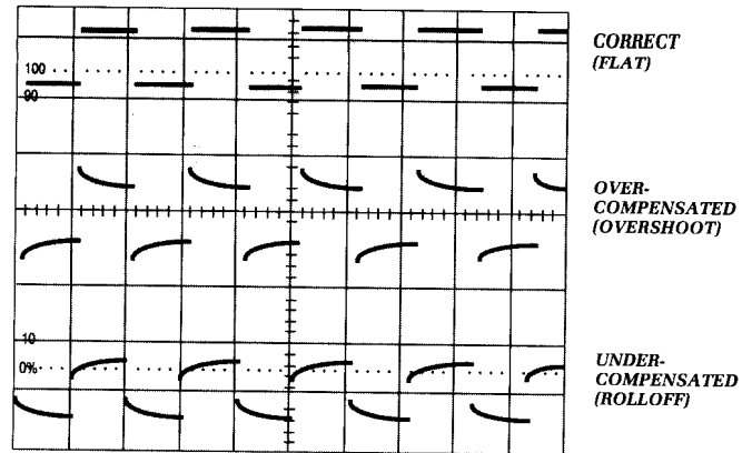
Figure 2-1: Probe Compensation
