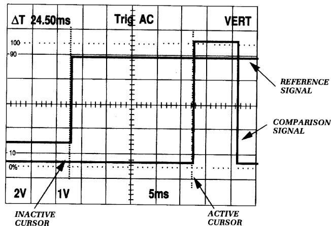
Figure 3-7: Time Difference Measurement between two Time-related Pulses
