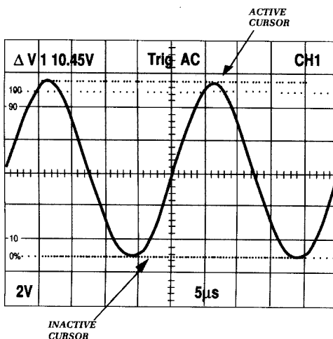
Figure 3-1: Peak-to-Peak Voltage Waveform Measurement
