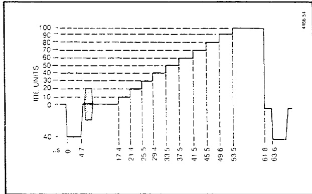
Fig. 6-29. 10-Step Staircase.
