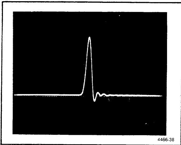
Fig. 6-13. 2T Pulse Exhibiting Gain/Frequency and/or Group-Delay Distortion.
