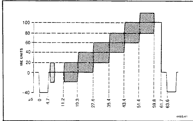
Fig. 6-16. Modulated 5-Step.
