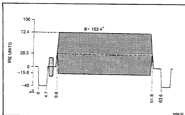
Fig. 6-25. Red Field.
