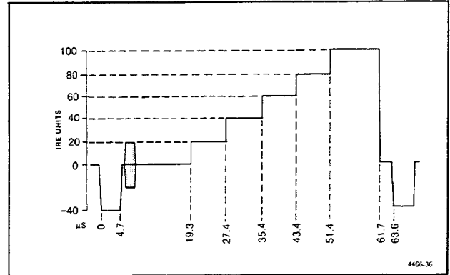
Fig. 6-11. 5-Step Staircase.
