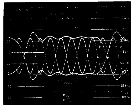
F. 8 high-bit/8 low-bit portion of pattern, interleaved with reference and band limited to 4 MHz.
