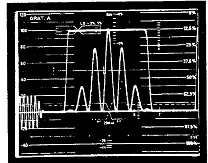
Figure 2 (a) 1.0 MHz
