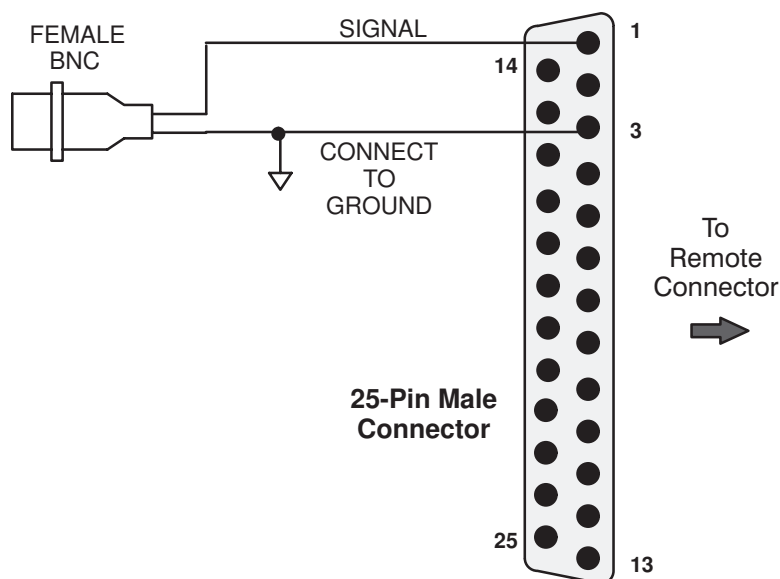
Figure 5-1: External Horizontal/RGB and YRGB Cable Adapter
