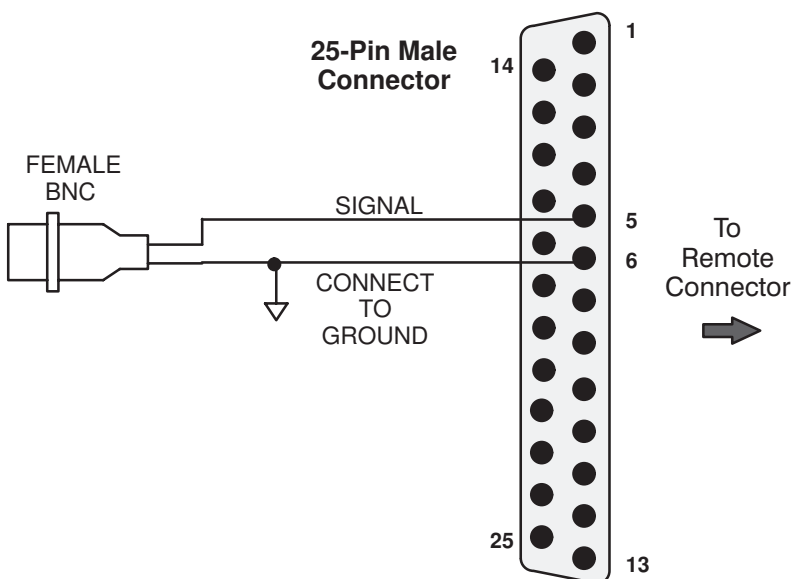
Figure 4–2: Remote Sync Cable Adapter
