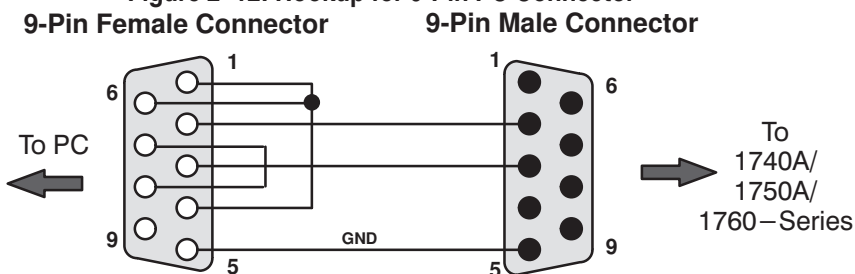
Figure 2-12: Hookup for 9-Pin PC Connector
