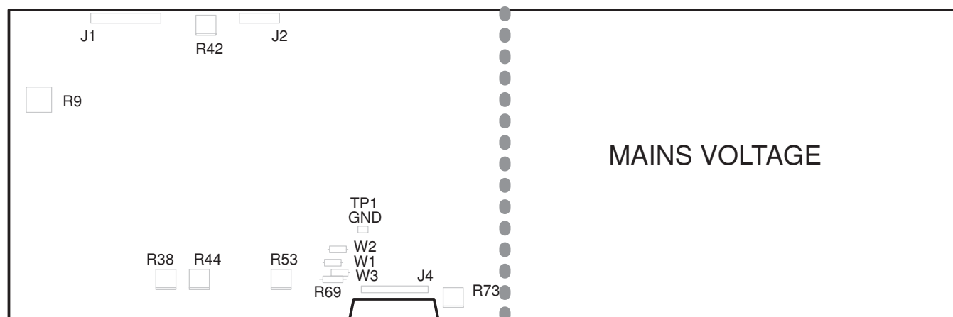
Figure 5–7: A1 Power Supply Board
