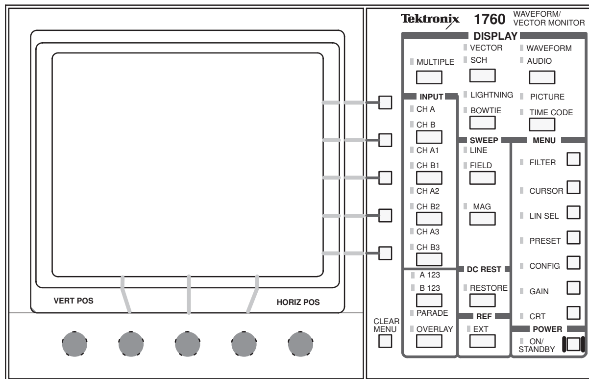
Figure 2–16: 1760 front panel
