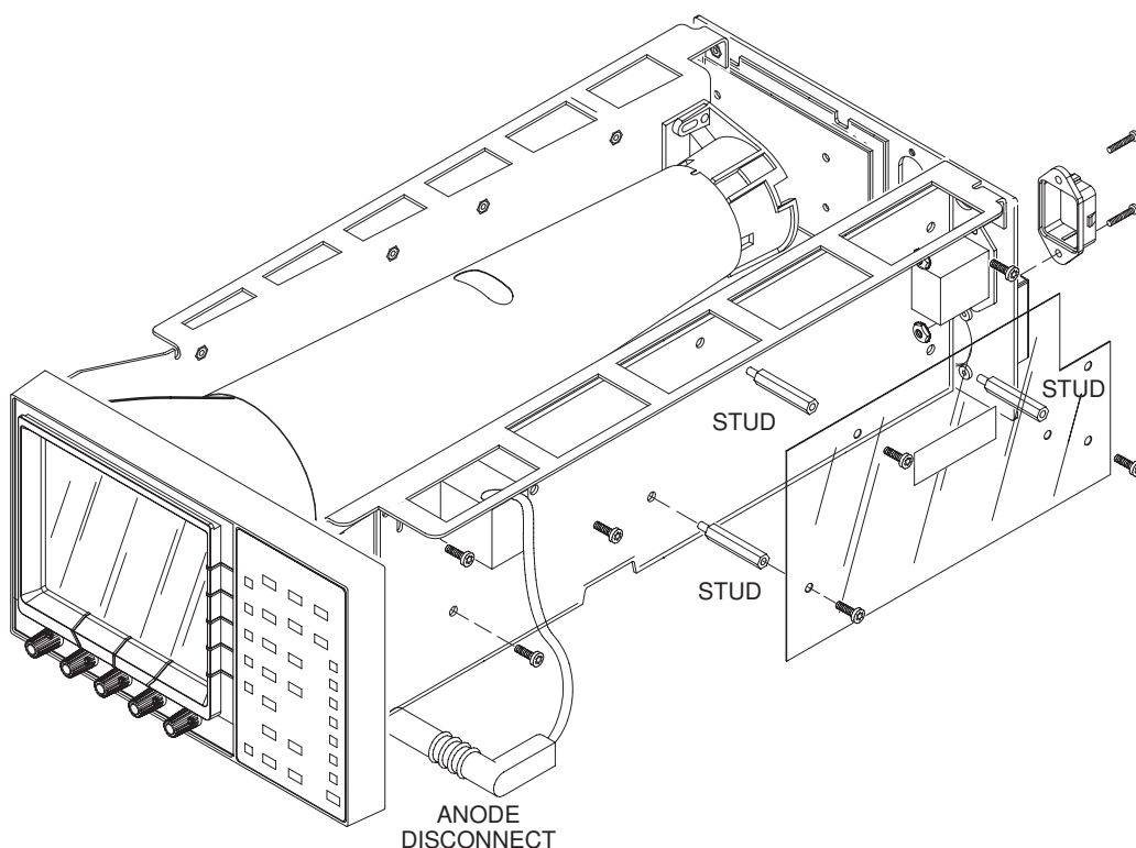
Figure 6-11: Securing screws for the Power Supply circuit
