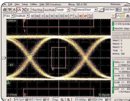
► OI1125 eye diagram at 12.5 Gb/s with scaled OC-192 mask.
