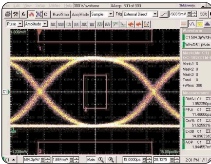
► OI1125 eye diagram at 9.953 Gb/s with OC-192 mask.
