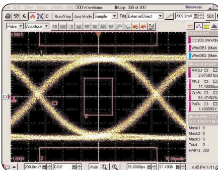
► OI2125 eye diagram at 9.953 Gb/s with an OC-192 mask.
