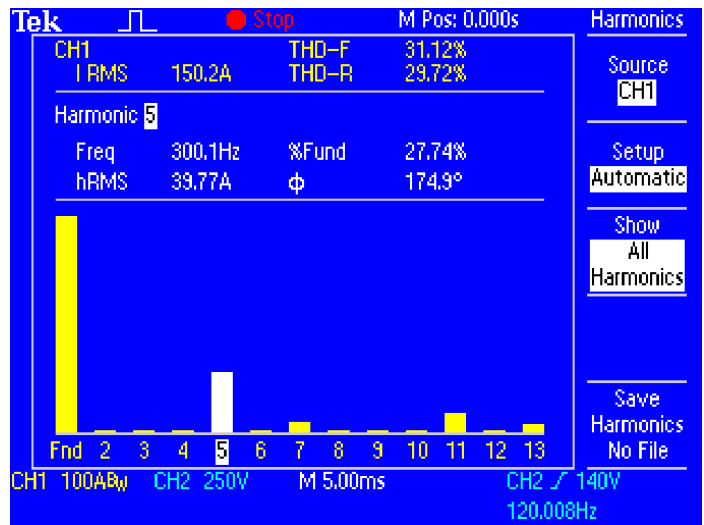
Conduct harmonic distortion measurements with TPS2PWR1 software.
