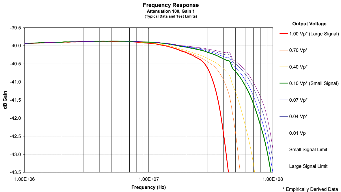
Graph 1.1 – 4040B Frequency Response, Attenuation 100, Gain 1
