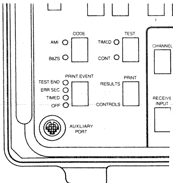
Figure 2-14 AUXILIARY Port Connector
