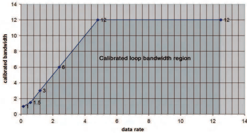
CRU loop bandwidth vs data rate
