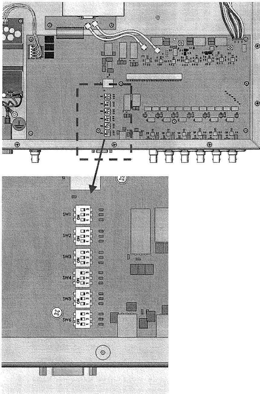
Figures 4 & 5: Dipswitch Locations for Configuring Outputs
