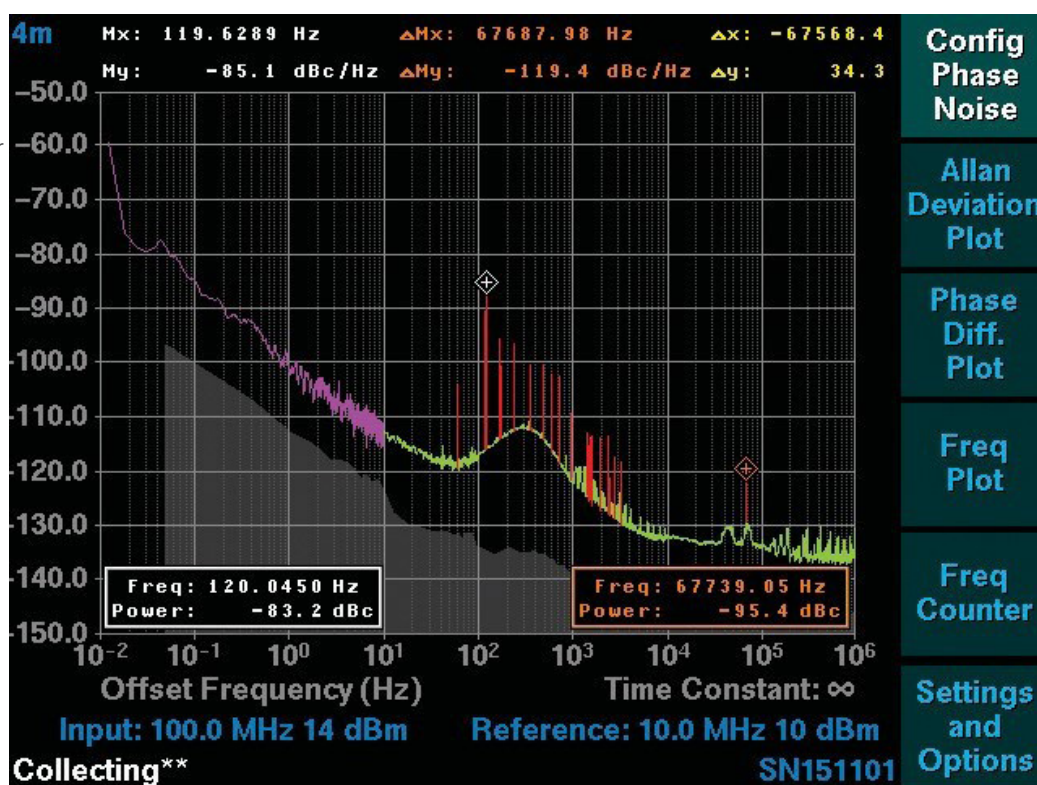
5125A Sample Display Capture—Phase Noise
