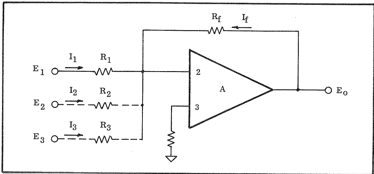
Figure 3. Summing amplifier
