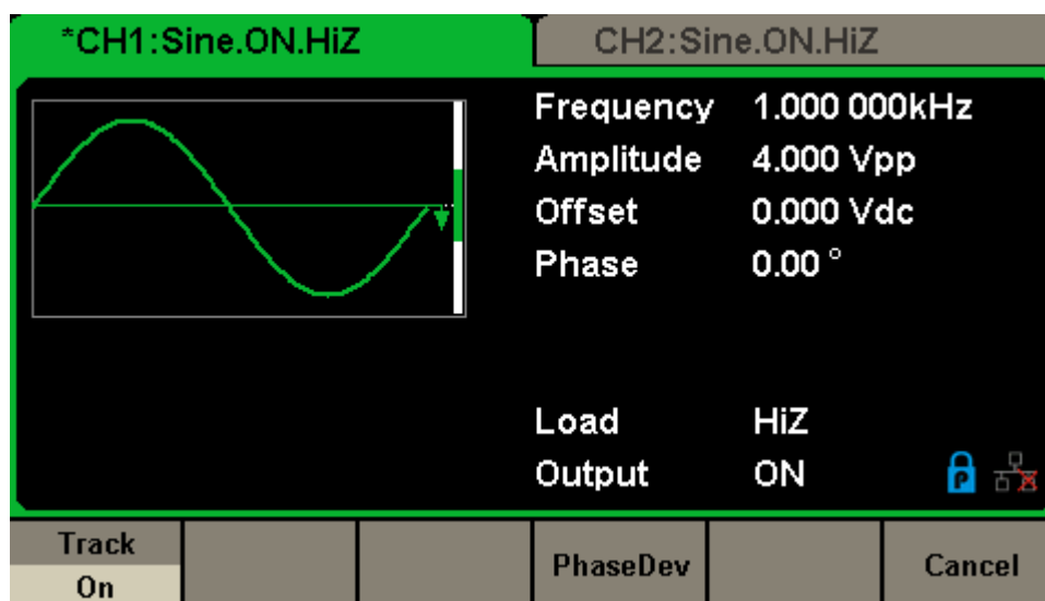
Figure 2-70 Track Interface
