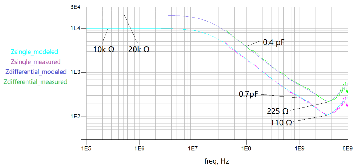
SAP5000D Input Impedance (Soldered 24.9 \Omega Lead Resistance)
