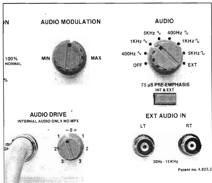
Figure 14: Select the type of audio signal to be used with the AUDIO control and set the level to match the circuit under test.
