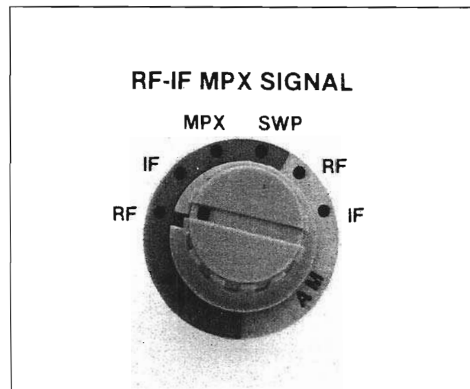
Figure 10: Use the FM RF, IF, MPX, And SWP signal for testing and troubleshooting an FM tuners and receivers.
