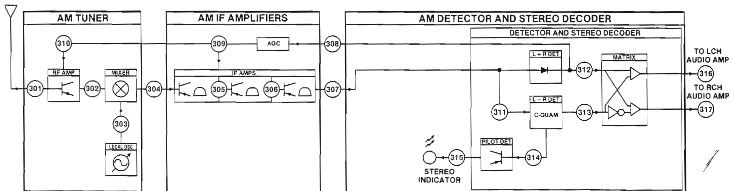
AM Block
