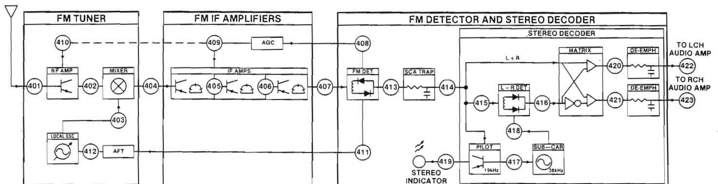
FM Block
