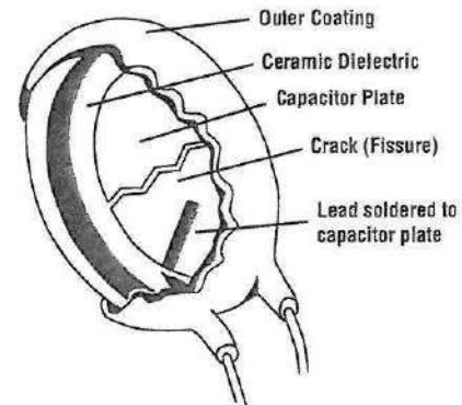
Fig. 43: A ceramic disc is made of a silver coated ceramic dielectric which is coated with a protective coating. Large cracks or fissures in the dielectric may develop which change the capacitance value.
