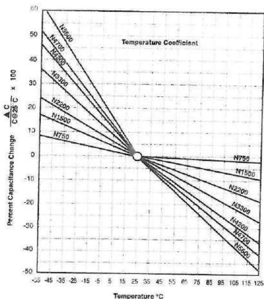
Fig. 40: Temperature change versus capacity change of N750 to N5600 temperature compensated ceramic disc capacitors.
